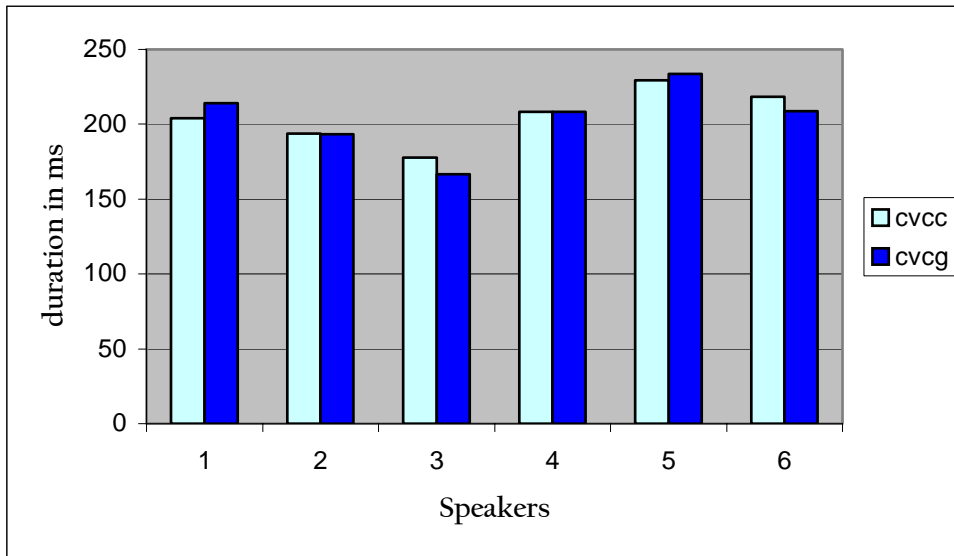
Figure 9: Mean durations in CVCC and CVCG words
