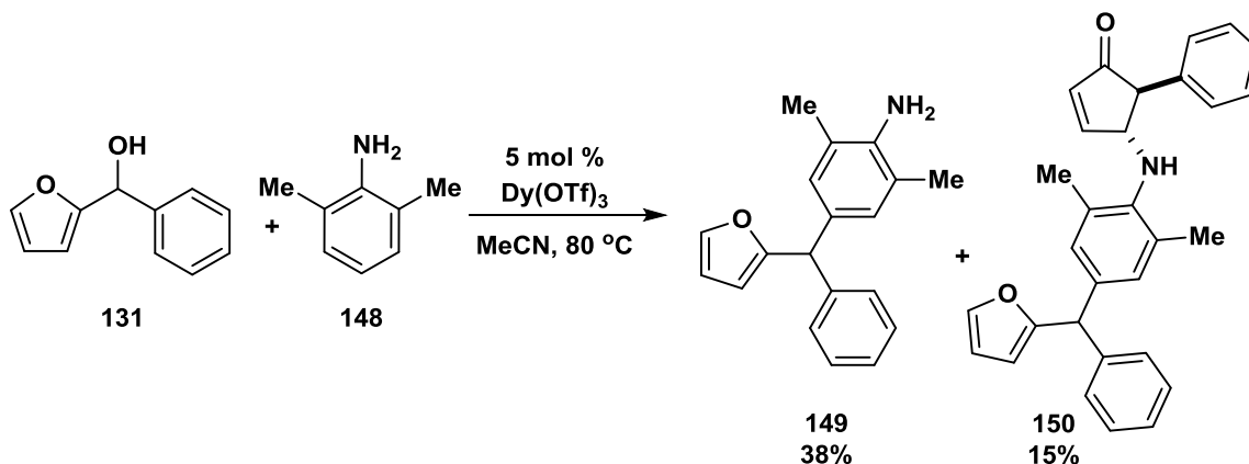
Scheme 17. Products resulting from Friedel–Crafts alkylation.
