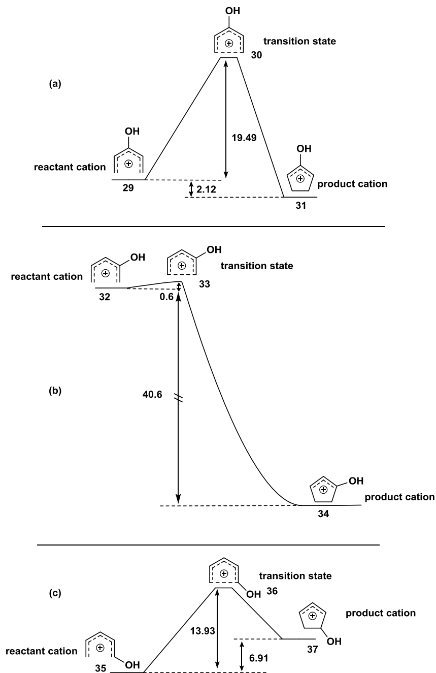
Figure 6. Reaction barriers for cyclization of hydroxy substituted pentadienyl cations. Calculated at the B3LYP/6-311G* level.
