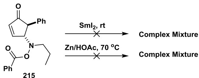
Scheme 28. Failed attempts to break the N–O bond.
