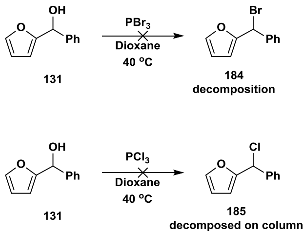
Scheme 24. Attempts to install halogen leaving groups.
