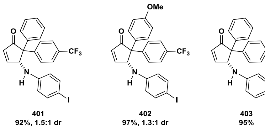
Figure 24. Bis-aryl cyclopentenones.
