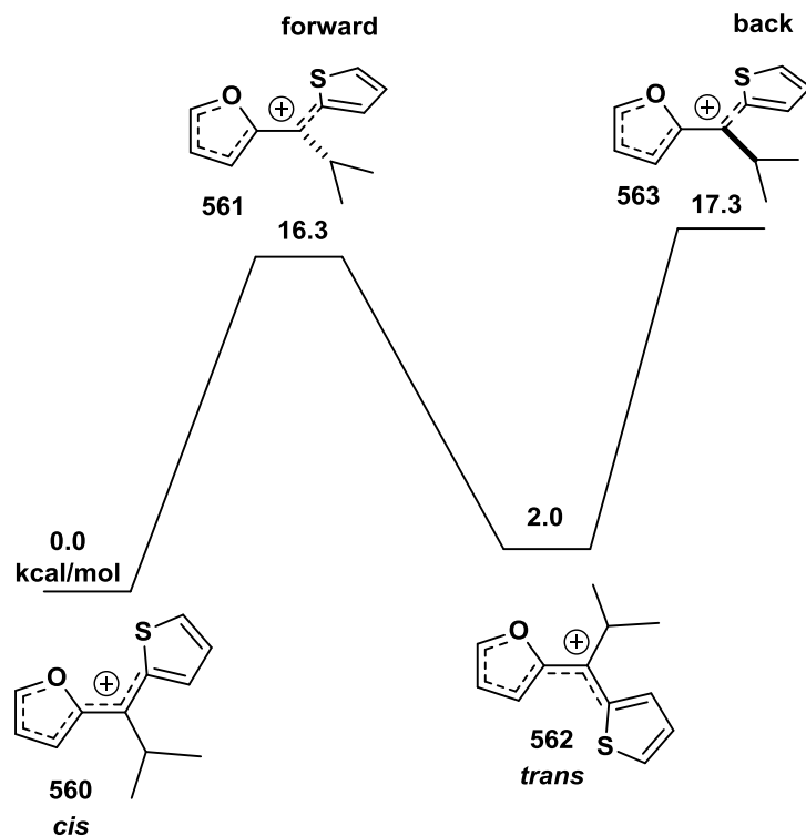
Figure 41. Isopropyl-, thiophene-substituted furyl carbocation geometries. Rotational scan calculated using B3LYP/6-31G* (d,p) with 10^\circ intervals. All values in kcal/mol.
