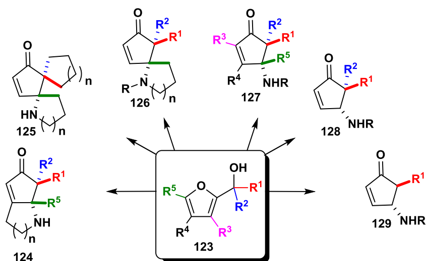
Figure 12. Possible 4-aminocyclopentenones from an aza-Piancatelli rearrangement.
