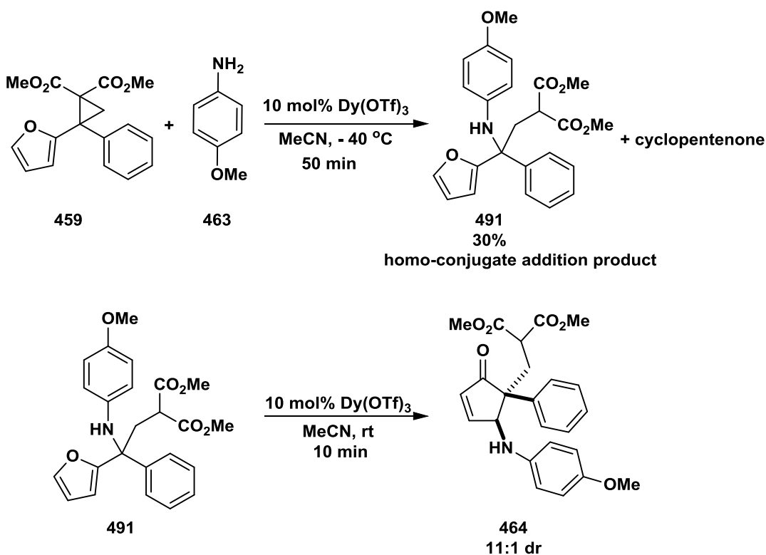
Scheme 68. Resubjection of homo-conjugate addition products.
