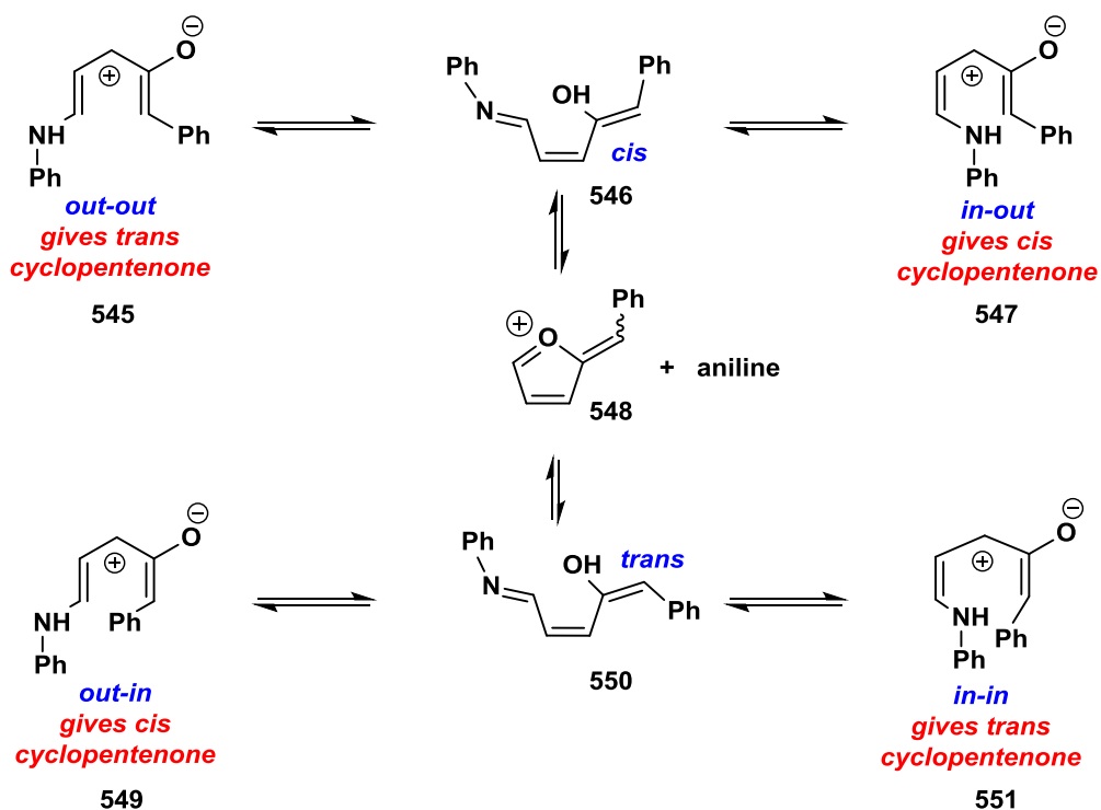
Figure 36. Possible pentadienyl cation geometries.
