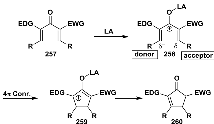
Figure 19. Polarization of the dienone.
