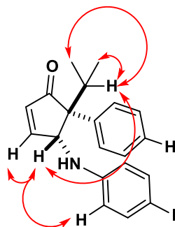
Figure 23. NOESY correlations for 381.
