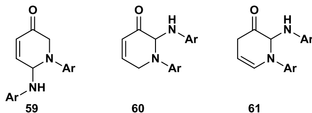
Figure 9. Structures proposed by McGowan of the free base Stenhouse compounds.
