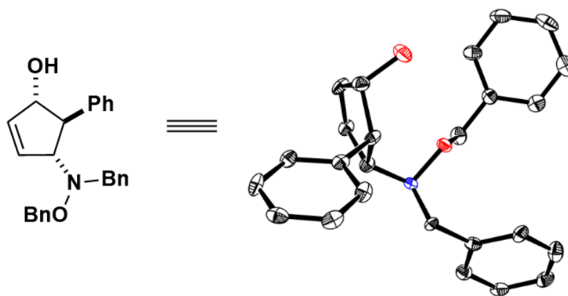
Figure 17. ORTEP drawing of 1,2- trans -2,3- trans -cyclopentenol 235 shown with 50% thermal ellipsoids. Hydrogen atoms have been omitted for clarity. The crystal structure data can be obtained from the Cambridge Crystallographic Data Centre via www.ccdc.cam.ac.uk/data_request/cif . CCDC # 986010
