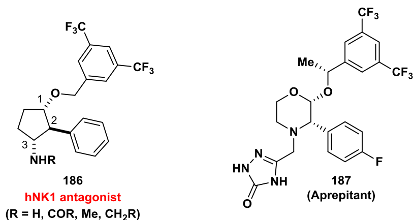
Figure 15. hNK1 Inhibitors.
