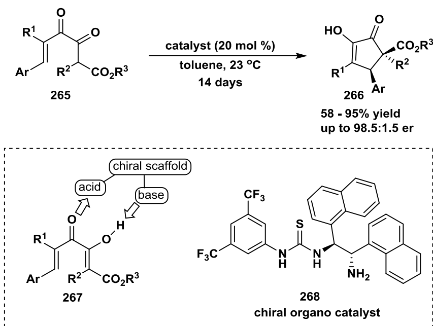
Scheme 36. Diketones for an enantioselective organocatalytic Nazarov reaction.
