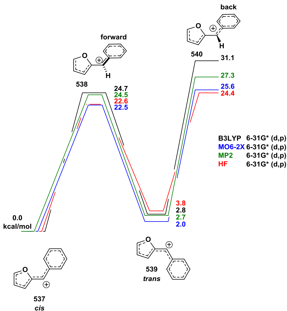
Figure 34. Comparison of computational methods. All values in kcal/mol.
