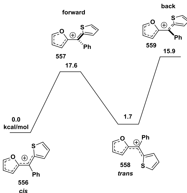
Figure 39. Phenyl-, thiophene-substituted furyl carbocation geometries. Rotational scan calculated using B3LYP/6-31G* (d,p) with 10^\circ intervals. All values in kcal/mol.
