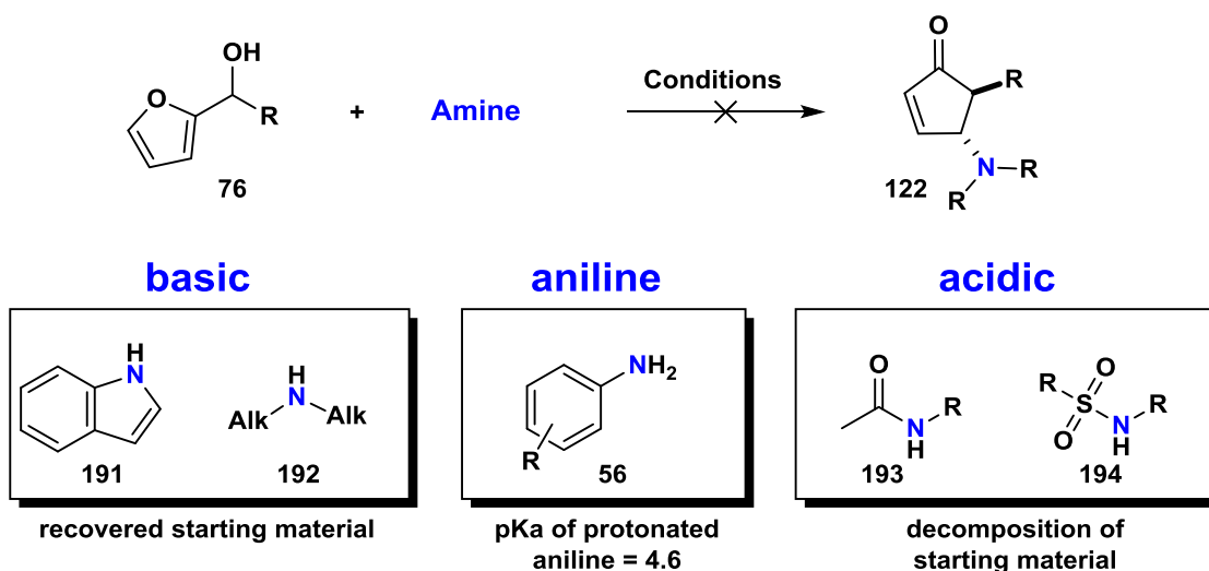
Figure 16. Attempts to utilize non-aniline amine nucleophiles.
