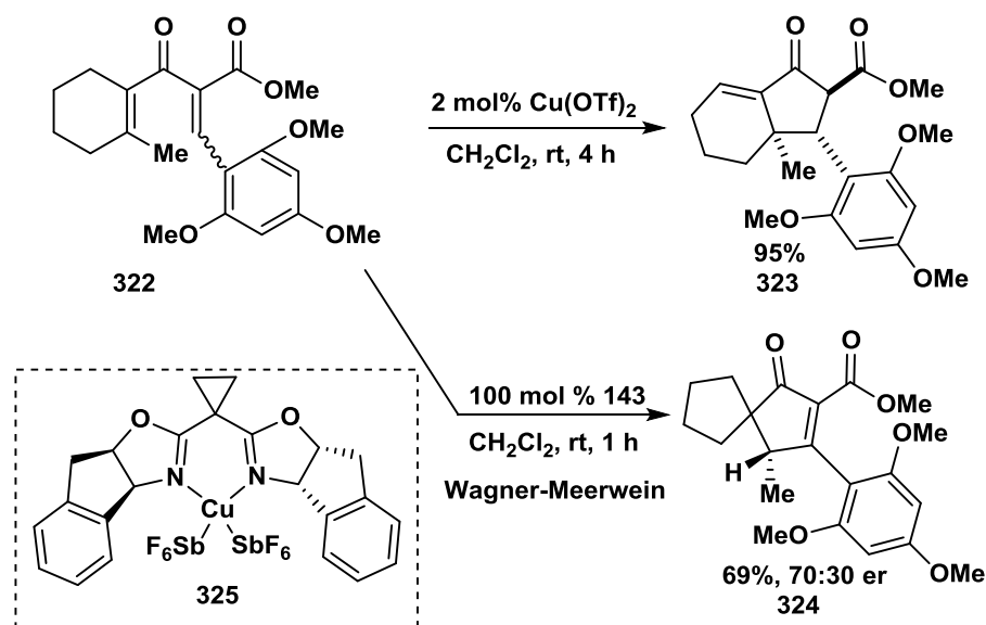
Scheme 49. Copper catalyzed Nazarov cyclization leading to different products.
