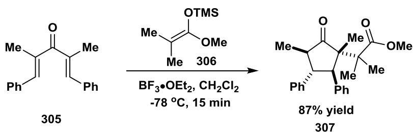
Scheme 45. Interrupting the Nazarov with silyl enol ethers.
