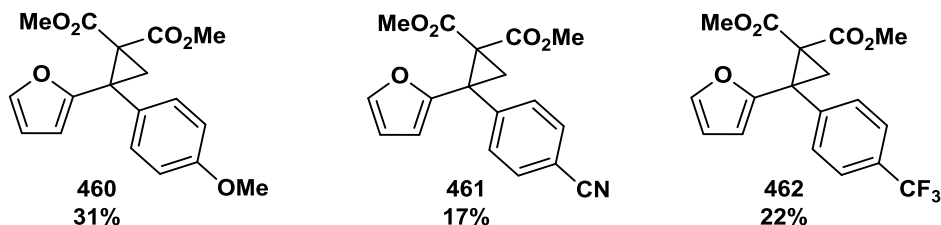
Figure 27. Cyclopropane yields from Rh(II) catalyzed cyclopropanation with phenyl iodonium ylides.
