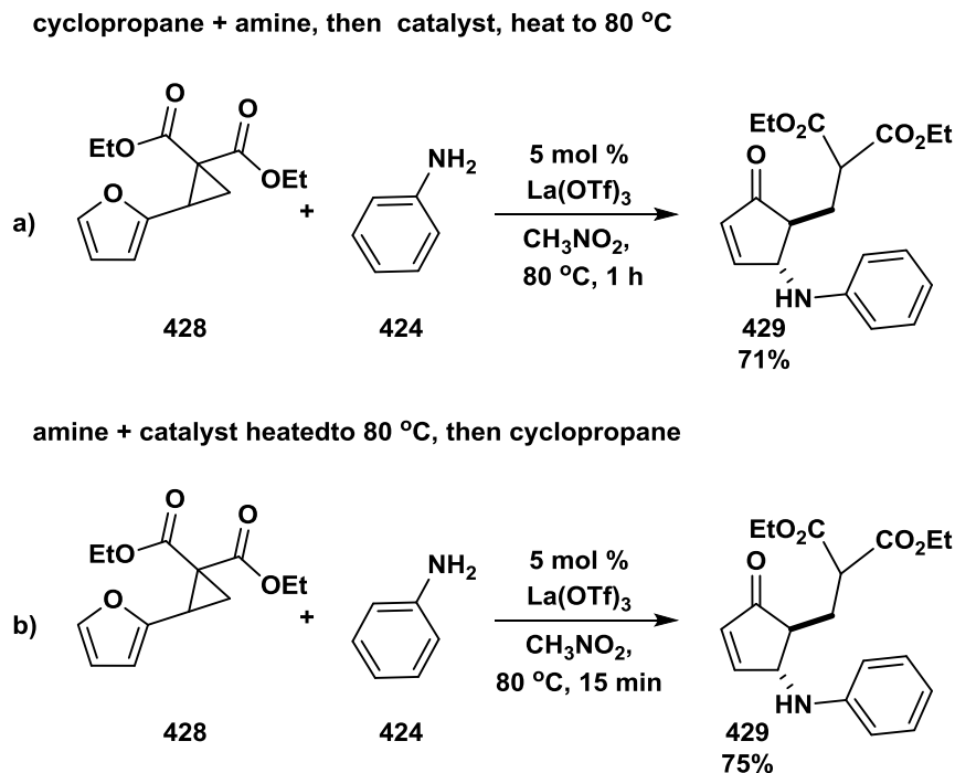
Scheme 61. The effect of changing the order of reagent addition.
