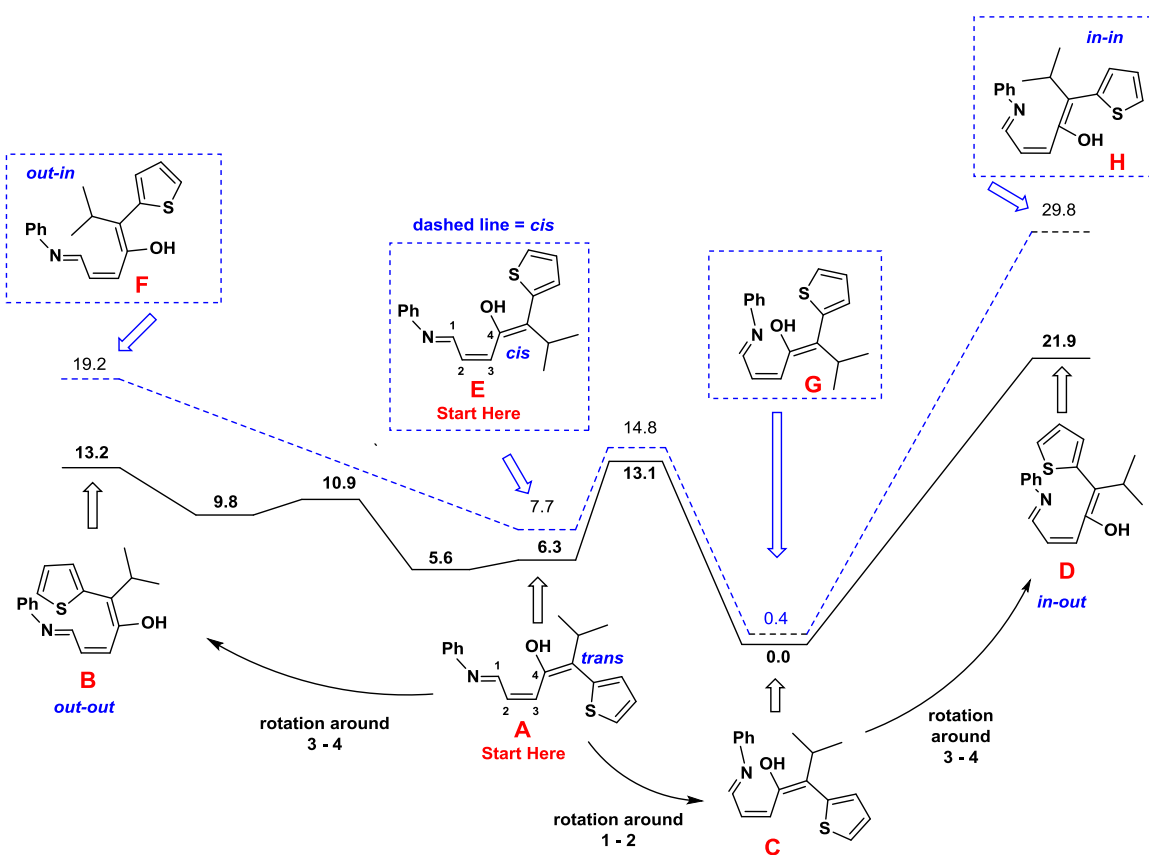
Figure 42. Energy barriers for rotation of the ring opened intermediate derived from isopropyl-, thiophene-substituted furylcarbinol. Rotational scans calculated using B3LYP/6-31G* (d,p) with 10° intervals. All values in kcal/mol.
