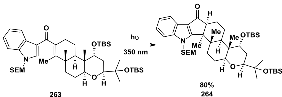
Scheme 35. Light catalyzed Nazarov for the construction of terpendole E Analogues.
