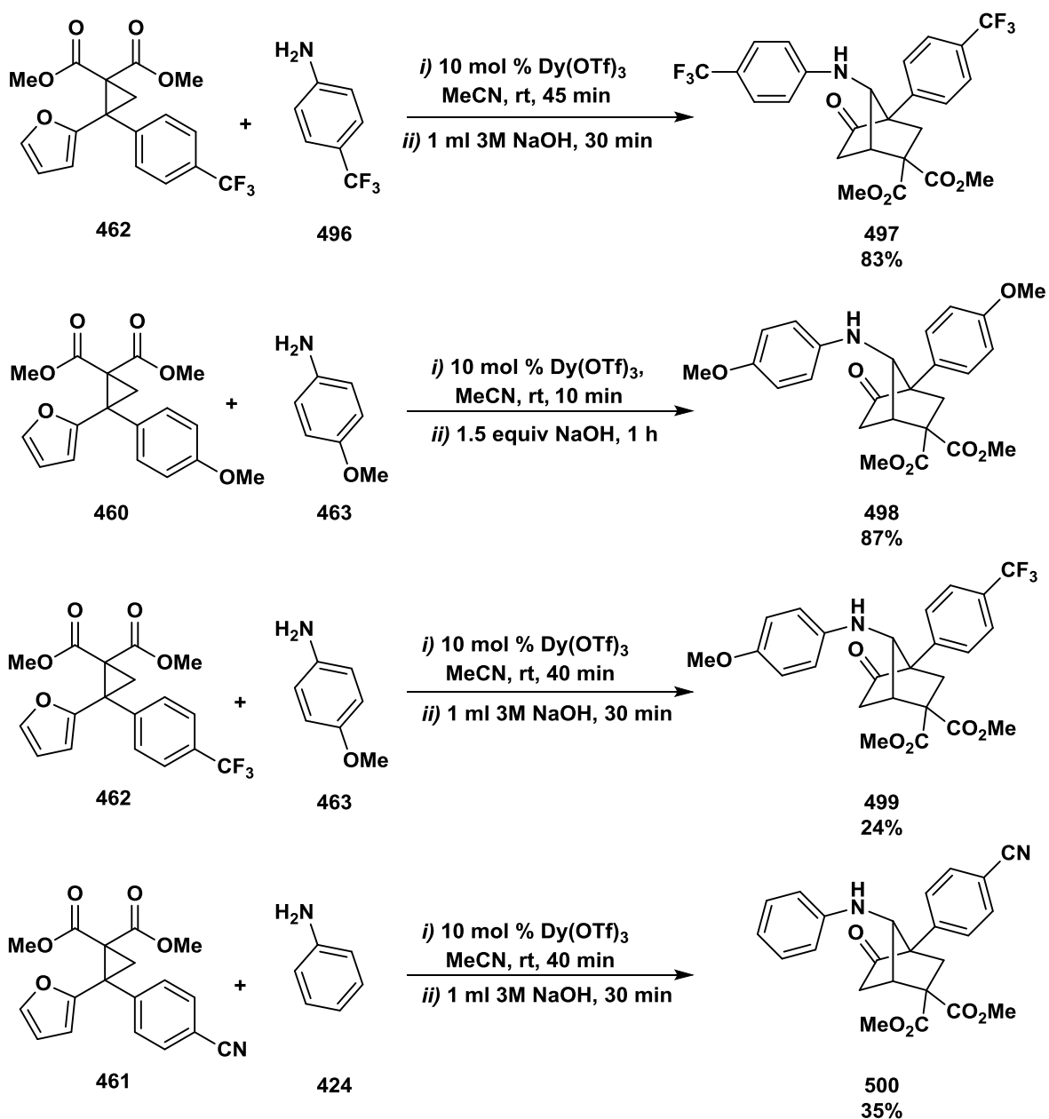
Scheme 72. NaOH induced intramolecular Michael addition.
