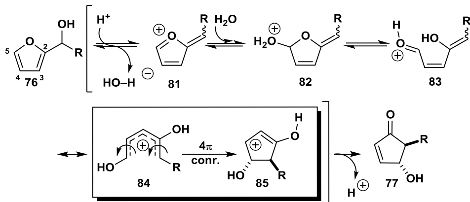
Figure 11. Proposed mechanism for the Piancatelli rearrangement.
