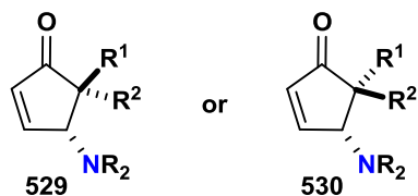
Figure 31. 4-Amino cyclopentenone diastereomers.
