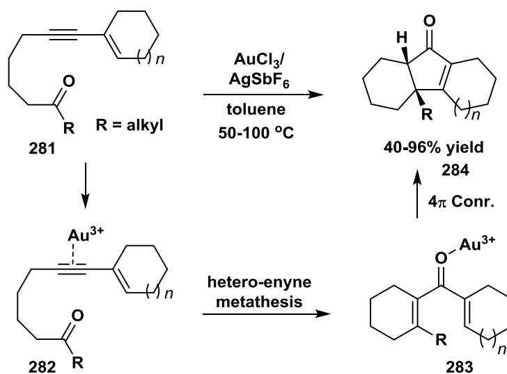
Scheme 40. Gold(I) catalyzed cascade/Nazarov reaction.
