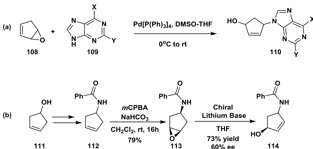
Scheme 13. Epoxides for synthesis of 1-hydroxy 4-aminocyclopent-2-enes.
