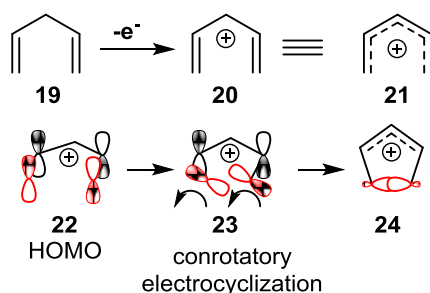
Figure 5. 4\pi Electrocyclization of pentadienyl cations
