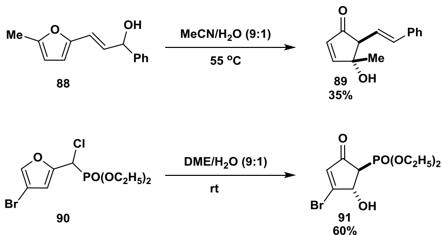
Scheme 8. Alternative activating groups for the Piancatelli rearrangement.
