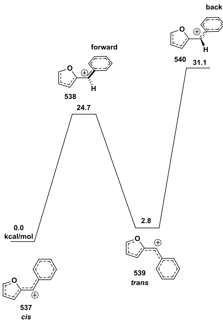
Figure 33. Relative energies of cationic intermediates. Rotational scan calculated using B3LYP/6-31G* (d,p) with 10^\circ intervals. All values in kcal/mol.
