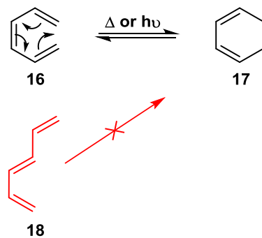
Figure 4. Electrocyclization of 1,3,5-hexatriene.
