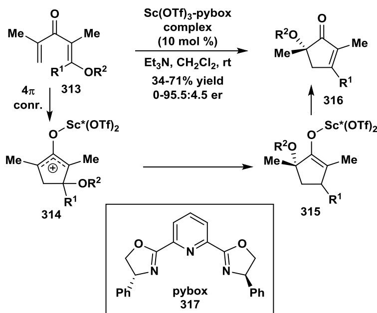
Scheme 47. Enantioselective interrupted Nazarov using oxygen nucleophiles.
