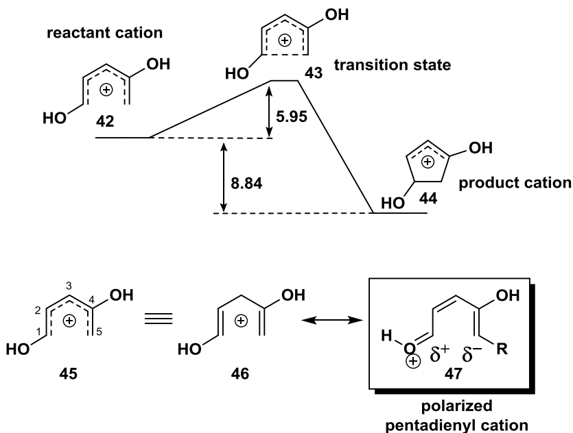
Figure 7. 1,4-Dihydroxy pentadienyl cation energy barrier profile.
