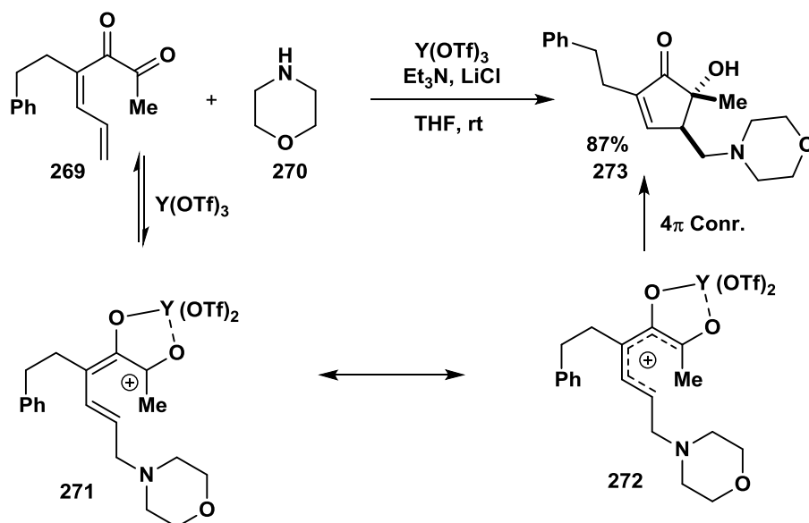
Scheme 37. Conjugate addition initiated Nazarov cyclization.
