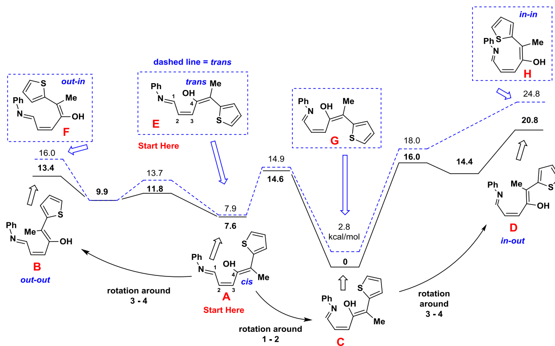
Figure 40. Energy barriers for rotation of the ring opened intermediate derived from methyl-, thiophene-substituted furylcarbinol. Rotational scans calculated using B3LYP/6-31G* (d,p) with 10^\circ intervals. All values in kcal/mol.
