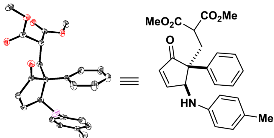
Figure 28. ORTEP drawing of cyclopentenone 468 (left) shown with 50% thermal ellipsoids. Hydrogen atoms have been omitted for clarity. The crystal structure data can be obtained from the Cambridge Crystallographic Data Centre via www.ccdc.cam.ac.uk/data_request/cif . CCDC # 916408
