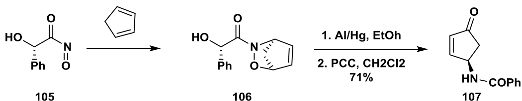
Scheme 12. Acyl nitroso Diels–Alder approach to 4-aminocyclopentenones.
