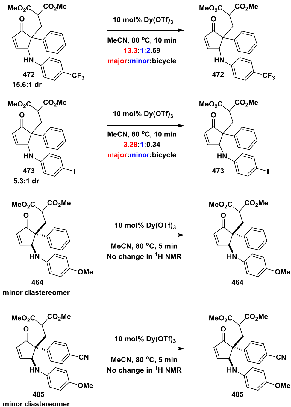
Scheme 74. Reversibility studies.
