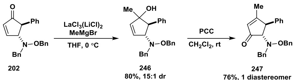
Scheme 33. Allylic transposition of tertiary alcohols.
