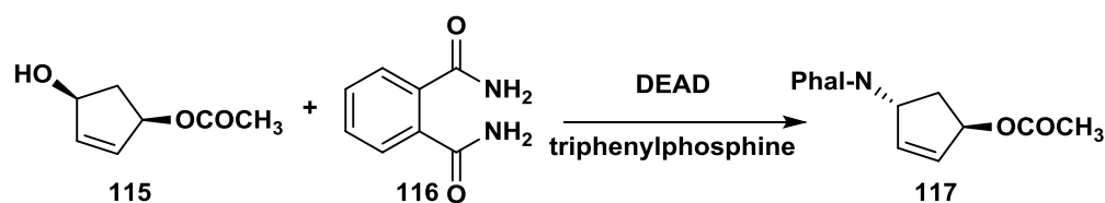
Scheme 14. Formation of 1-hydroxy 4-aminocyclopent-2-enes.
