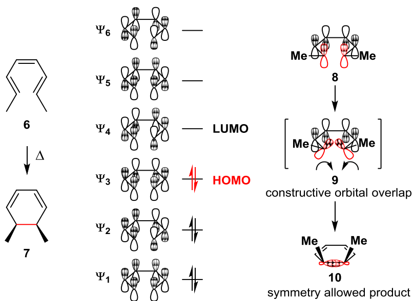
Figure 2. Molecular orbital diagram for a thermally promoted 6\pi electron disrotatory electrocyclic ring closure.
