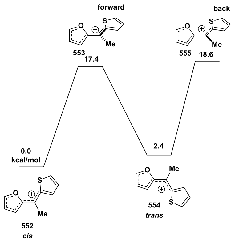
Figure 38. Methyl-, thiophene-substituted furyl carbocation geometries. Rotational scan calculated using B3LYP/6-31G* (d,p) with 10^\circ intervals. All values in kcal/mol.
