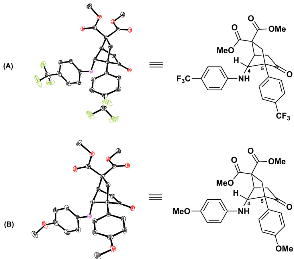
Figure 30. ORTEP drawings of bicyclic intramolecular Michael adducts of 497 (A) and 498 (B) (left) shown with 50% thermal ellipsoids. Hydrogen atoms have been omitted for clarity. The crystal structure data can be obtained from the Cambridge Crystallographic Data Centre via www.ccdc.cam.ac.uk/data_request/cif . CCDC # (A) 901791, (B) 913832.
