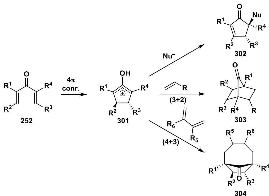
Figure 21. Methods for intercepting the Nazarov oxyallyl cation.
