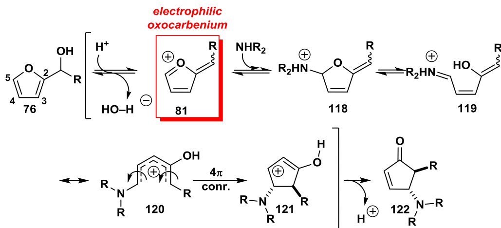
Scheme 15. Proposed mechanism for an aza-Piancatelli rearrangement.
