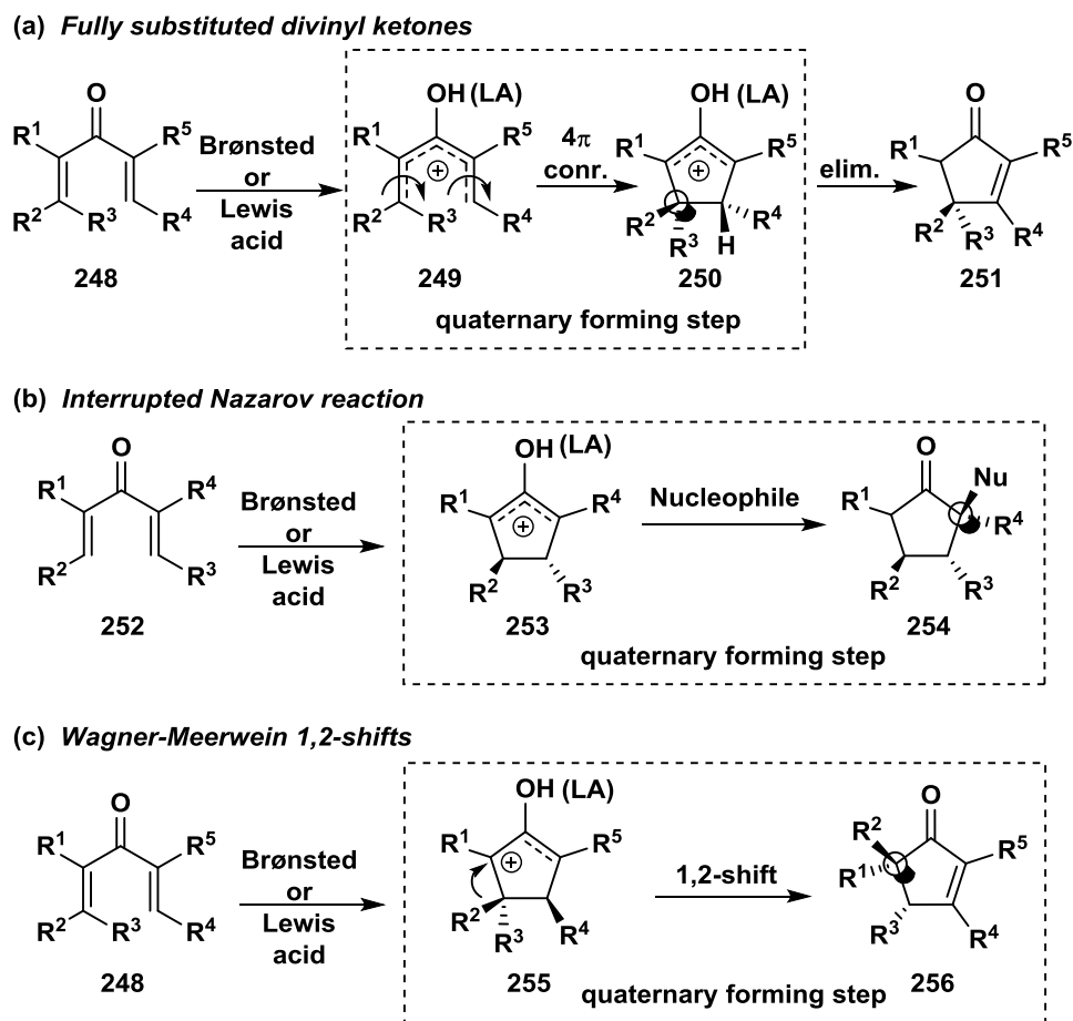
Figure 18. Three ways to form fully substituted centers using the Nazarov cyclization.
