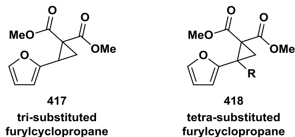
Figure 26. Tri- and tetra-substituted furylcyclopropanes.
