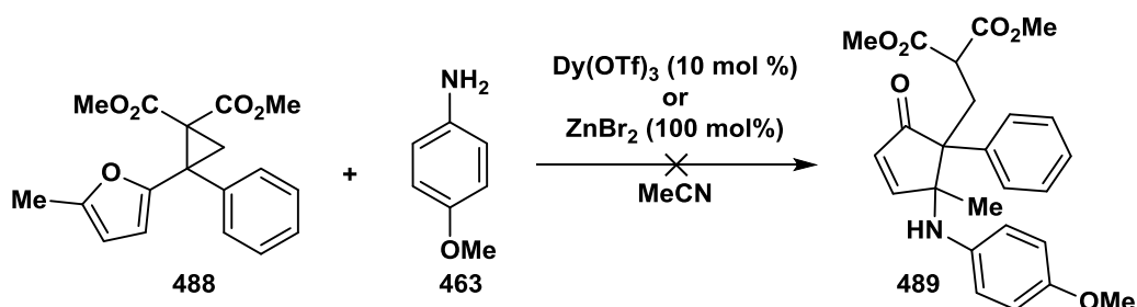
Scheme 67. Attempts to rearrange 5-methyl furylcyclopropanes.
