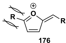
Figure 14. Steric blocking at the 5 position.
