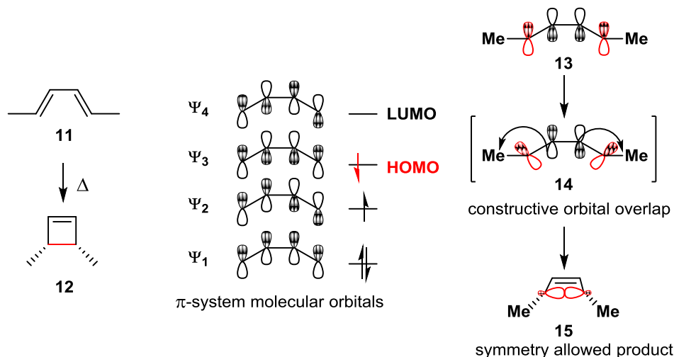
Figure 3. Molecular orbital diagram for a photochemically promoted 4\pi electron disrotatory electrocyclic ring closure.
