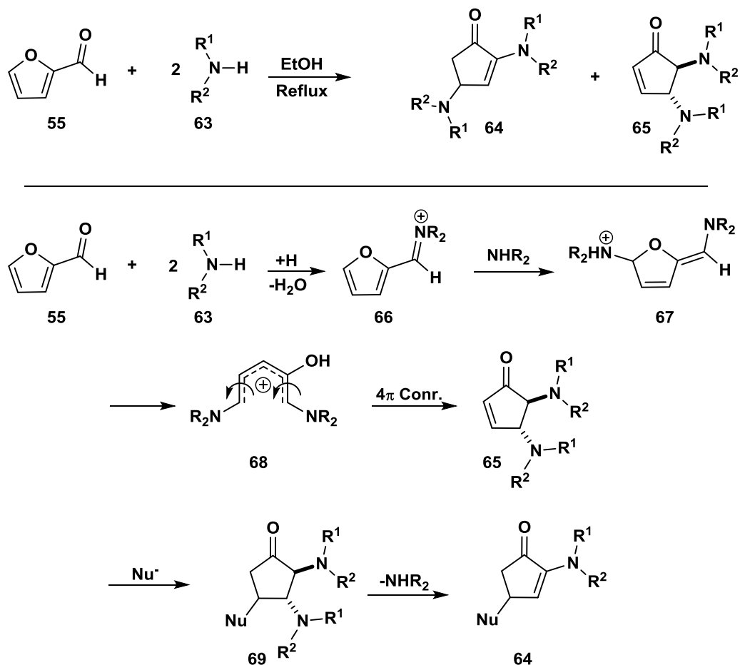
Scheme 6. Conditions and mechanism postulated by Lewis and Mulquiney.
