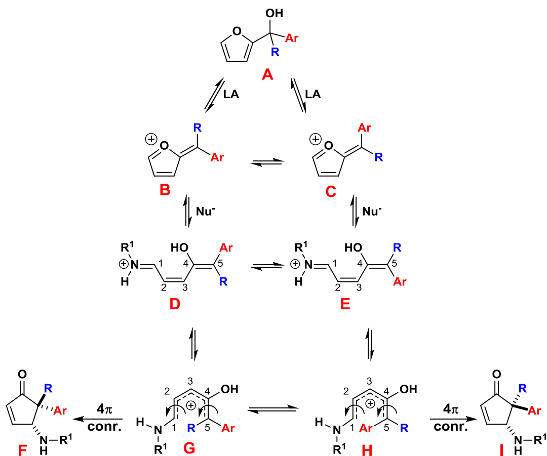
Figure 32. Examination of the mechanism that gives rise to diastereoselectivity.
