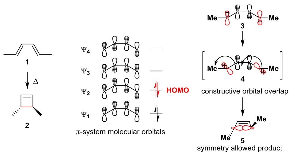
Figure 1. Molecular orbital diagram for a thermally promoted 4\pi electron conrotatory electrocyclic ring closure.
