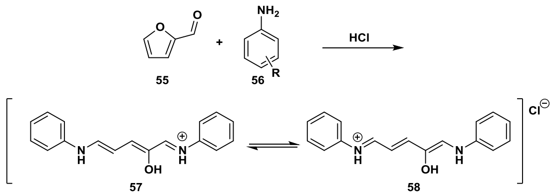
Figure 8. Structure of resonance stabilized Stenhouse salts proposed by Foley.
