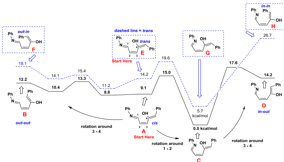
Figure 37. Energy barriers for rotation of the ring opened intermediate derived from phenyl furylcarbinol. Rotational scans calculated using B3LYP/6-31G* (d,p) with 10^\circ intervals. All values in kcal/mol.
