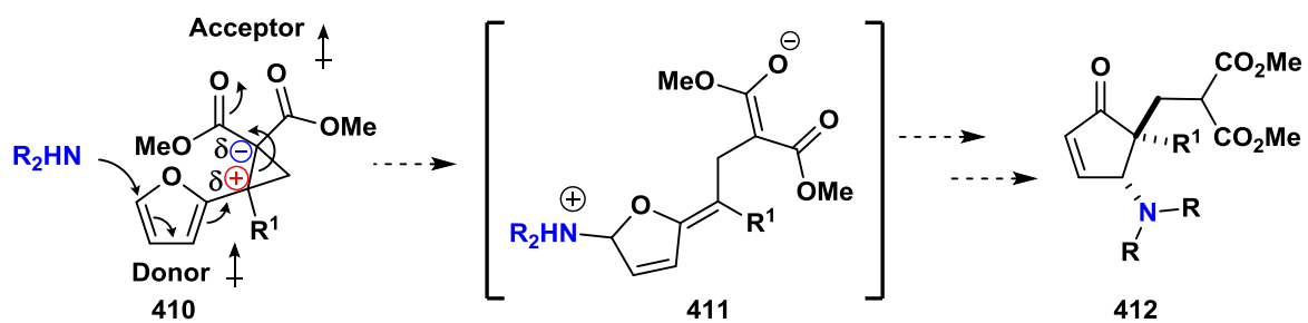
Figure 25. Hypothetical reactivity of furylcyclopropanes.
