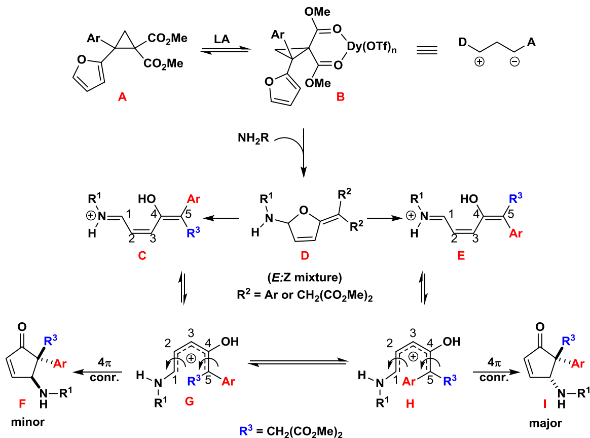
Scheme 69. Origins of diastereoselectivity.
