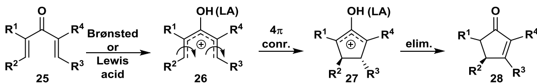
Scheme 1. A prototypical Nazarov cyclization.
