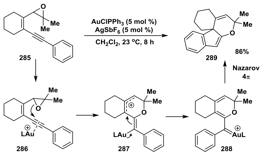
Scheme 41. Cascade sequence that generates a pentadienyl cation equivalent.
