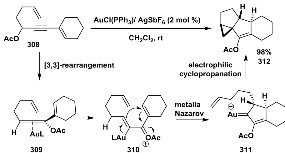
Scheme 46. Gold(I) catalyzed Nazarov reaction.
