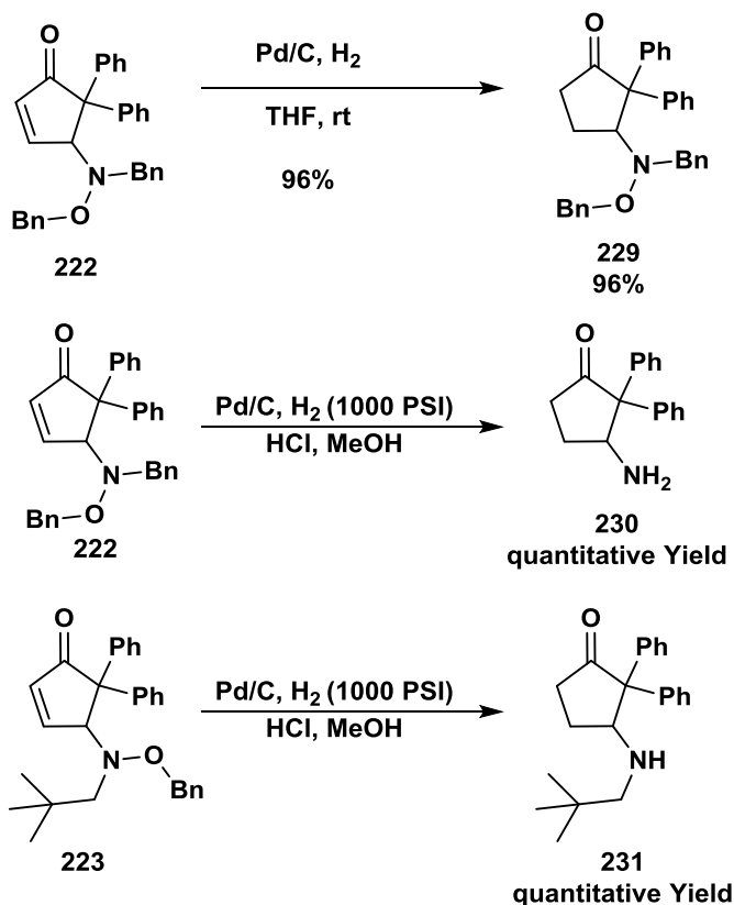
Scheme 30. Hydrogenation conditions for breaking the N-O bond.
