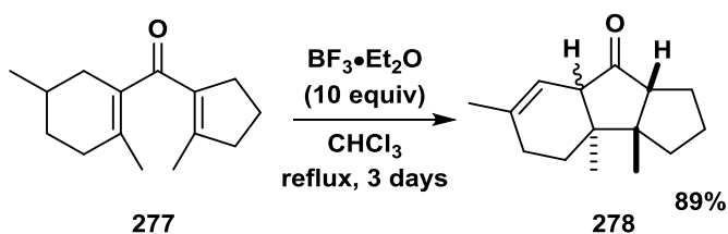
Scheme 38. Fully substituted terminal divinyl ketones.
