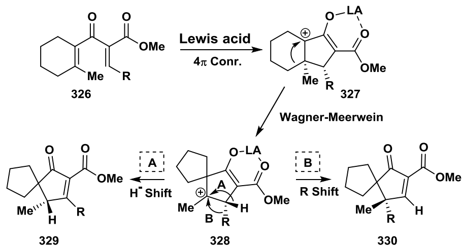
Figure 22. Cationic Wagner-Meerwein shifts.
