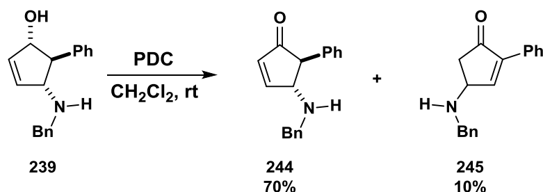
Scheme 32. Formation of amino cyclopentenones bearing an aliphatic amine.
