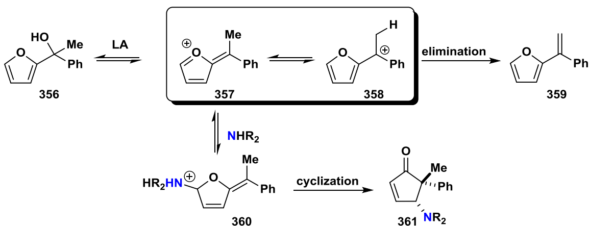
Scheme 56. Competitive elimination using tertiary furylcarbinols.
