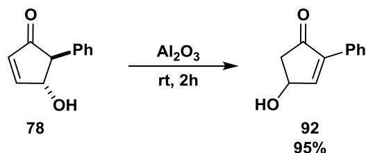
Scheme 9. Isomerization of 4-hydroxycyclopentenones by absorption on basic alumina.
