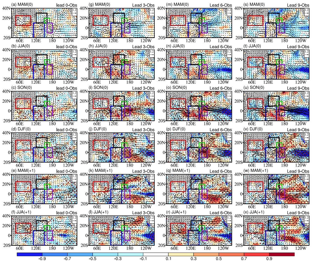
Fig. 8 Differences between composited EP El Niño 850 hPa wind (vector, unit: m/s) and SST anomalies (shaded, unit: °C) in the 0-month lead (1st column), 3-month lead (2nd column), 6-month lead (3rd column), and 9-month lead (4th column) and the observations. The evolution spans from El Niño's developing spring (MAM (0); 1st row), summer (JJA (0); 2nd row), developing autumn (SON (0); 3rd row), peak winter (DJF (0); 4th row), decaying spring (MAM (1); 5th
