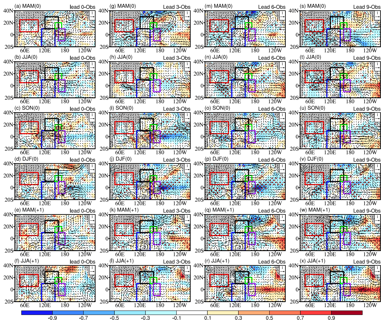
Fig. 9 Same as Fig. 8 but for the CP-I El Niño
