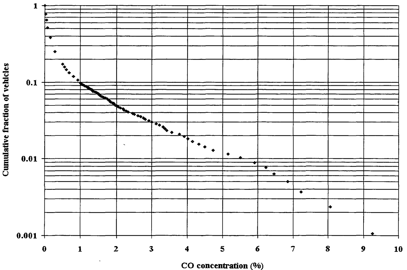
Figure A.16. Stephans plot of distribution of CO emissions from MY87 fuel-injected vehicles (CARB 1991 Remote Sensing Data)
