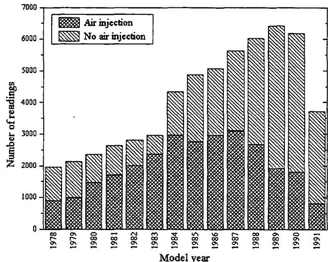
Figure A.15. Number of readings by air injection system and MY
