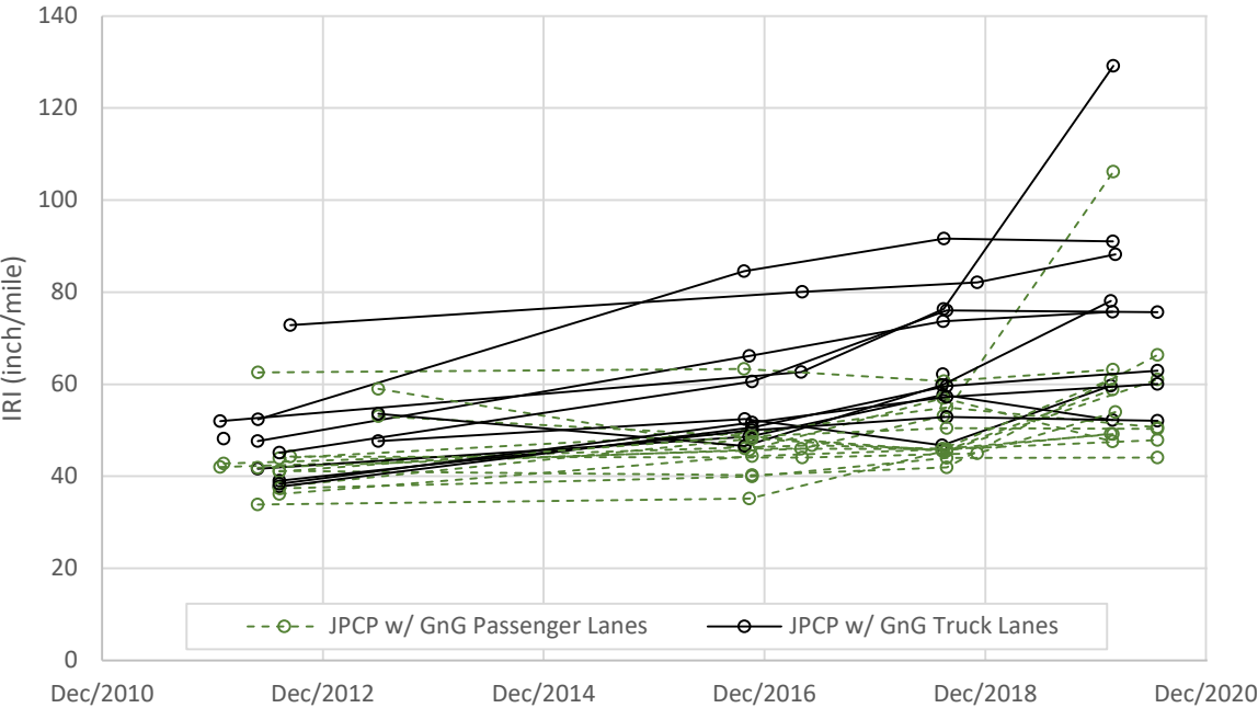
Figure 4.20: IRI on JPCP with GnG truck and passenger lanes.
