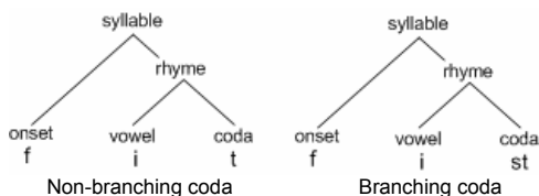
Figure 1: Syllabic structure.
