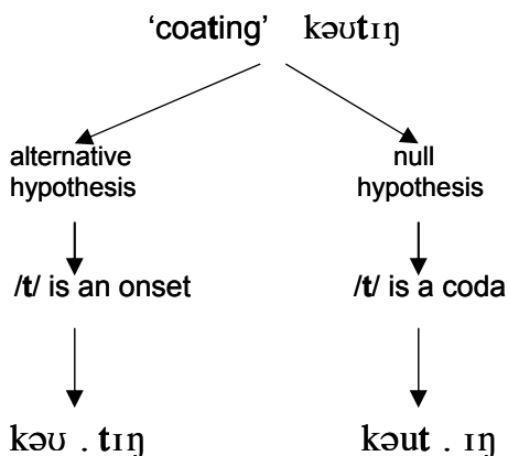
Figure 4: Syllabification hypotheses.
