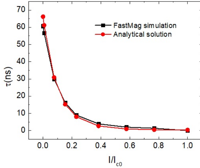
Figure 6.3: Thermal relaxation time of a macrospin calculated from the forward flux sampling and analytical formula. The model used for finite elements simulations is a 5 \times 5 \times 5 \text{nm}^3 cube with an energy barrier of 5.16k_B T . The computed thermal activation time is \tau_0 = 0.38 \text{ns} and \alpha = 2 .
