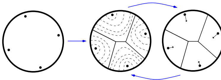
Fig. 5.1: The three steps of the Bubble framework. Black nodes indicate the seed nodes. On the left hand side, seed nodes are found. In the middle, a partition is found by performing breadth-first searches around the seed nodes and on the right hand side new seed nodes are found.
