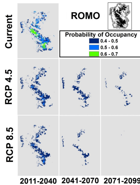
Fig. 4. Example of a pika population predicted to experience a steady decline throughout this century in an area near Niwot Ridge, Rocky Mountain National Park (ROMO). Shown are the total potential habitats and predicted occupant probability using an ensemble climate model with two carbon forcings; RCP 8.5, a “business as usual,” “high emissions,” “worst-case” scenario, and RCP 4.5, a stabilization scenario, where warming is stabilized by reductions in greenhouse gas emissions. (After Schwaln et al. 2016.)
