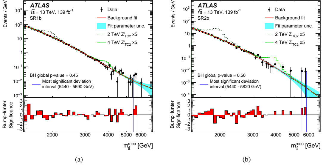
Figure 3: Observed m_{ii}^{\text{reco}} distributions in data for (a) SR1b and (b) SR2b, shown together with the result of the fit with the three-shape-parameter function. The shaded bands around the fits indicate the effect of the fit parameter uncertainty on the background prediction. The bin width of the distributions is chosen to be the same as that used in the background parameterization (Section 5.2). The predicted Z'_{\text{TC}2} signal distributions with masses of 2 and 4 TeV (multiplied by a factor of 5) are superimposed on the background prediction. The lower panel shows the significance of data with respect to the background prediction from the fit, calculated in continuous mass intervals scanned over the binned m_{ii}^{\text{reco}} distributions. The two vertical lines extending between the upper and lower panel represent the most significant deviation interval. The global p -value of the interval is 0.45 (0.56) for SR1b (SR2b).
