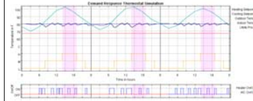
(b) Three day simulation with fixed precooling start point
