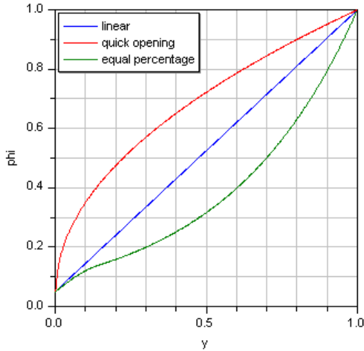
Figure 2: Flow characteristic \phi(y) for valves.
