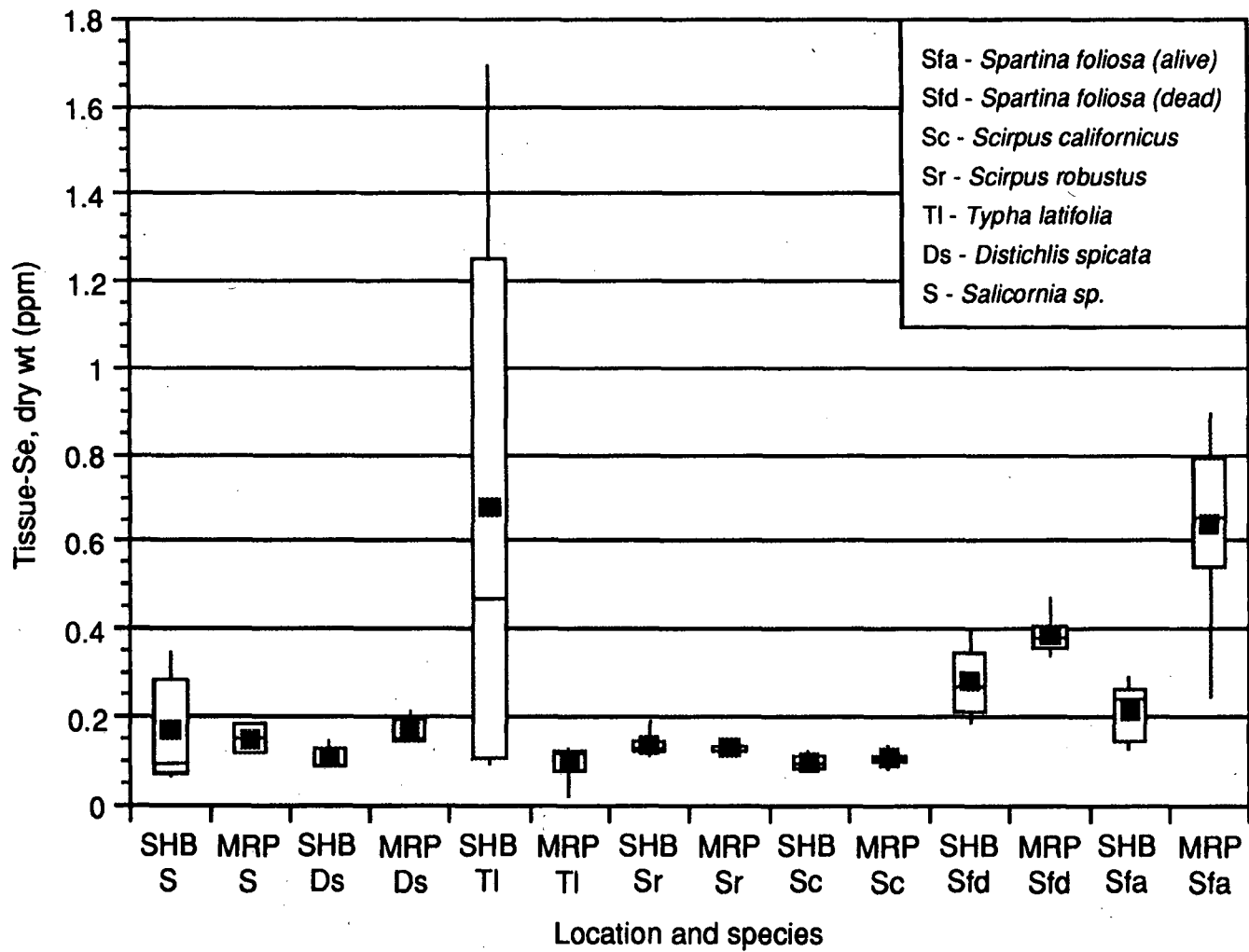
Figure 5.2 Species-specific tissue-Se concentrations of aboveground parts at sites MRP and SHB.
