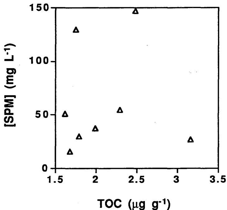
Figure 3.1. Suspended particulate matter (SPM) concentrations from 12/1/95-1/29/96, plotted versus the total organic carbon concentration (TOC).
