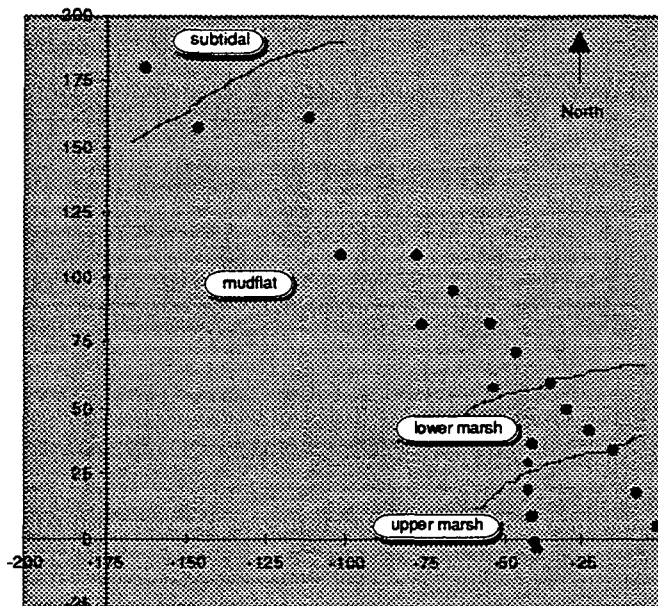
Figure 2.1 Location of core sampling points relative to the intertidal environments at MRP.
