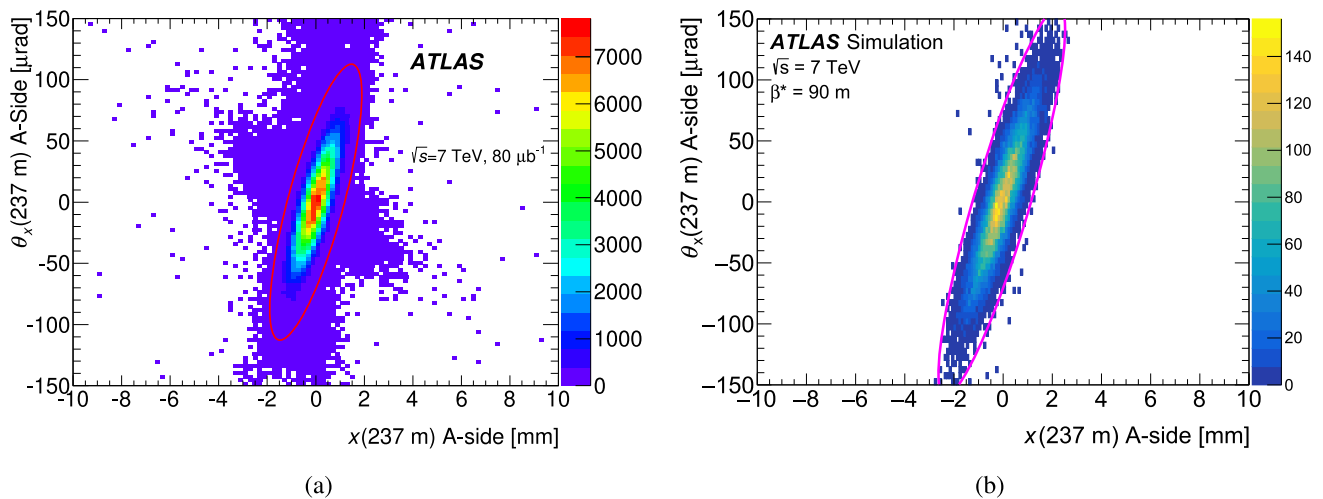
Fig. 4 The correlation between the reconstructed position of a proton at |z| = 237 m (A-side; a similar correlation is measured for the C-side) and its local angle projection on the horizontal direction. In a the proton candidates in elastic proton–proton data lie within the area of
