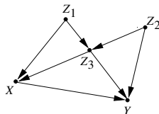
FIG 3. Markovian model illustrating the derivation of the causal effect of X on Y , Eq. (20). Error terms are not shown explicitly.
