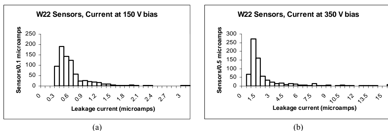
Fig. 14: Leakage currents for CiS W22 sensors measured at 20 °C and ~ 50% RH (a) at 150 V bias, average value 0.59 \mu\text{A} , (b) at 350 V bias, average value 2.32 \mu\text{A} .
