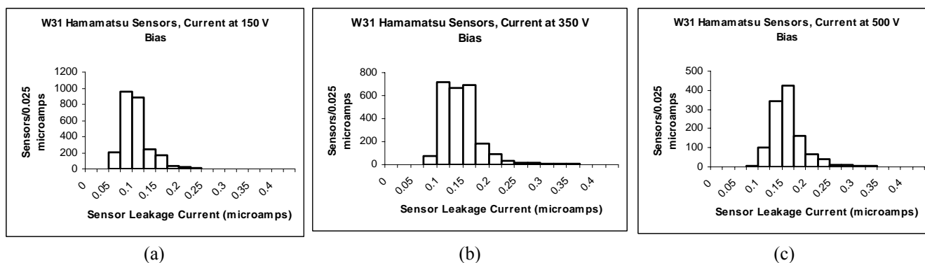
Fig. 13: Leakage currents for Hamamatsu W31 sensors measured at 20 °C (a) at 150 V bias, average value 0.09 \mu\text{A} , (b) at 350 V bias, average value 0.14 \mu\text{A} , (c) at 500 V bias, average value 0.16 \mu\text{A} .
