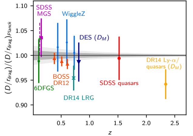
Fig. 11. Acoustic-scale distance measurements divided by the corresponding mean distance ratio from Planck TT,TE,EE +lowE+lensing in the base- \Lambda CDM model. The points, with their 1\sigma error bars are as follows: green star, 6dFGS (Beutler et al. 2011); magenta square, SDSS MGS (Ross et al. 2015); red triangles, BOSS DR12 (Alam et al. 2017); small blue circles, WiggleZ (as analysed by Kazin et al. 2014); large dark blue triangle, DES (DES Collaboration 2019); cyan cross, DR14 LRG (Bautista et al. 2018); red circle, SDSS quasars (Ata et al. 2018); and orange hexagon, which shows the combined BAO constraints from BOSS DR14 Lyman- \alpha (de Sainte Agathe et al. 2019) and Lyman- \alpha cross-correlation with quasars, as cited in (Blomqvist et al. 2019). The green point with magenta dashed line is the 6dFGS and MGS joint analysis result of Carter et al. (2018). All ratios are for the averaged distance D_V(z) , except for DES and BOSS Lyman- \alpha , where the ratio plotted is D_M (results for H(z) are shown separately in Fig. 16). The grey bands show the 68% and 95% confidence ranges allowed for the ratio D_V(z)/r_{\text{drag}} by Planck TT,TE,EE+lowE+lensing (bands for D_M/r_{\text{drag}} are very similar).
