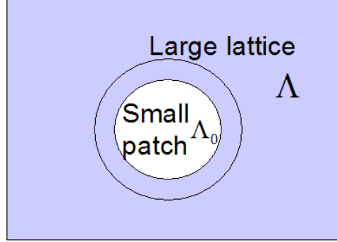
Figure 15: The deterministic concept of micro-canonical ensemble defined on \Lambda \rightarrow \mathbf{Z}^2 produces the probabilistic concept of Markov random field on a fixed patch \Lambda_0 , according to the equivalence of ensemble in statistical physics.
