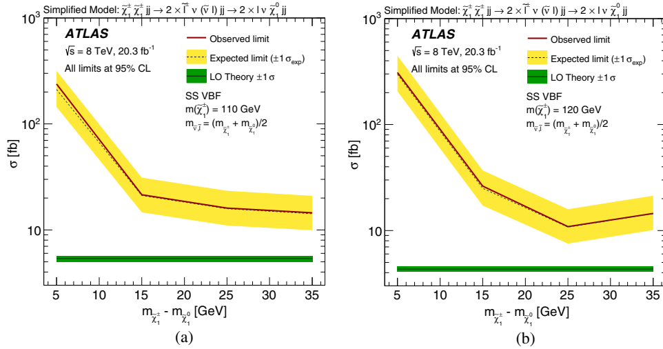
FIG. 14. The 95% CL upper limit on the signal cross section for VBF \tilde{\chi}_1^\pm \tilde{\chi}_1^\pm production for (a) m(\tilde{\chi}_1^\pm) = 110 GeV and (b) m(\tilde{\chi}_1^\pm) = 120 GeV. The limits are set with respect to the mass difference between the \tilde{\chi}_1^\pm and \tilde{\chi}_1^0 , and use the results from the same-sign, two-lepton VBF analysis.
