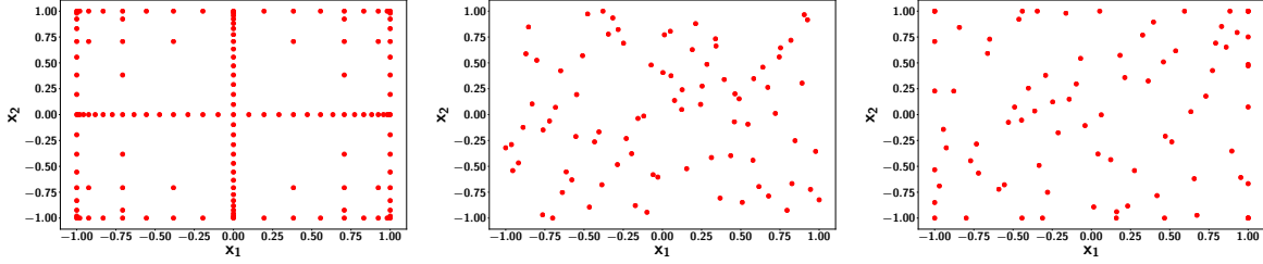
(a) 2D Sparse grid of level 5 with 145 points. (b) 2D Latin hypercube sample with 84 points. (c) 2D decoupled Latin hypercube Design with 84 points.
