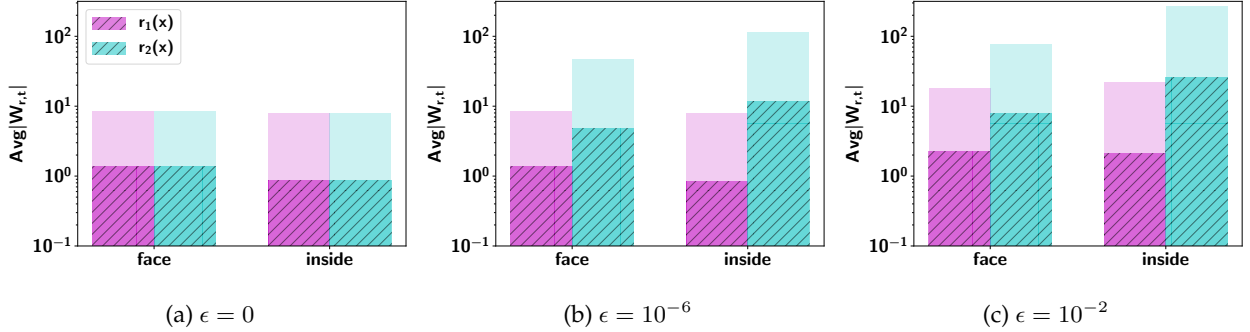
Figure 7: Comparison of the average number of polelike points found over all functions in Table A.5 for different relative noise levels \epsilon . The data is sampled with d-LHD. Each bar represents the average number of polelike points found when t \geq 10^2 . The average number of polelike points found when t \geq 10^3 is shown as a hatched bar. The average number of polelike points found when 10^2 \leq t < 10^3 is shown as a faded bar. The number of polelike points found in r_3(x) is 0 for all noise levels.
