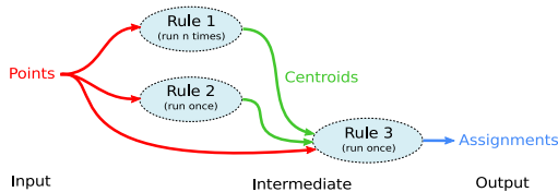
Fig. 2. Dependency graph for kmeans example. The rules are the vertices while each edge represents the dependencies of each rule. Each edge color corresponds to each named data dependence in the pseudocode.
