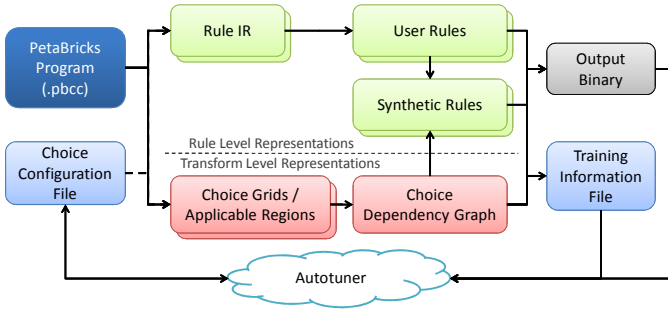
Fig. 4. Flow for the compilation of a PetaBricks program with a single transform. (Additional transforms would cause the center part of the diagram to be duplicated.)
