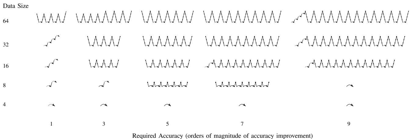
Fig. 9. Resulting cycle shapes for Helmholtz after tuning for different input data sizes and required accuracies. The solid arrows at the bottom of the cycles represent shortcut calls to the direct solver, while the dashed arrows represents an iterative solve using SOR. The dots present in the cycle represent single relaxations. Note that some paths in the full multigrid cycles skip relaxations while moving to a higher grid resolution. The notation of these diagrams is similar to that of [9].
