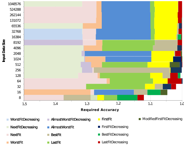
Fig. 7. Best algorithm for each accuracy and input size in the Bin Packing benchmark. By best we mean on the optimal frontier (there exists no algorithm with better performance and accuracy for a given input size on average). Accuracy is defined as the number of bins over the optimal number of bins achievable. Lower numbers represents a higher accuracy.
