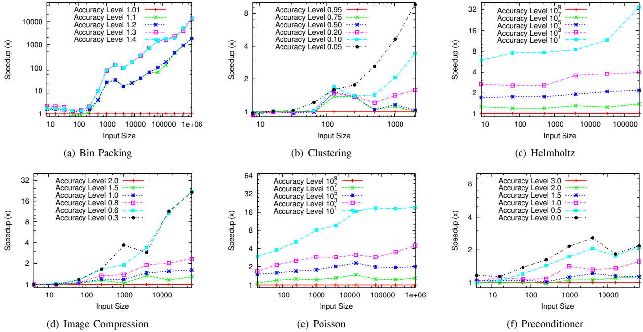
Fig. 6. Speedups for each accuracy level and input size, compared to the highest accuracy level for each benchmark. Run on an 8-way ( 2 \times 4 -core Xeon X5460) system.
