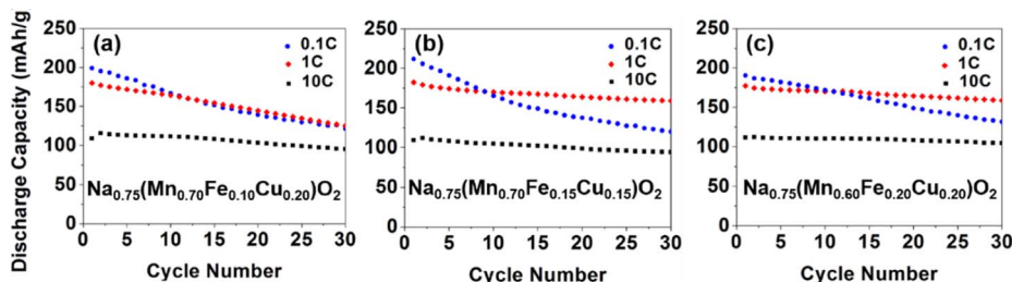
Figure 4. Rate performance of MnFeCu-based compounds cycled at 0.1 C, 1 C and 10 C between 1.5 V and 4.5 V: (a) \text{Na}_{0.75}\text{Mn}_{0.70}\text{Fe}_{0.10}\text{Cu}_{0.20}\text{O}_2 ; (b) \text{Na}_{0.75}\text{Mn}_{0.70}\text{Fe}_{0.15}\text{Cu}_{0.15}\text{O}_2 ; (c) \text{Na}_{0.75}\text{Mn}_{0.60}\text{Fe}_{0.20}\text{Cu}_{0.20}\text{O}_2 .
