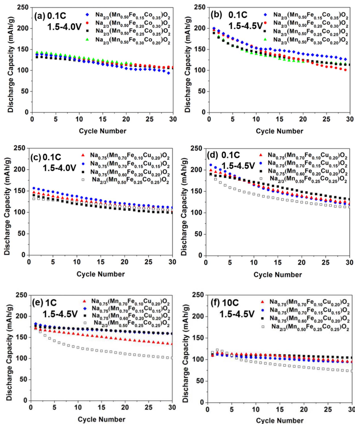
Figure 3. Cyclability of MnFeCo-based and MnFeCu-based compounds at different voltage window and rates: (a) MnFeCo-based compounds cycled at 0.1 C between 1.5 V and 4.0 V; (b) MnFeCo-based compounds cycled at 0.1 C between 1.5 V and 4.5 V; (c) MnFeCu-based compounds and \text{Na}_{2/3}(\text{Mn}_{0.50}\text{Fe}_{0.25}\text{Co}_{0.25})\text{O}_2 cycled at 0.1 C between 1.5 V and 4.0 V; (d) MnFeCu-based compounds and \text{Na}_{2/3}(\text{Mn}_{0.50}\text{Fe}_{0.25}\text{Co}_{0.25})\text{O}_2 cycled at 0.1 C between 1.5 V and 4.5 V; (e) MnFeCu-based compounds and \text{Na}_{2/3}(\text{Mn}_{0.50}\text{Fe}_{0.25}\text{Co}_{0.25})\text{O}_2 cycled at 1 C between 1.5 V and 4.5 V; (f) MnFeCu-based compounds and \text{Na}_{2/3}(\text{Mn}_{0.50}\text{Fe}_{0.25}\text{Co}_{0.25})\text{O}_2 cycled at 10 C between 1.5 V and 4.5 V.
