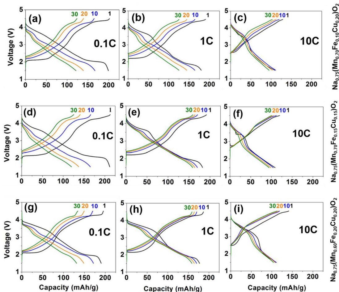
Figure 2. Galvanostatic charge and discharge profiles of MnFeCu-based half cell in 1 st , 10 th , 20 th , 30 th cycle: (a)(b)(c) \text{Na}_{0.75}\text{Mn}_{0.70}\text{Fe}_{0.10}\text{Cu}_{0.20}\text{O}_2 ; (d)(e)(f) \text{Na}_{0.75}\text{Mn}_{0.70}\text{Fe}_{0.15}\text{Cu}_{0.15}\text{O}_2 ; (g)(h)(i) \text{Na}_{0.75}\text{Mn}_{0.60}\text{Fe}_{0.20}\text{Cu}_{0.20}\text{O}_2 ; (a)(d)(g) tested at 0.1 C rate; (b)(e)(h) tested at 1 C rate; (c)(f)(i) tested at 10 C rate. All is predischarged to 1.5 V and then cycled between 1.5 V and 4.5 V.
