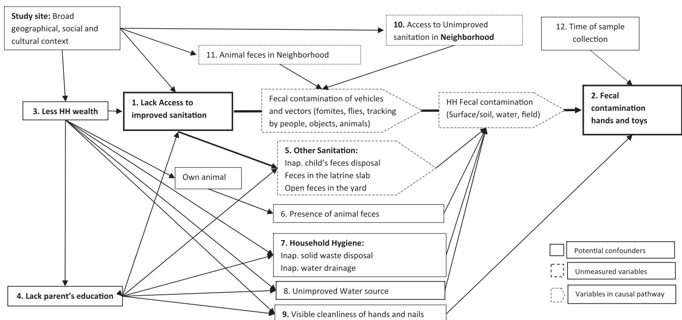
FIGURE 1. Directed acyclic graph showing the variables that were measured and included in the multivariable analysis.
