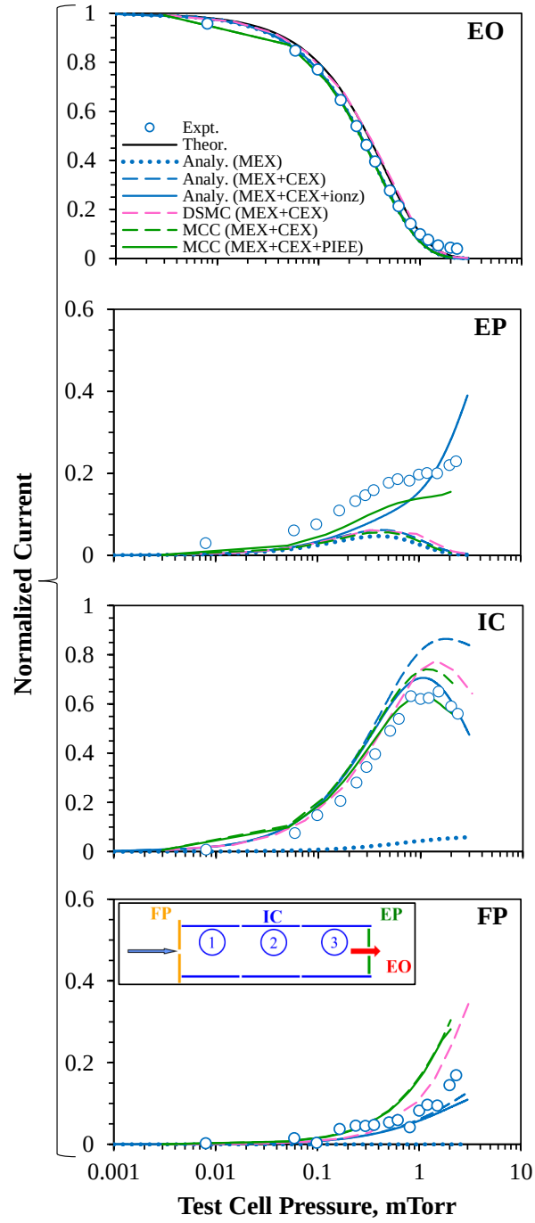
Figure 3.13: Results from the semi-analytical and computational models of current to the exit orifice (EO), exit plate (EP), inner cylinders (IC), and front plate (FP) as a function of test cell pressure. Contributions from MEX ions (dotted lines), from MEX and CEX ions (dashed lines), and from ions and electrons (solid lines) are shown. Electrons from neutral-neutral ionization collisions are considered in the semi-analytical model, while particle-induced electron emission is considered in the MCC model.
