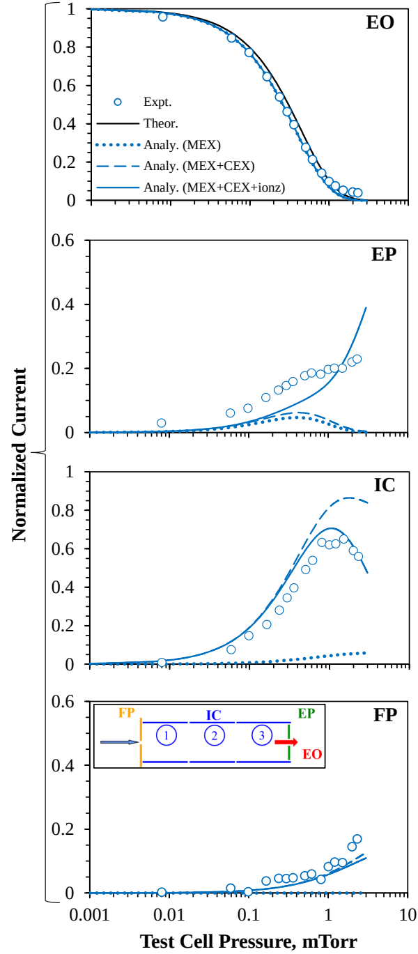
Figure F.7: Results from the semi-analytical model of current to the exit orifice (EO), exit plate (EP), inner cylinders (IC), and front plate (FP) as a function of test cell pressure. Contributions from MEX ions (dotted line), from MEX and CEX ions (dashed line), and from ions and electrons (solid lines) are shown, where electrons are assumed to be generated in neutral-neutral ionization collisions. Current calculated from Equation 3.9 with \Delta x = L and \sigma_{tot} = \sigma_{CEX} is compared to exit orifice current.
