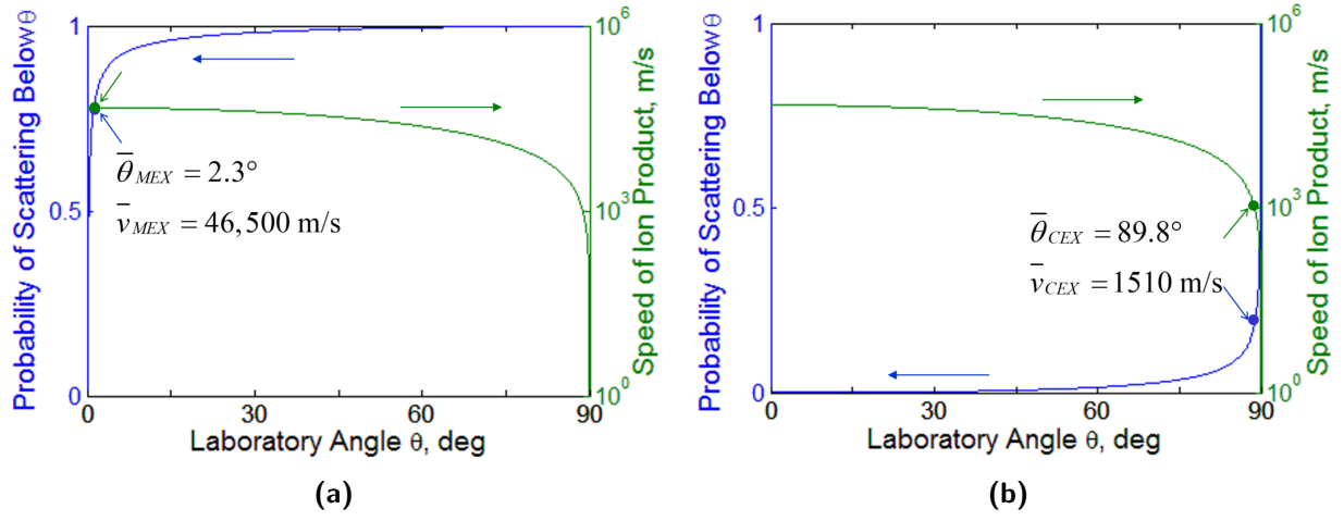
Figure 3.12: Cumulative probability of scattering below angle \theta , speed of an ion scattered at angle \theta , and average values of each for (a) MEX and (b) CEX ions; \text{Xe}^+\text{-Xe} at 1500 eV.
