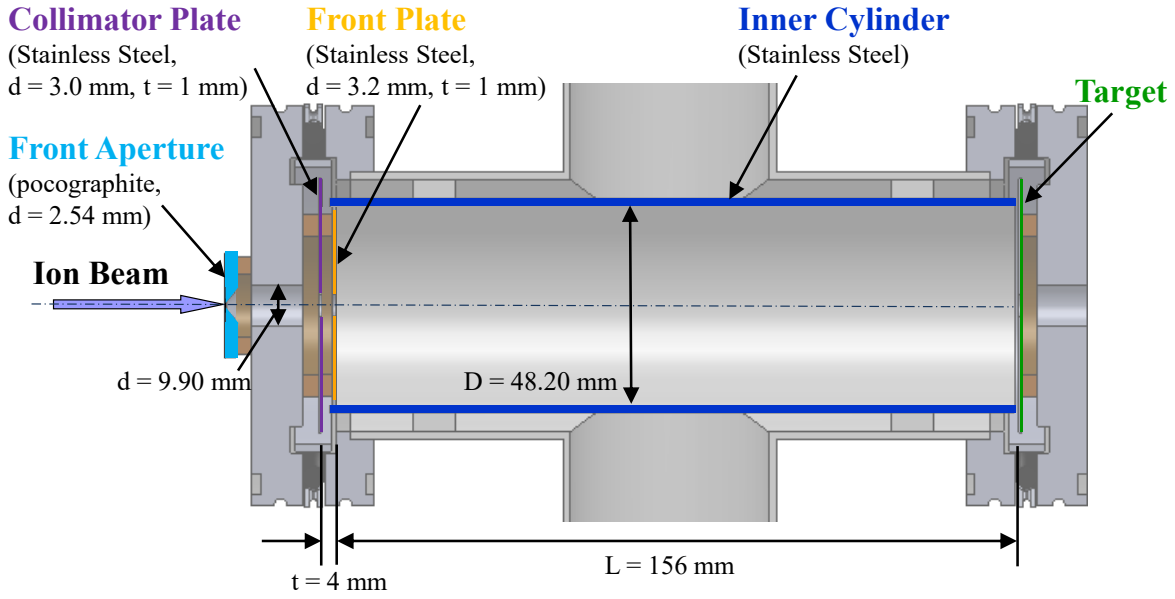
Figure G.1: Test cell electrodes for measuring ion-induced electron emission properties of conducting materials. Important materials and dimensions are included.
