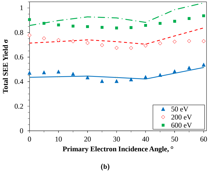
Figure 4.29: Computational results (shown as lines) of total SEE yield dependence on (a) incidence energy and (b) incidence angle for W fuzz. Experimental data is reproduced.
