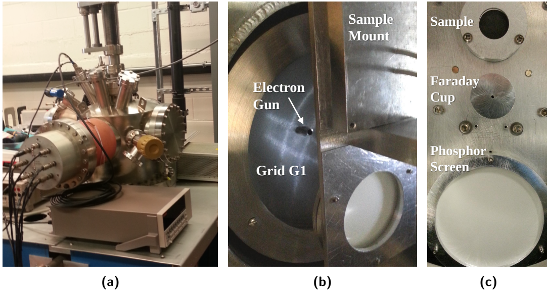
Figure 4.2: Facility for measuring secondary electron emission from graphite, including (a) chamber, (b) LEED/AES electron optics, and (c) sample mount.
