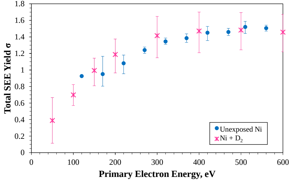
Figure 4.27: Total SEE yield measured for 50-600 eV, 0° primary electrons impacting clean Ni(110) and Ni(110) exposed to D 2 + .
