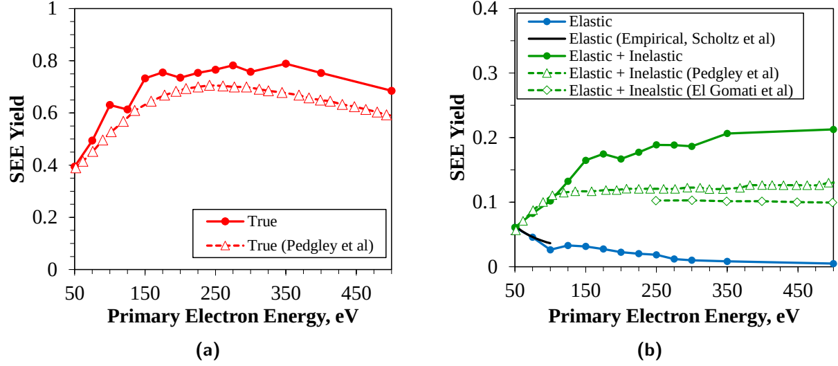
Figure 4.19: Yields of elastically reflected, inelastically reflected, and true secondary electrons versus primary electron energy for graphite. Comparison are made to previous measurements by Pedgley et al [12] and El Gomati et al [21] and to values calculated using Equation 4.6 [17].
