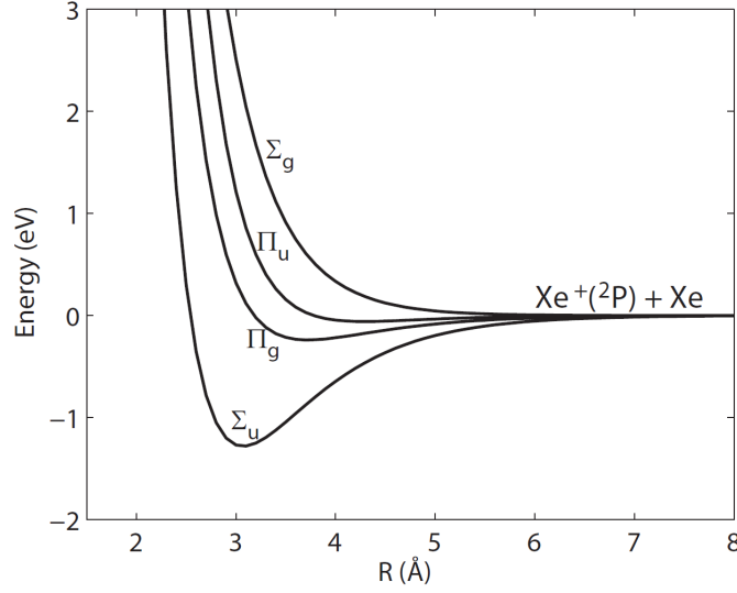
Figure 2.3: \text{Xe}^+ - \text{Xe} spin-orbit free interaction potential [8, 9].
