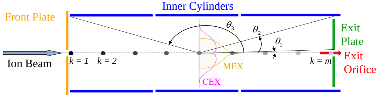
Figure 3.10: Test cell with attenuated MEX and CEX sources, MEX and CEX scattering angular distributions, and electrodes with bounding angles.
