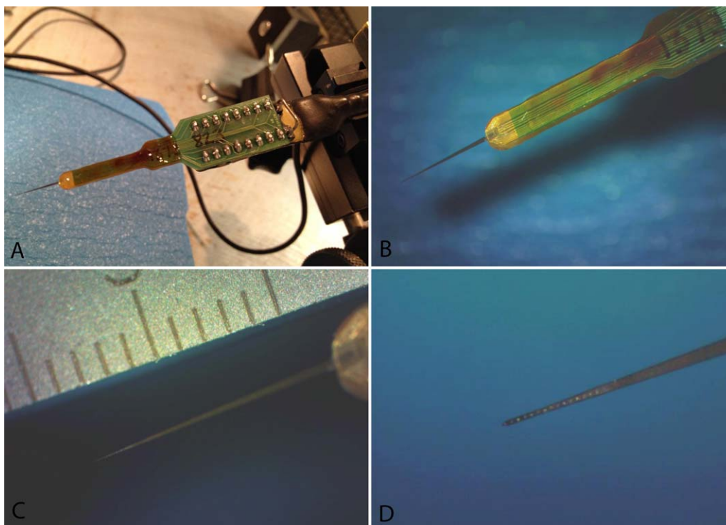
Fig. 1. (A) Photograph of a NeuroNexus 16-channel stimulating electrode array (NeuroNexus, Ann Arbor, MI) in position on a micropositioner. (B) Microscopic picture of the shank and distal board. (C) The silicon-substrate shank with a metric ruler-size reference. (D) High-magnification microscopic photograph of the distal end of the penetrating shank. The 16 electrode sites can be seen. Superficial or proximal electrodes are those furthest from the tip of the array (to the right in this picture), whereas deep or distal electrodes are those closest to the array tip (to the left). [Color figure can be viewed in the online issue, which is available at www.laryngoscope.com .]
