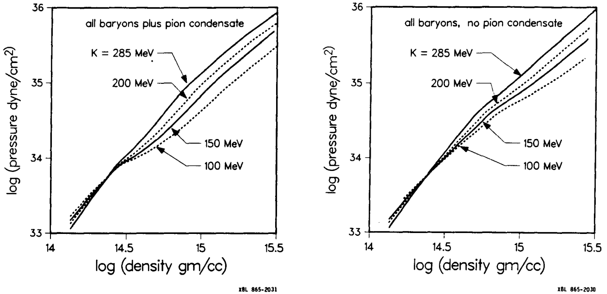
Fig. 1. The equation of state for various compressibilities when (a) free pions condense, and (b) when they do not. These are limiting cases for the role of pions.
