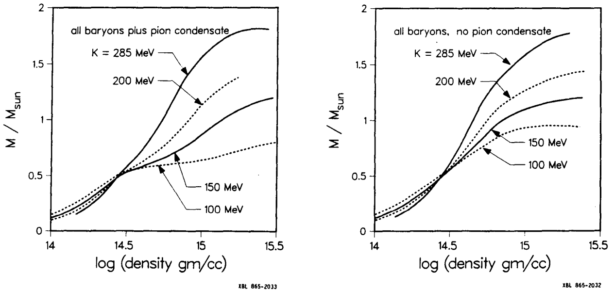
Fig. 2. The masses of neutron stars as a function of their central density for various nuclear compressibilities, in the two cases (a) free pions condense and (b) pions do not condense. These are limiting cases as concerns the effect of pions.
