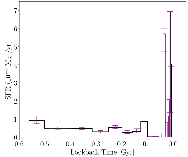
Figure 7. The absolute SFH of the ACS field over the most recent 500 Myr. In general, the SFH over the last 500 Myr has been fairly constant, with larger amplitude bursts within the more recent 10 Myr.
