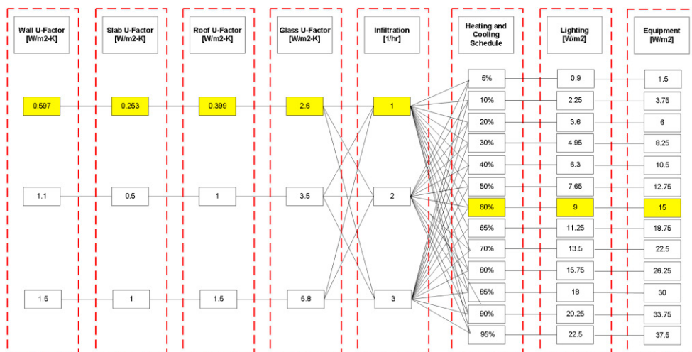
Figure 4 117 parametric combinations of the small office building model
