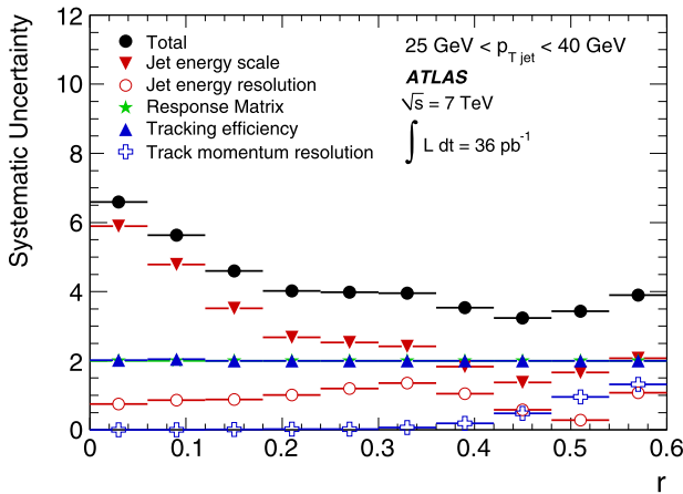
Fig. 3 Systematic uncertainty in \rho_{\text{ch}}(r, p_{T\text{jet}}) from uncertainties in the jet energy scale and resolution, the track reconstruction efficiency and momentum resolution and the response matrix for
