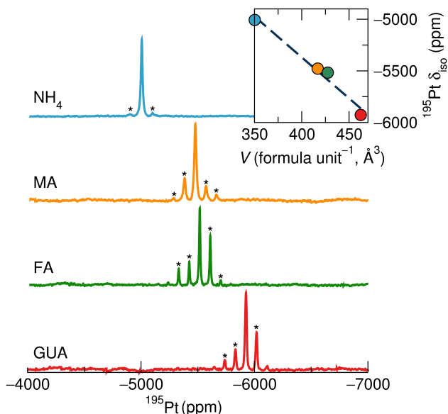
Figure 3: Room temperature 10 kHz MAS ^{195}\text{Pt} NMR spectra of \text{A}_2\text{PtI}_6 showing the influence of the counteranion on chemical shift and lineshape. Asterisks indicate spinning sidebands, shifts are referenced to a 1 M solution of \text{Na}_2\text{PtCl}_6 in \text{D}_2\text{O} (0 ppm), and the field is 11.7 T (500 MHz for ^1\text{H} ). Inset: Isotropic ^{195}\text{Pt} chemical shift, \delta_{iso} , is correlated with unit cell volume per formula unit, V / \text{F.U.} A dashed line is drawn as a visual guide.
