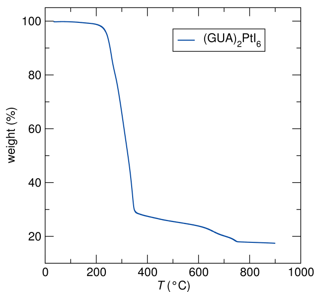
Figure S14: TGA data for (GUA) 2 PtI 6 from room temperature to 900°C.
