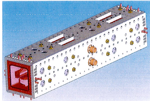
Figure 1: CAD model of a single RFQ module.
