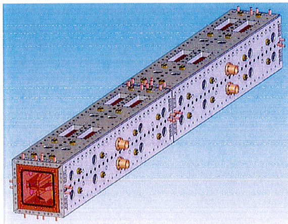
Figure 3: CAD model of the entire RFQ.
