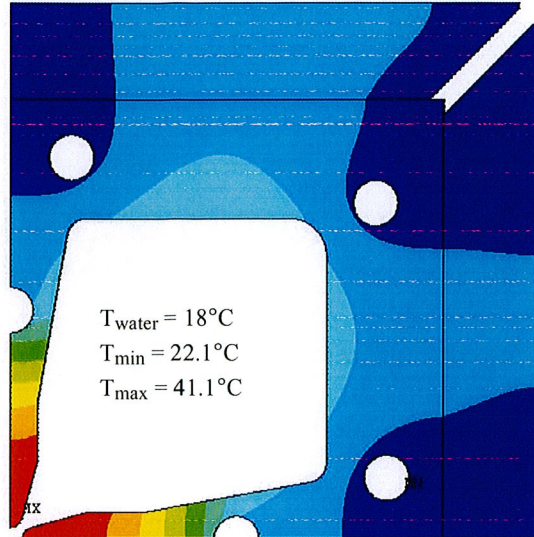
Figure 5: Temperature distribution in one RFQ quadrant.
