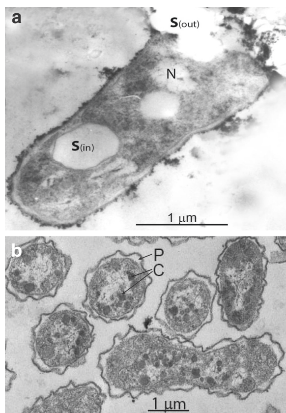
Fig. 1 Thin section electron microscopy photographs of cells of strain ARh 1 T grown with thiocyanate in batch (a) and chemostat (b) cultures at pH 10 and 0.6 M total Na + . S (in) - intracellular sulfur globe; S (out) - excreted sulfur globe damaging the cell membrane and the wall; N - nucleoid; C - carboxysomes
