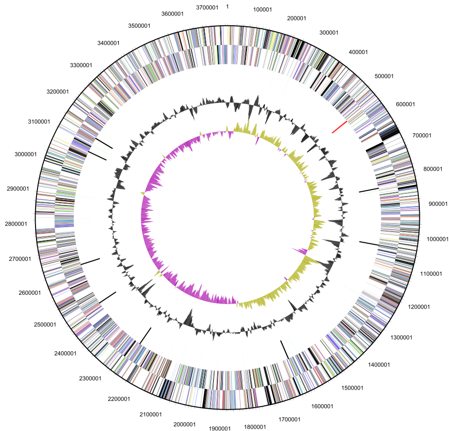
Fig. 3 Genome map of Thioalkalivibrio paradoxus ARh 1 T . From outer to inner ring: genes on the forward strand; genes on the reverse strand; RNA genes (tRNA: green; rRNA: red; other: black); GC content and GC skew
