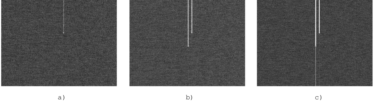
Figure 9. Sub-images of a 10.5\ \mu\text{m} pixel CCD taken under dark conditions at -140\ ^\circ\text{C} for various substrate bias voltages. The readout direction is to the bottom. The images were taken by immediately reading out the CCD after a clear operation. The readout time is approximately 12 seconds. The sub-images are approximately 290 \times 220 pixels. a) 160V, b) 180V, and c) 200V.
