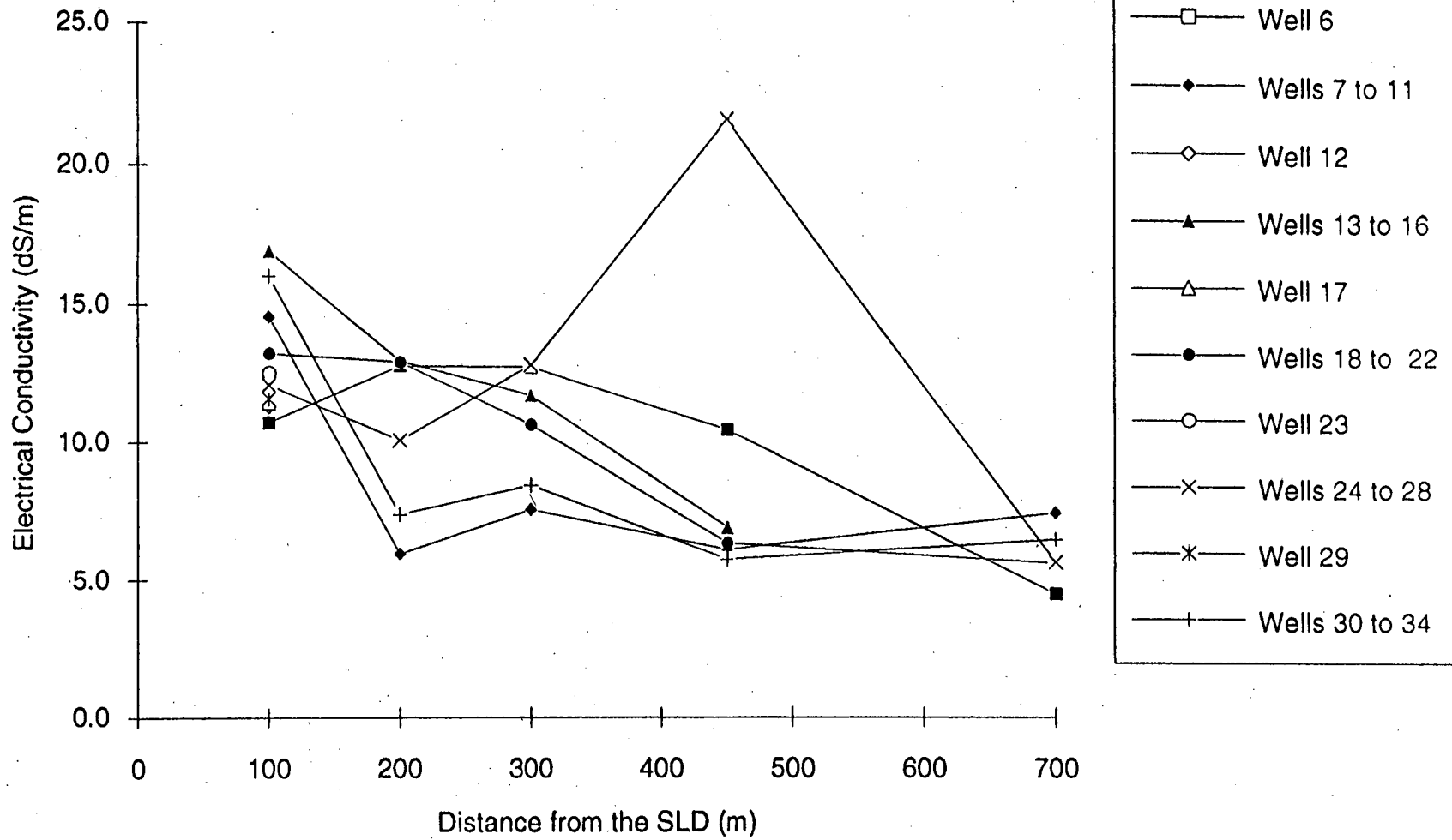
Figure 4.10. Electrical conductivity of groundwater along transects perpendicular to the San Luis Drain for May 1990.
