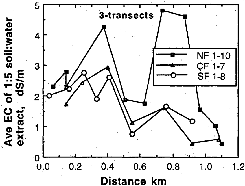
Figure 4.3a. Average electrical conductivities by transect from San Luis Drain outward along transects.
