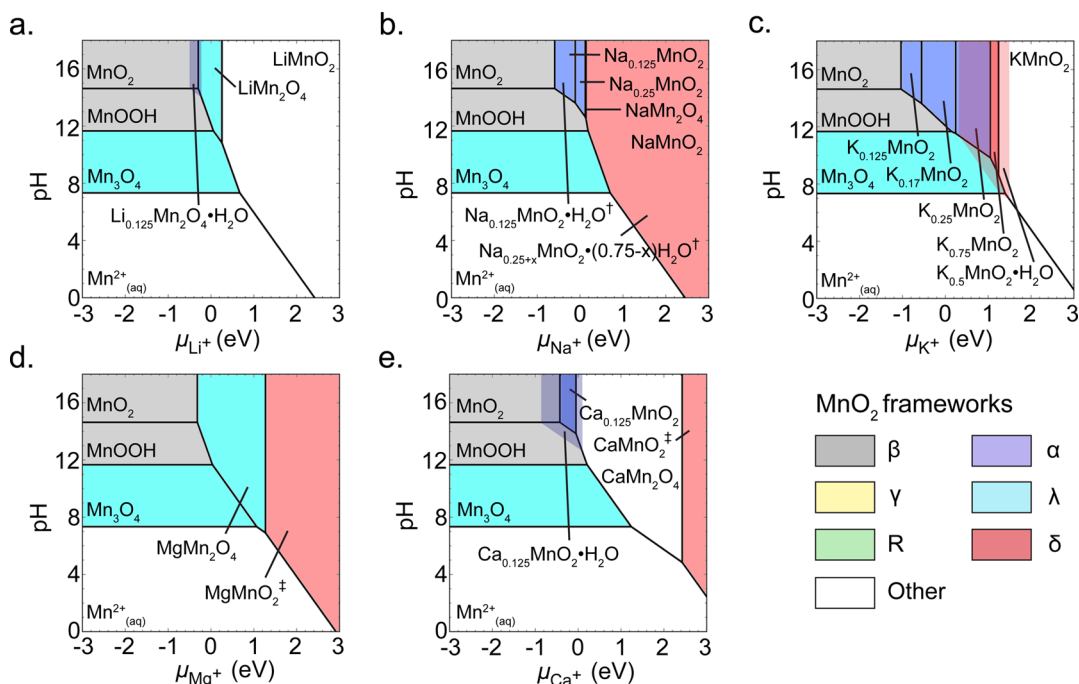
Figure 4. Constrained equilibrium thermodynamics driving phase selection between MnO 2 polymorphs as a function of solution conditions at 298 K and zero applied potential, for solutions containing (a) Li + , (b) Na + , (c) K + , (d) Mg 2+ , or (e) Ca 2+ cations. The zero of the alkali-ion chemical potential corresponds to the chemical potential of the ion in an aqueous solution at a 1 molal concentration. The bixbyite Mn 2 O 3 phase does not appear here as we find it to be unstable with respect to MnOOH up to 231 °C, in close agreement with TGA experiments 60 and recent DFT results, 55 but in conflict with older results. 61 Hydrated configurations from Figure 2 are included as lightly shaded regions demonstrating the relative stability of hydrated phases but not the precise hydrated composition, which we do not resolve in this study. The set of reactions considered in these phase diagrams are available in the Supporting Information. In particular, we do not include the A x MnO 2+y manganate phases which would appear under oxidizing conditions as they fall outside the scope of our analysis, or the alkali oxides and hydroxides which would appear at high alkali potential. †The hydrated α and δ regions align almost exactly with the nonhydrated regions and are not shown for clarity. ‡The AMnO 2 phases for A = Mg, Ca favor the δ phase among the MnO 2 frameworks considered here, but are unstable with respect to phase separation into MnO and AO rocksalts.
