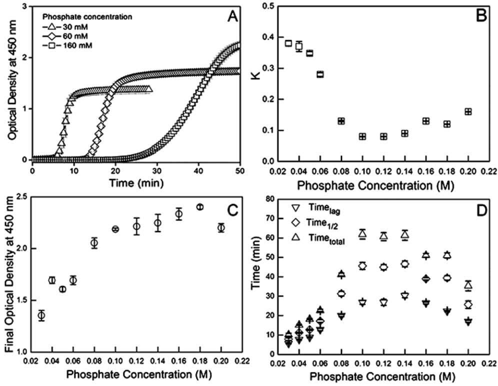
Figure 2.1 The effect of different concentrations of phosphate on turbidity and kinetic parameters during collagen self-assembly into a 2 \text{ g l}^{-1} hydrogel at pH 7.4, 37^\circ\text{C} . (A) Typical turbidity–time curves and corresponding standard deviations of the mean during collagen self-assembly. (B) The rate constants ( K , in units of \text{min}^{-1} ) of collagen self-assembly evaluated by fitting the slopes of turbidity curves like those shown in (A). (C) The observed final optical densities as a function of final phosphate concentration and corresponding standard deviations from the mean. (D) The times to the beginning ( \text{Time}_{\text{lag}} ), middle ( \text{Time}_{1/2} ) and completion ( \text{Time}_{\text{total}} ) of collagen self-assembly and corresponding standard deviations from the mean.
