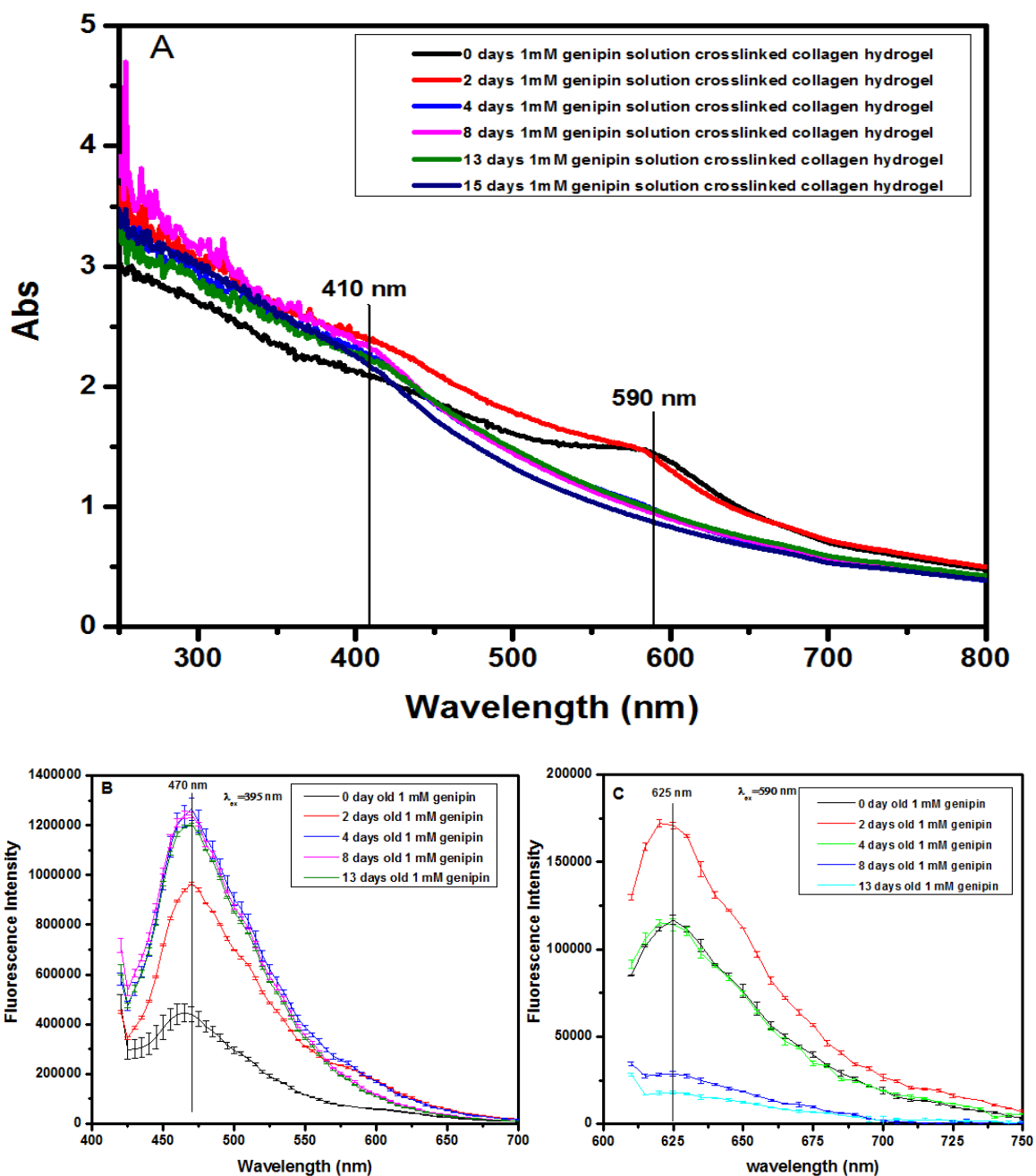
Figure 5.4 The absorption and emission spectra of different “aged” genipin crosslinked collagen hydrogel (A) The absorbance spectra of reaction products between a 2 g/l collagen hydrogel and 1 mM genipin solutions of different ages. (B) Emission spectrum of GCC gel excited with 395 nm wavelength. (B) Emission spectrum of GCC gel excited with 590 nm wavelength. The cross-linking reaction was carried out for 24 hours.
