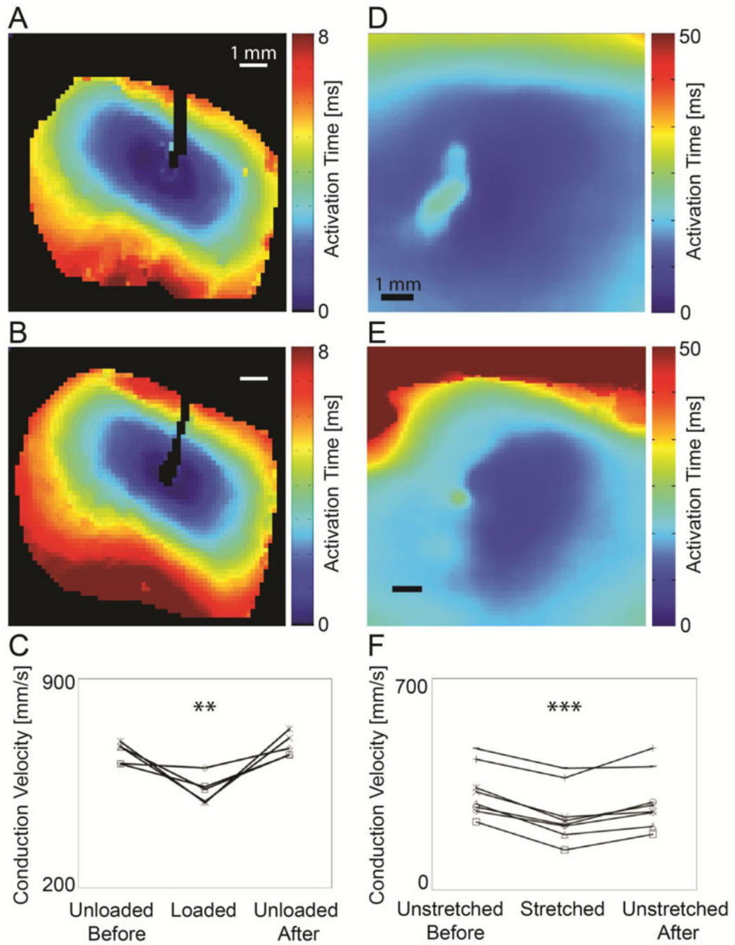
Figure 1. Effects of stretch on conduction velocity measured by fluorescence optical mapping in isolated hearts (A–C) and in micropatterned cardiomyocytes (D–F). Isochronal maps from the epicardium of an isolated WT mouse heart before (A) and after (B) ventricular pressure loading and from micropatterned neonatal ventricular myocyte cultures before (D) and after (E) anisotropic stretch show prolongation of activation times indicating conduction slowing during mechanical loading (scale 1 mm). Maximal epicardial conduction velocity ( CV_{max} ) in isolated mouse hearts (C) decreased significantly and reversibly during loading (N=5,
