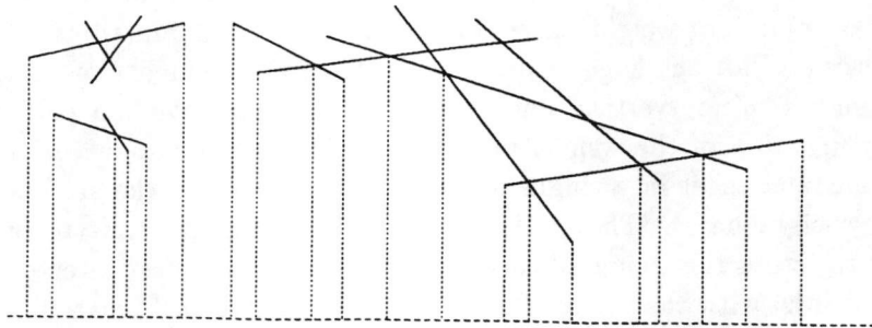
Figure 2. The lower envelope of line segments.
