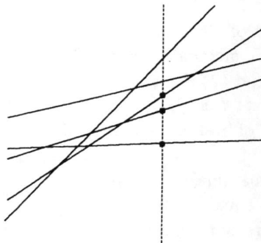
Figure 1. Minimum weight base in a uniform matroid with positive-slope weight functions.
