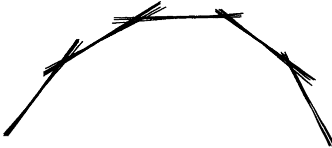
Figure 4. Combining several flattened line arrangements into a single convex chain.
