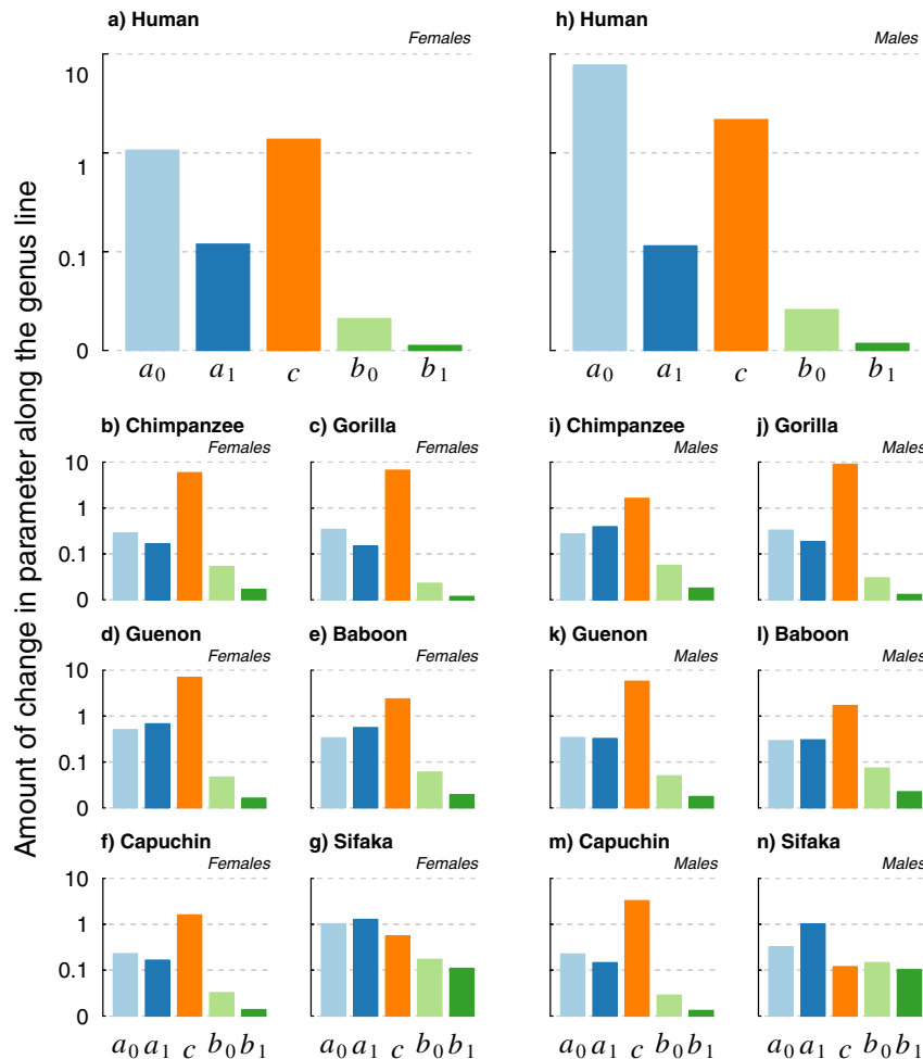
Fig. 3 Relative magnitude of change of each parameter along the genus lines. Pre-adult and age-independent mortality parameters ( a_0 , a_1 , and c ) vary several orders of magnitude more, within each genus, than the ageing parameters ( b_0 and b_1 ). Colours: a_0 (light blue), a_1 (dark blue), c (orange), b_0 (light green) and b_1 (dark green). Values were calculated by numerically solving the path integral in Eq. (9) (see ‘Material and Methods’) for each parameter along each genus line. The y-axes were scaled by the logarithm base 10 to improve interpretability. a–g depict results for females, and h–n for males (Source data are provided as a Source Data File and available in Supplementary Table 4).
