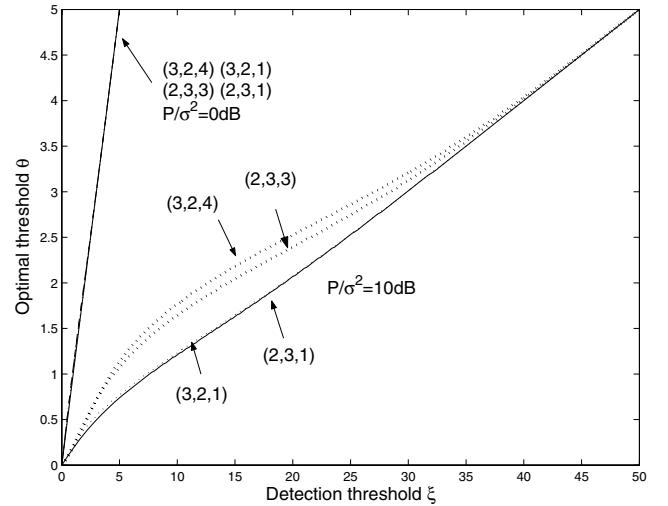
Fig. 9. Optimal \theta versus \xi for \frac{P}{\sigma^2} = 0dB and \frac{P}{\sigma^2} = 10dB under (p, q, n) = (2, 3, 1), (2, 3, 3), (3, 2, 1), (3, 2, 4) .
