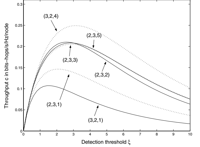
Fig. 5. Throughput comparison under \theta = 0 and \frac{P}{\sigma^2} = 10dB .
