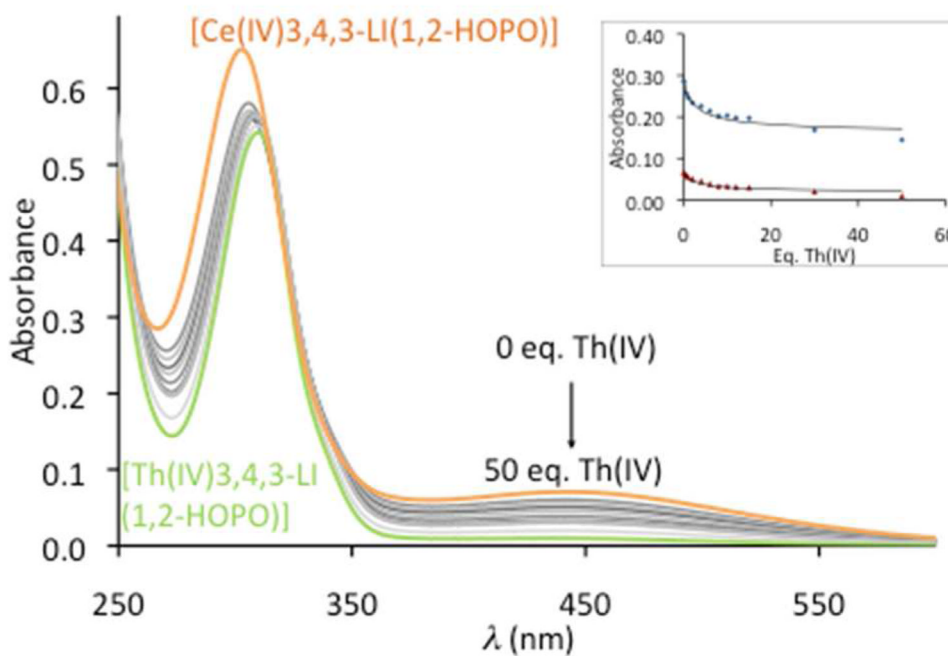
Figure 6. Metal competition batch titration of [\text{Ce(IV)}(3,4,3\text{-LI}(1,2\text{-HOPO}))] with \text{Th(IV)} . [\text{Ce(IV)}] = [3,4,3\text{(LI-1,2-HOPO)}] = 30 \mu\text{M} , [\text{Th(IV)}]:[\text{Ce(IV)}] = 0 to 50 , [\text{H}_2\text{SO}_4] = 0.05 \text{ M} , \text{pH } 1.0 , I = 0.15 ( \text{Na}_2\text{SO}_4 ), T = 20^\circ\text{C} . Inlet: Change of absorbance at 272 \text{ nm} (squares) and 450 \text{ nm} (triangles) versus equivalents of \text{Th(IV)} with the corresponding HypSpec fits (solid lines).
