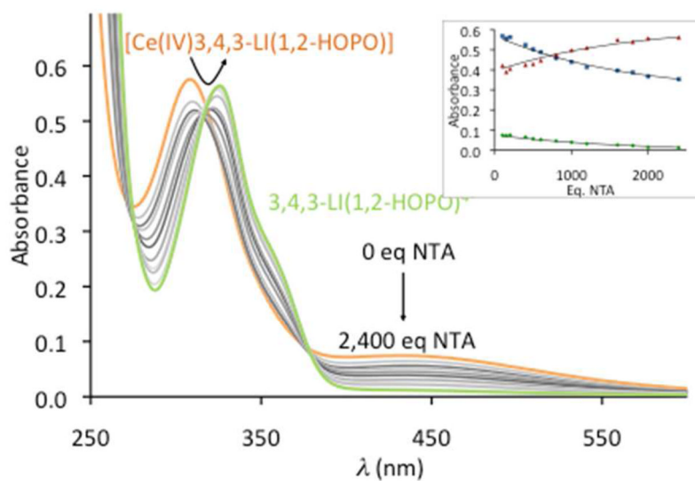
Figure 4. Ligand competition batch titration for the complexation of Ce(IV). [Ce(IV)] = [3,4,3LI-1,2-HOPO] = 30 \mu M , [NTA]:[3,4,3-LI(1,2-HOPO)] = 0:1 to 2,400:1 , [CHES] = 10 \text{ mM} , pH 10.0 , I = 0.4 (KCl), T = 20^\circ C . Inlet: Absorbance change at 305 nm (squares), 327 nm (triangles) and 450 nm (diamonds) versus equivalents of NTA with the corresponding HypSpec fits (solid lines).
