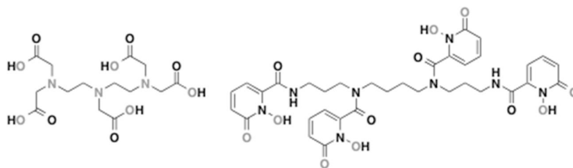
Figure 1. Structures of the ligands discussed in this study: diethylenetriaminepentaacetic acid (DTPA, left) and 3,4,3-LI(1,2-HOPO) (right); metal-coordinating atoms are highlighted in grey.
