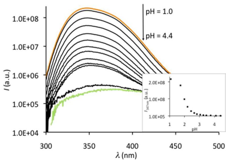
Figure 2. Direct batch spectrofluorimetric titration of [\text{Ce(III)(3,4,3-LI(1,2-HOPO))}]^- in water. [\text{Ce(III)}] = [\text{3,4,3-LI-1,2-HOPO}] = 20 \mu\text{M} , \lambda_{exc} = 252 \text{ nm} , I = 0.1 (KCl), T = 20^\circ\text{C} . Inlet: Fluorescence intensity loss at emission maximum ( \lambda_{em} = 347 \text{ nm} ) showing complex formation upon increasing pH.
