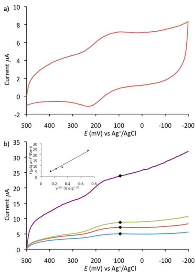
Figure 5. Cyclic Voltammograms for 0.5 mM 3,4,3-LI(1,2-HOPO) cerium complex in 1 M \text{SO}_4^{2-} at pH 8.5 a) with a scan rate of 50 \text{ mV}\cdot\text{s}^{-1} . b) voltammograms of the cathodic site (reduction wave) at different scan rates ( 20 \text{ mV}\cdot\text{s}^{-1} blue, 50 \text{ mV}\cdot\text{s}^{-1} red, 100 \text{ mV}\cdot\text{s}^{-1} green, 500 \text{ mV}\cdot\text{s}^{-1} violet). inlet) linear dependence of the current intensity at 95 mV vs. the square root of the scan rate, suggesting a diffusion controlled process.
