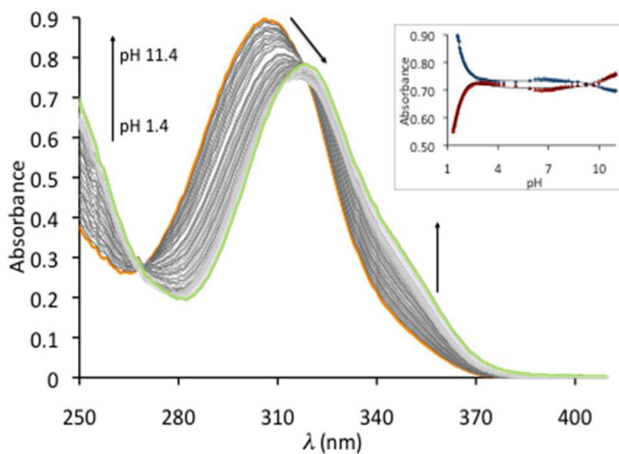
Figure 3. Incremental spectrophotometric titration of [\text{Ce}(\text{III})(3,4,3\text{-LI}(1,2\text{-HOPO}))]^- ( 50 \mu\text{M} ) by KOH in water. I = 0.1 (KCl), T = 20^\circ\text{C} . Inlet: Absorbance change at 305 nm (diamonds) and 327 nm (triangles) versus pH with the corresponding fits (solid lines) from HypSpec.
