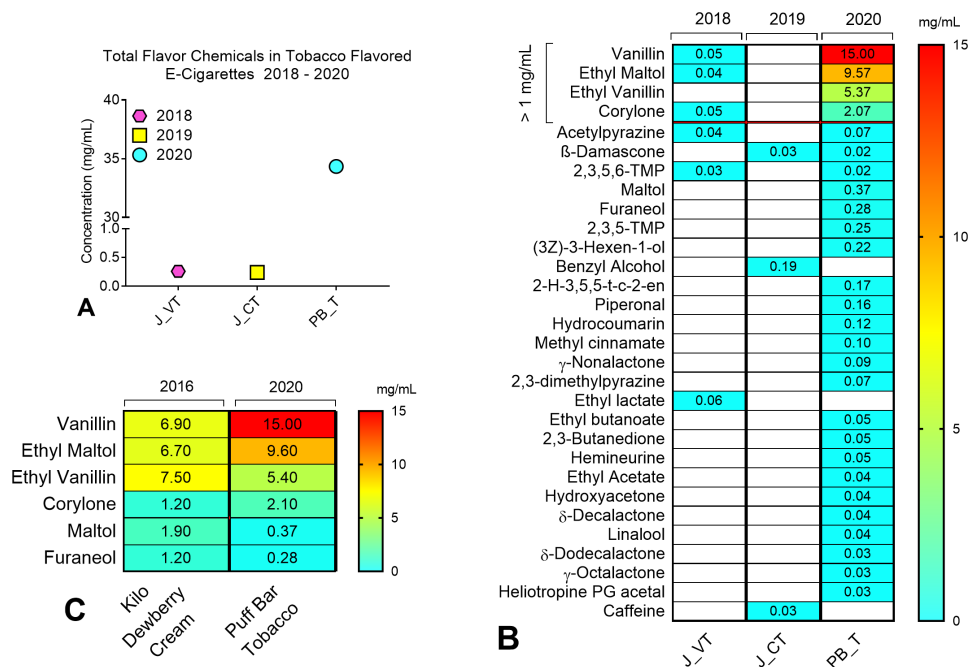
Figure 5 The total flavour chemical concentrations and individual chemicals in JUUL and Puff products. (A) Total flavour chemical concentrations in JUUL and Puff e-cigarettes. (B) Concentrations of individual flavour chemicals in JUUL and Puff e-cigarettes. (C) Dominant flavour chemicals in Kilo Dewberry Cream and Puff Bar Tobacco. The y-axis shows concentrations in mg/mL, and codes represent the products as described in online supplemental table S1. 2-H-3,5,5-t-c-2-en, 2-Hydroxy-3,5,5-trimethyl-cyclohex-2-en; e-cigarettes, electronic cigarettes; TMP, trimethylpyrazine.
