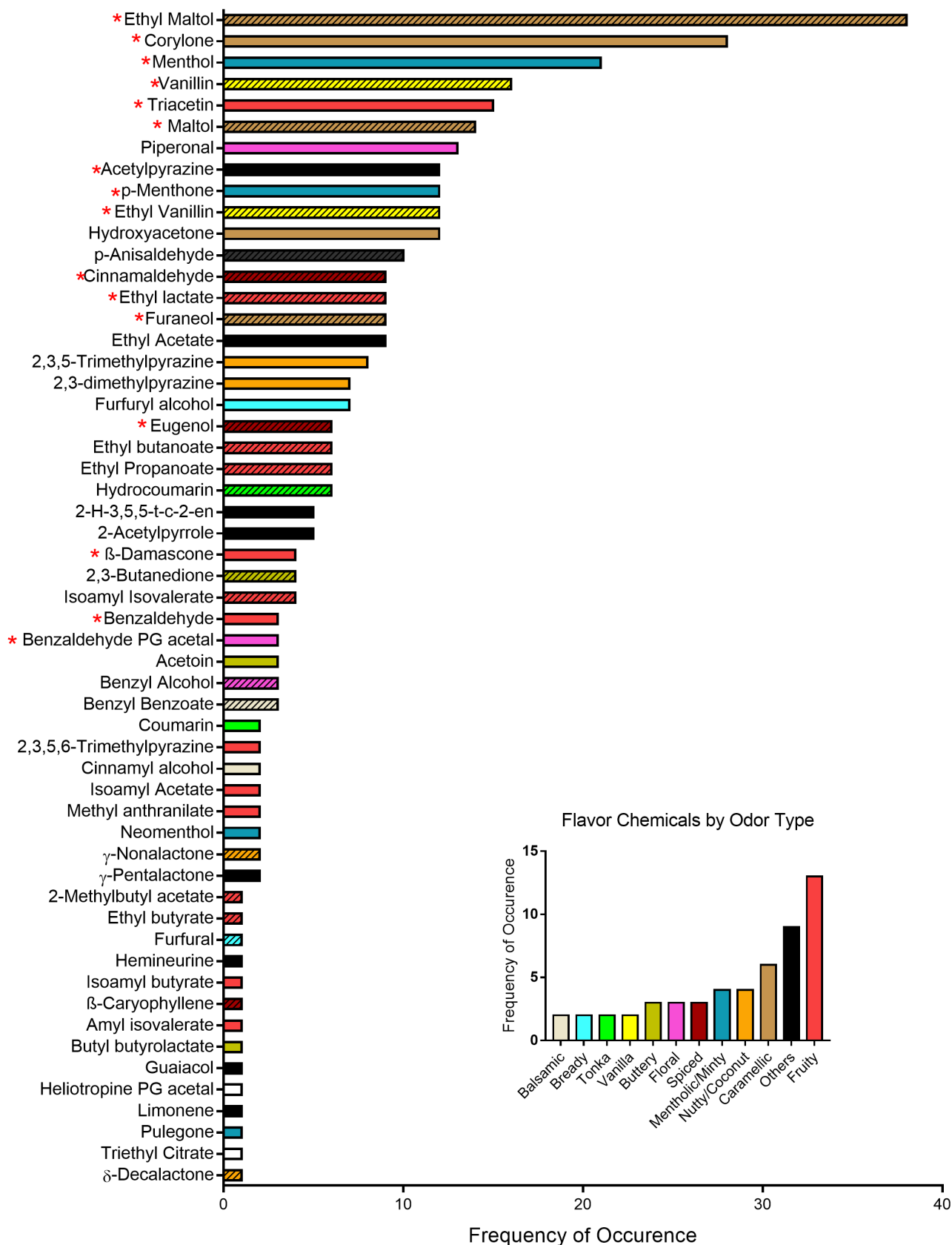
Figure 4 Frequency distribution for 55 flavour chemicals found in 63 tobacco-flavoured refill fluids. The x-axis is the number of products, and the y-axis is sorted according to decreasing frequency of their occurrence. Representative colour codes based on odour type are shown in the insert. Frequency ranged from 1 to 38, with the highest being ethyl maltol. The asterisks indicated chemicals found at >1 mg/mL in at least one product, and hatched bars indicate flavour chemicals that produce a sweet taste. 2-H-3,5,5-t-c-2-en, 2-Hydroxy-3,5,5-trimethyl-cyclohex-2-en.
