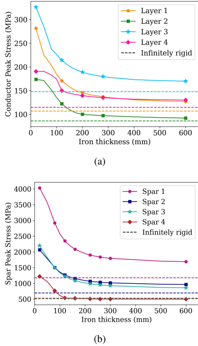
Fig. 3. Von Mises equivalent stress in the conductors (a) and in the mandrels (b) of the stress managed layers 1-4 as a function of the iron thickness variation. The dashed lines represent the results evaluated with an infinitely rigid structure.
