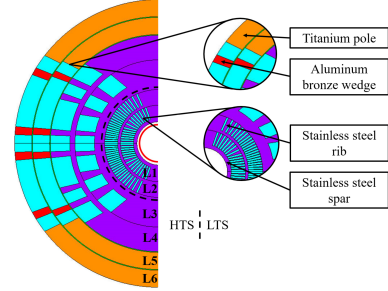
Fig. 1. 2D cross-section of the dipole. The black dashed line separates the HTS from LTS parts. The red line represents the magnet aperture. On the right, the magnified portions of the dipole show the mandrel components (spar and rib) and the parts of the traditional \cos\theta design (pole and wedge).
