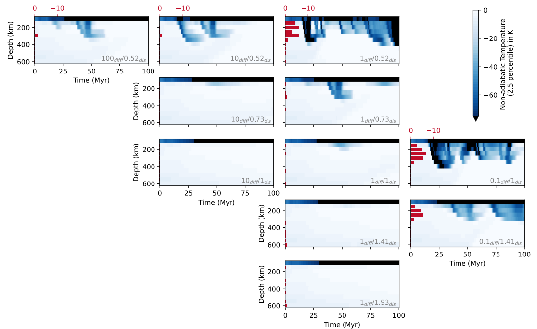
Figure 8. 2.5 percentile of the temperature anomaly (compared to the adiabat with T_p = 1623 K) in ridge-parallel ( y ) direction at a plate age of 42 Ma, plotted in dependence of time and depth for all models. Blue streaks sloping downward indicate cold downwellings from the base of the plate. Temperature anomalies below -75 K are shown in black. Red horizontal bars indicate the mean temperature anomaly in K averaged over the whole model evolution time for each depth range below 100 km. Panels are arranged as in Figure 2.
