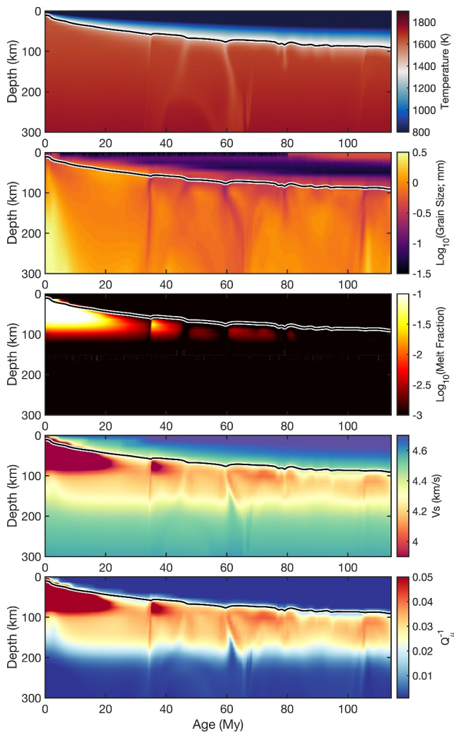
Figure 3. Vertical cross-sections through model 7 ( l_{\text{diff}}/0.52_{\text{disl}} ) at model time of 80 My and associated seismic properties calculated at 65 s period assuming 100 ppm \text{H}_2\text{O} + 100 ppm \text{CO}_2 . Physical properties temperature and grain size are output from ASPECT. Melt fraction is calculated in post-processing using a hydrous equilibrium melting model (Blatter et al., 2022). Shear velocity ( V_S ) and attenuation ( Q_\mu^{-1} ) are calculated using the VBRc (Havlin et al., 2021) and Perple_X (Connolly, 2005; Connolly & Kerrick, 1987). The black contour in each panel marks the 1150°C isotherm, temperatures below which are assumed to represent dehydrated mantle.
