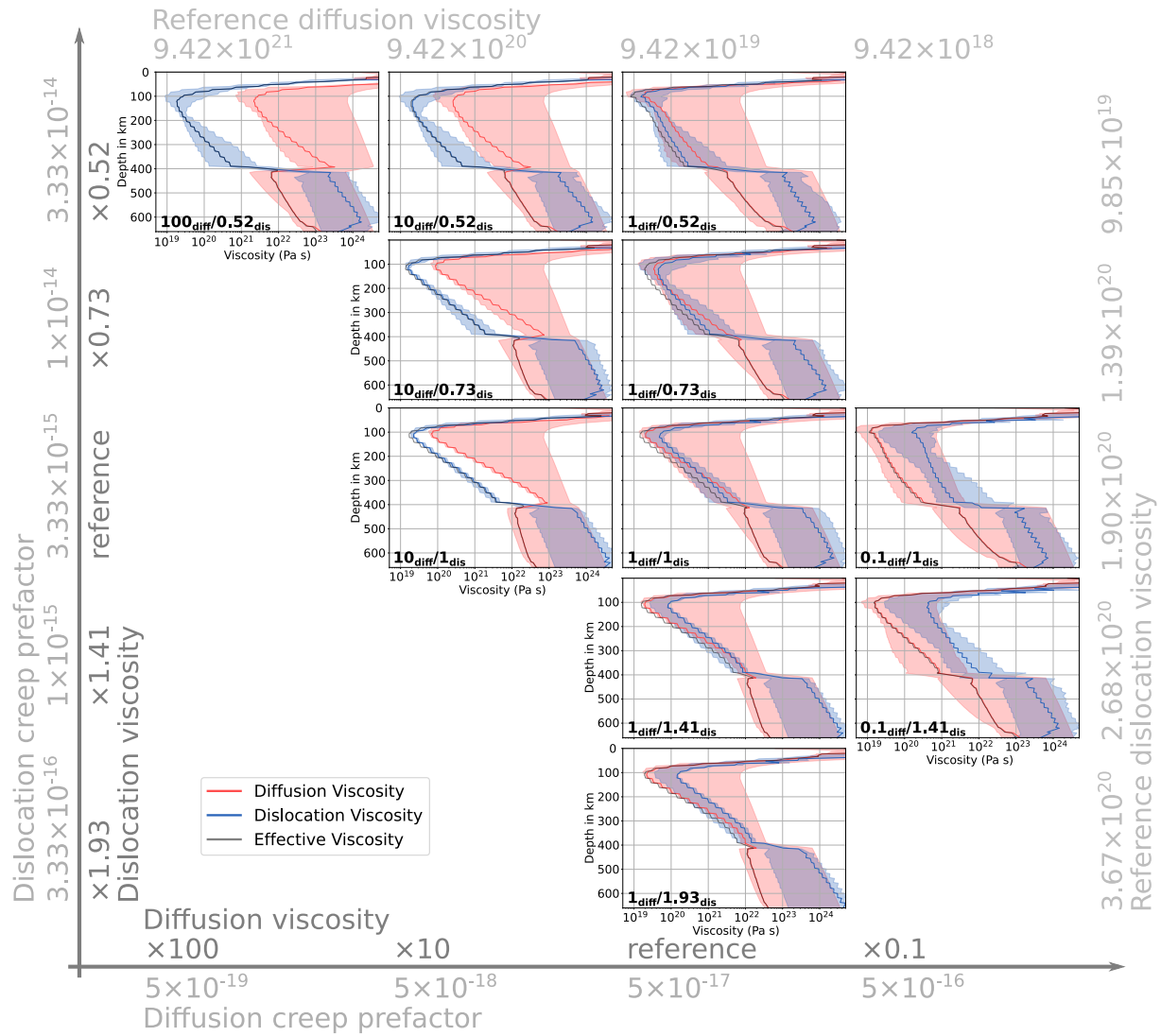
Figure 2. Viscosity profiles for different models at a distance of 2,940 km from the ridge (42 Ma plate age), averaged (using the log-average) across all values in ridge-parallel ( y ) direction. Solid lines show the temporal average over the whole model time, shaded areas show variations between the minimum and maximum viscosities at different points in time. See Table S2 in Supporting Information S1 for details on how reference viscosities are defined.
