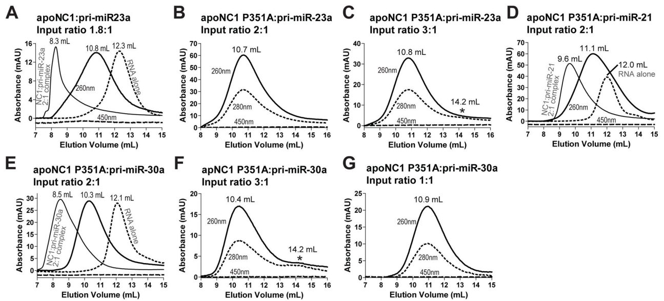
Figure 5. Fe(III) heme causes a large conformational change to DGCR8-pri-miRNA complexes. Size exclusion chromatograms of (A) apoNC1 in complex with 0.45 \mu M pri-miR-23a and (B–G) apoNC1 P351A with 2 \mu M pri-miRNAs at the indicated input ratios. The asterisk in (C) and (F) marks a potential free protein peak.
