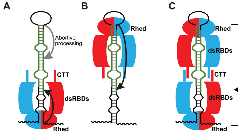
Figure 6. Models of how a pri-miRNA is recognized by the Microprocessor (A) The basal junction anchoring model (Han et al., 2006). (B) The apical junction anchoring model (Zeng et al., 2005). (C) Our proposed molecular clamp model. See Discussion for details. The DGCR8 subunits in a dimer are shown in red and cyan. The thick avocado strands represent 5' and 3' mature miRNAs.
