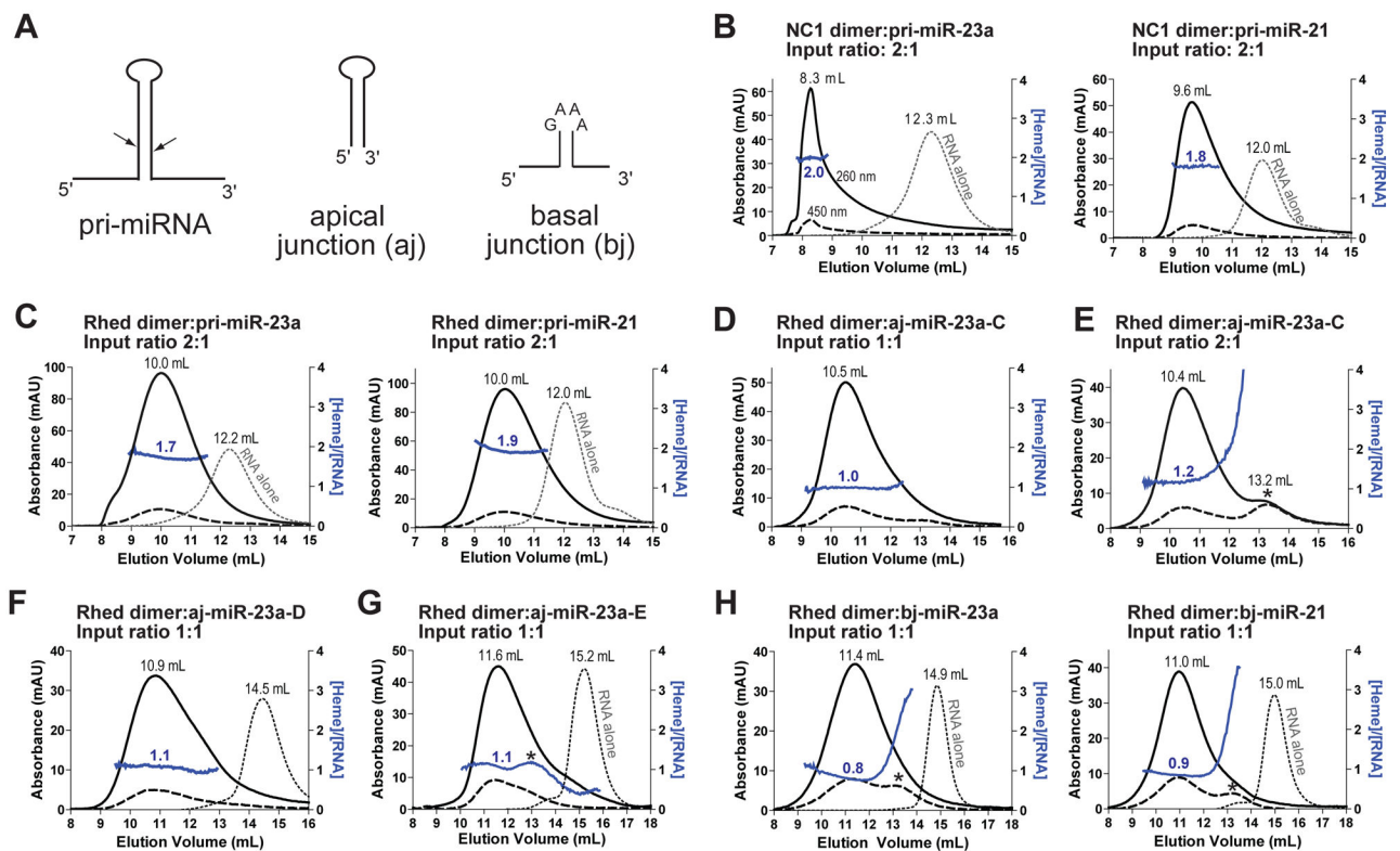
Figure 2. RNA truncation and SEC analyses suggest that the Rhed binds to pri-miRNA junctions (A) Schematics of pri-miRNA fragments. The arrows indicate the Droscha cleavage sites. The sequences and secondary structures are shown in Table S1 and Figures S2 and S3. (B–H) Size exclusion chromatograms of NC1 in complex with 2 \mu M pri-miRNAs (B), the Rhed with 2 \mu M pri-miRNAs (C), the Rhed with 4 \mu M of aj-miR-23a-C at varying input ratios (D–E), the Rhed with 4 \mu M of aj-miR-23a-D (F), the Rhed with 4 \mu M of aj-miR-23a-E (G), and the Rhed with 4 \mu M of indicated basal junctions (H). Solid black lines indicate A_{260} , dashed lines show A_{450} and dotted lines are A_{260} of the RNA-only runs. Solid blue lines represent heme:RNA ratios calculated from A_{450} and A_{260} , following the scale on the right y axis. The asterisk in (E, G, H) marks a peak of free Rhed. See also Figures S1–S4 and Table S1.
