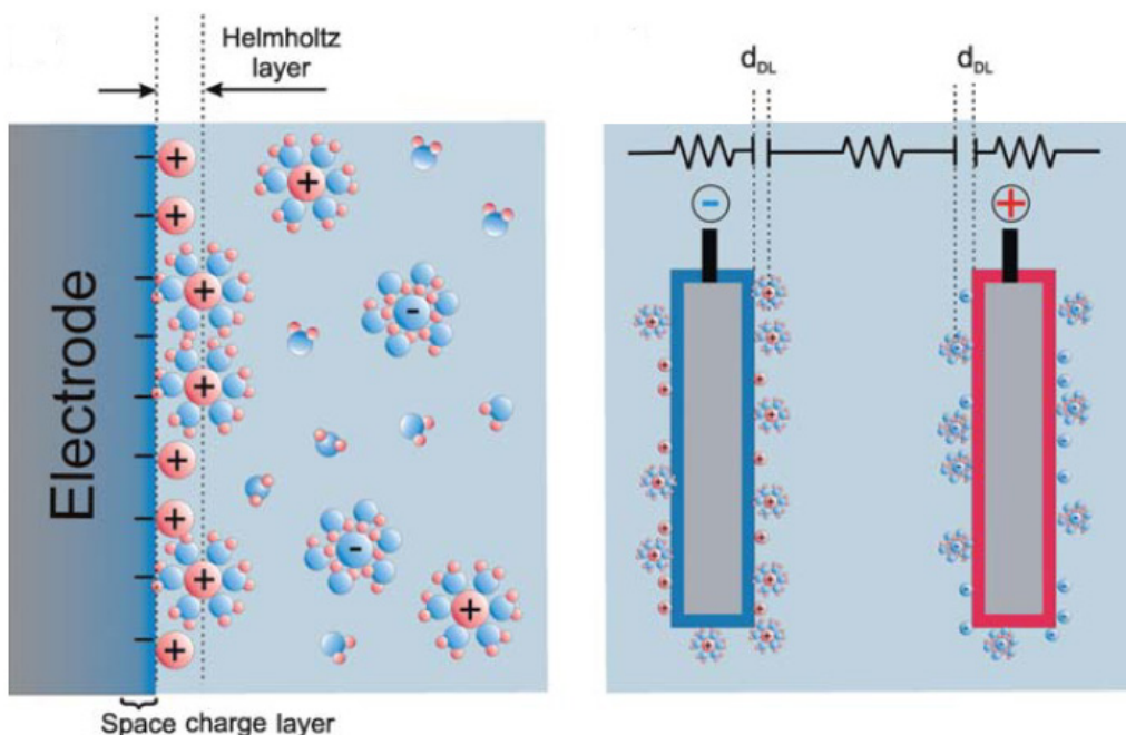
Figure 4.1. Diagram of an electric double layer (left) and the two electrodes of an EDLC (right). Adapted from Biener et al. 1
