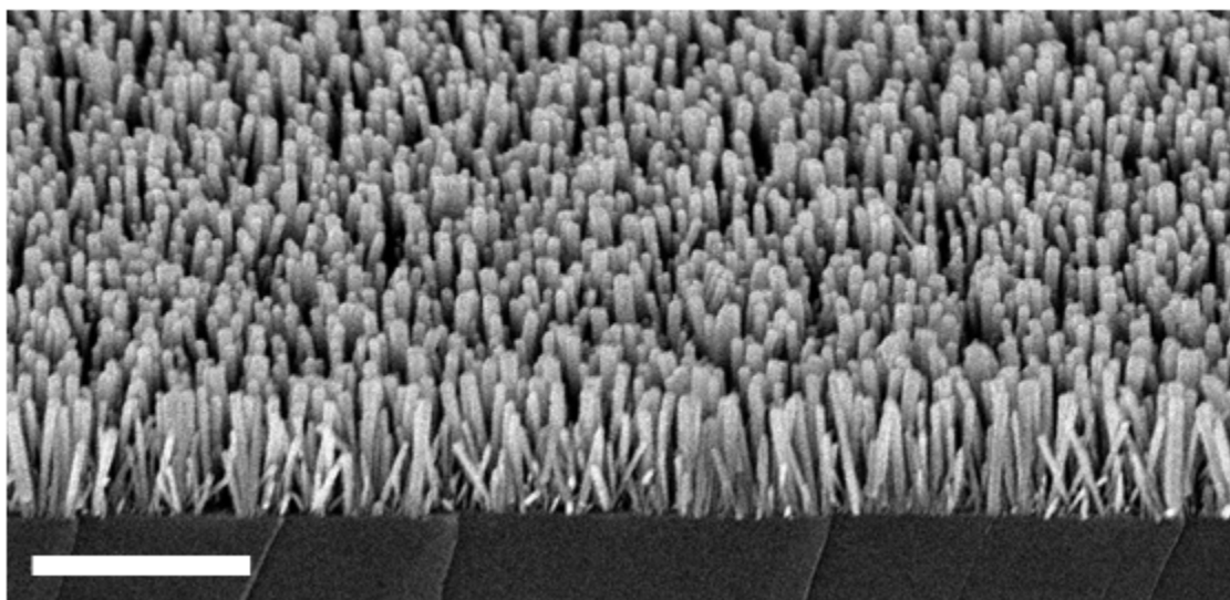
Figure 2.3. Cross-sectional SEM of a hydrothermally grown ZnO nanowire array, tilted to 45°. Scale bar is 1 \mu\text{m} .
