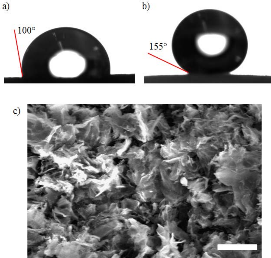
Figure 6.17. Contact angle measurements of a 10 \mu\text{L} droplet on samples of (a) graphene aerogel annealed at 1050 ^{\circ}\text{C} and (b) BN aerogel. (c) SEM of an exposed inner surface of the BN aerogel. Scale bar is 100 \mu\text{m} . Data courtesy of Thang Pham.
