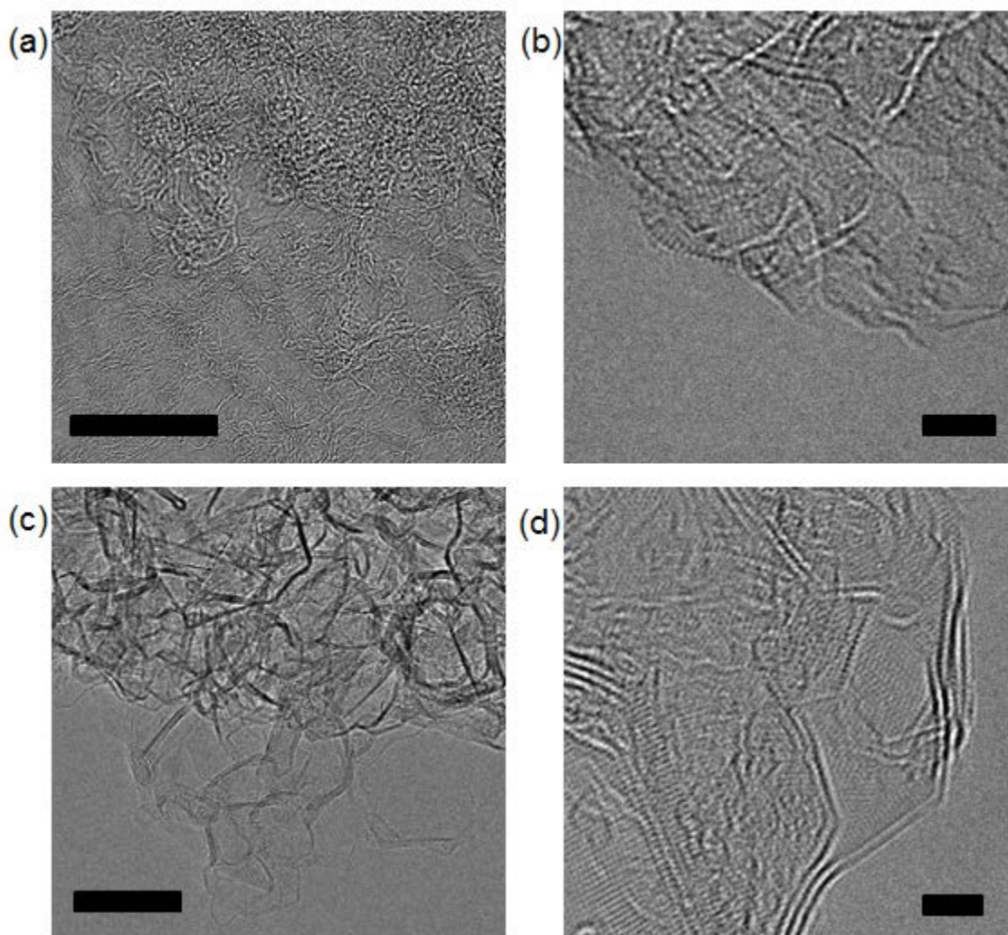
Figure 6.1. TEM images of a GO-based aerogel after annealing at (a, b) 1050 °C and (c, d) 1600 °C. Scale bars are (a, c) 20 nm and (b, d) 2 nm. Data collected with assistance from Peter Ercius.
