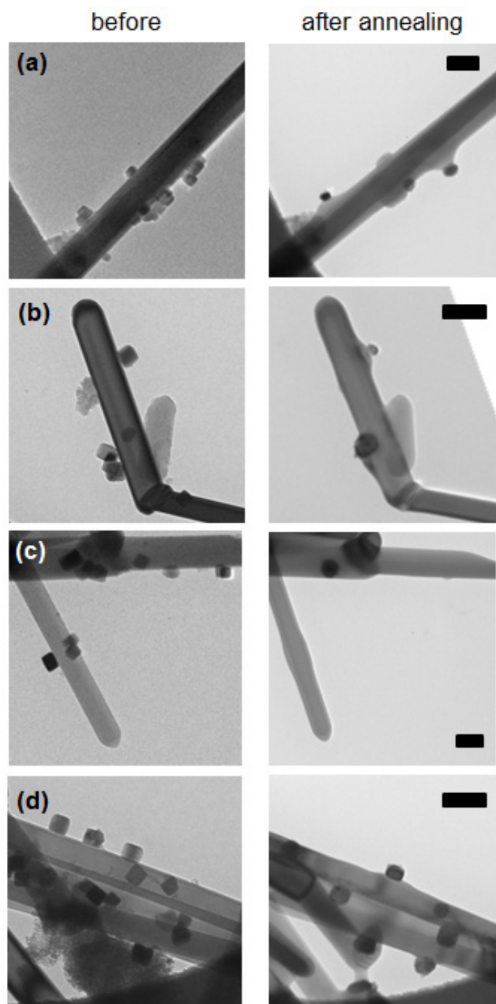
Figure 3.2. Low-resolution TEM of \text{TiO}_2 nanowires coated with \text{Co}_3\text{O}_4 nanoparticles, before and after ex situ heating. The nanoparticle-nanowire interfaces were annealed at 785 °C in Ar for 30 seconds. Scale bars are all 100 nm.
