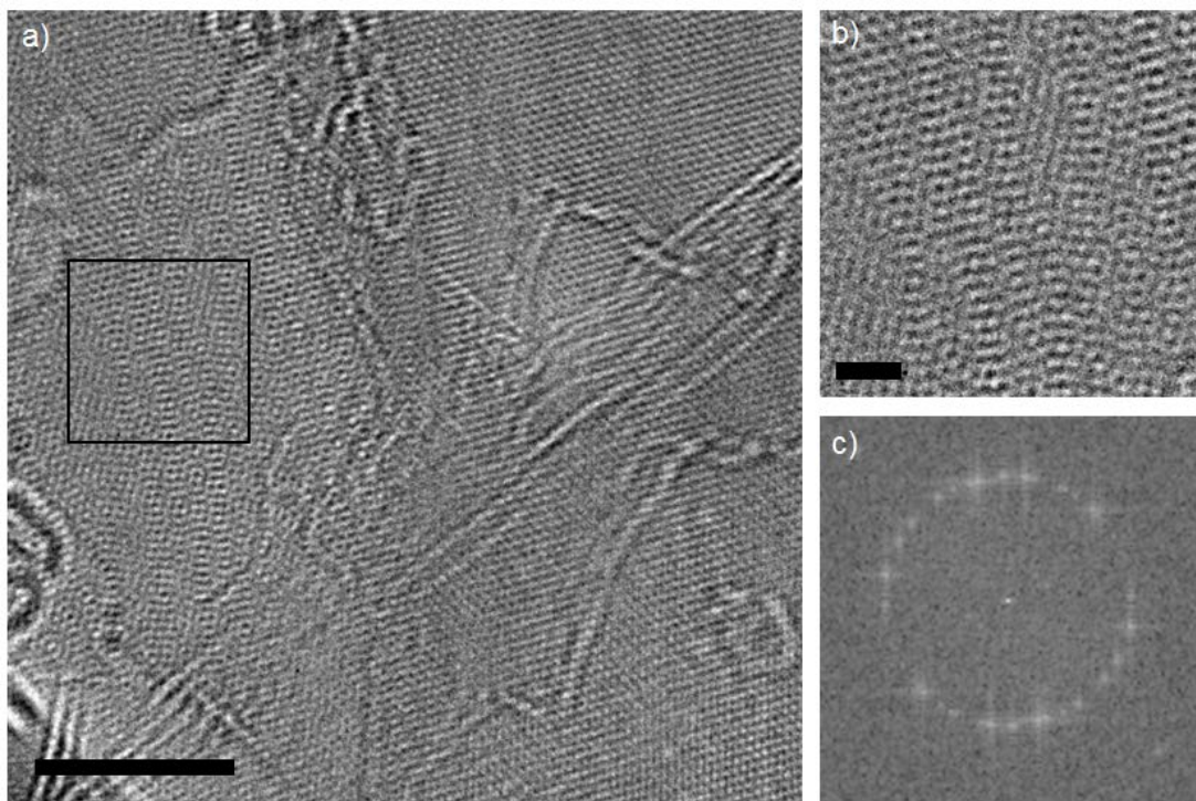
Figure 6.13. (a) TEM of a portion of BN aerogel and (b) a magnified region of the image in part a, showing a portion of BN sheets lying parallel to the imaging plane. (c) FFT of this region with at least 5 overlapping hexagonal spot patterns. Scale bars are (a) 5 nm and (b) 1 nm.
