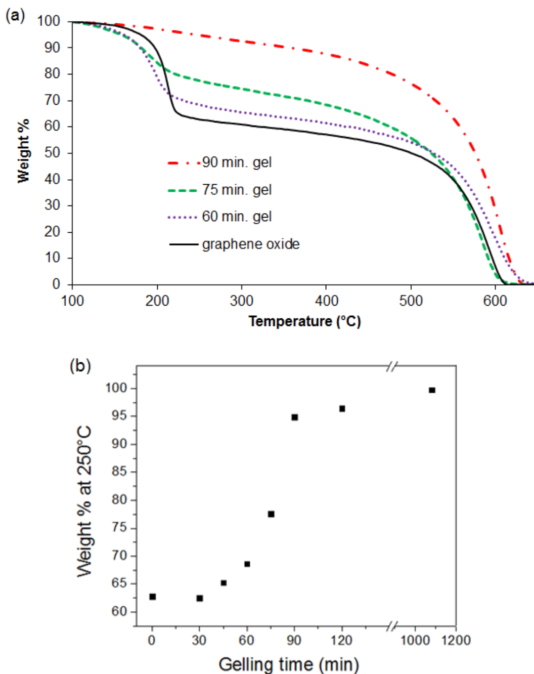
Figure 5.5. (a) TGA data for a series of GO samples exposed to different gelation times. Curves are normalized at 100 °C and baseline subtracted. (b) Extent of mass loss in the lower-temperature portion of the TGA curve, expressed as percent of original mass vs. gelation time.
