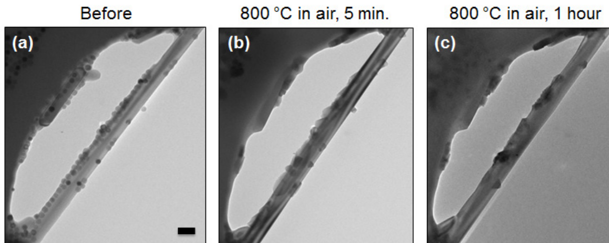
Figure 3.1. MnO particles deposited on TiO 2 nanowires for ex situ heating and imaging by TEM. Particles aggregate and change shape after short annealing times (b) and begin to incorporate into the nanowire during longer anneals (c). Scale bar is 100 nm.
