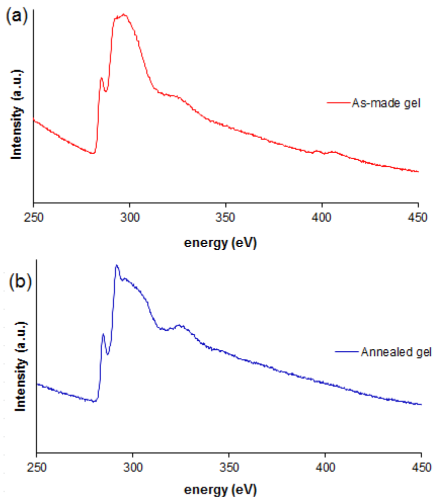
Figure 6.5. C-K edge of the EEL spectrum GO-based aerogels (a) before and (b) after annealing at 1050 °C.
