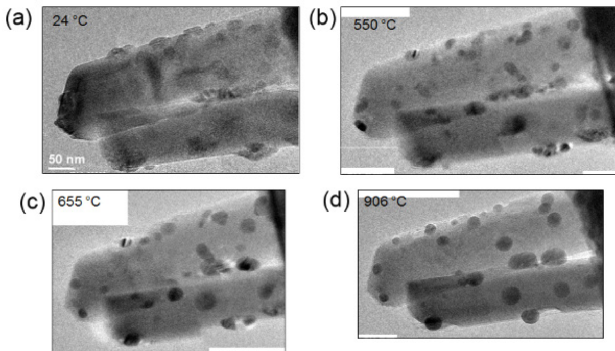
Figure 3.7. An in situ heating experiment on a \text{TiO}_2 nanowire that had been coated in \text{Co}(\text{NO}_3)_2 and then annealed at 350^\circ\text{C} to form particles of \text{Co}_3\text{O}_4 . Temperature of the heating stage increases from (a) through (d). Local temperature at the nanowire may differ from the value measured at the thermocouple.
