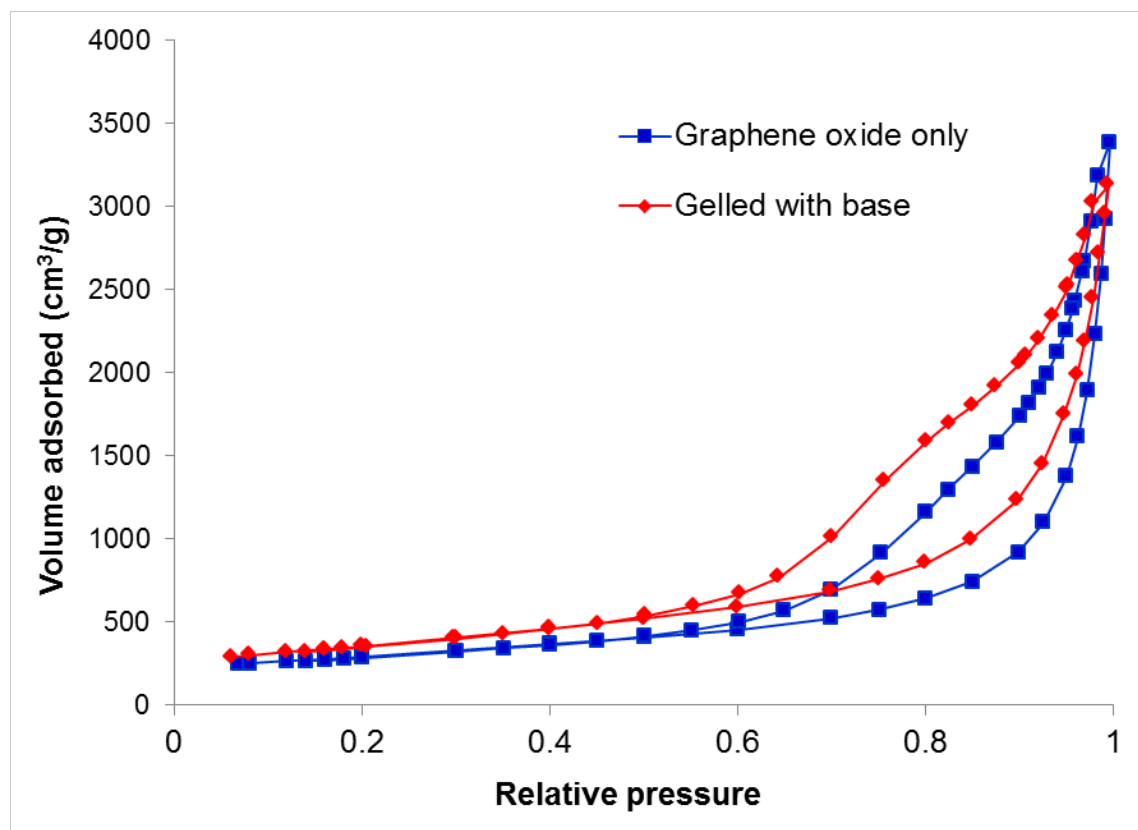
Figure 5.3. Nitrogen adsorption isotherm for two aerogels, formed from GO with \text{NH}_4\text{OH} at 80 °C (red diamonds) and formed from GO with no base at 180 °C (blue squares). Data courtesy of Marcus Worsley and Lawrence Livermore National Laboratory (LLNL).
