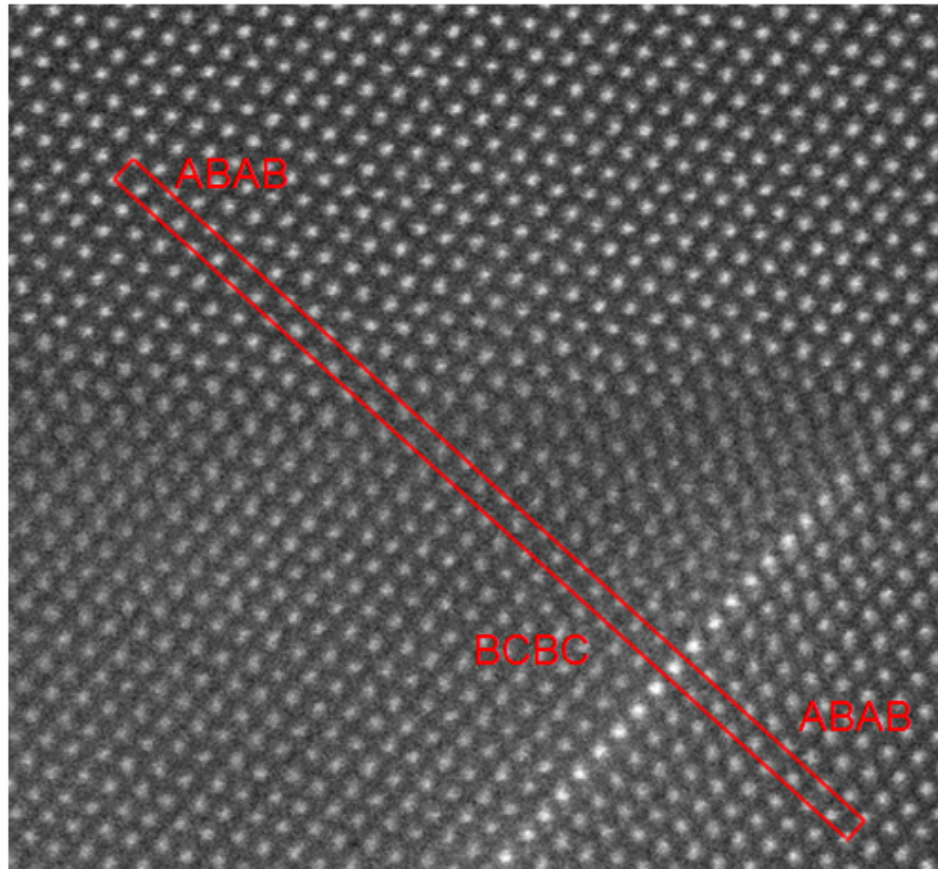
Figure 2.8. Aberration-corrected STEM shows a paired zigzag and basal inclusion, where both layers serve as stacking faults for the ZnO wurtzite lattice. The red lines are intended to guide the eye along a column of atoms that represent the A position.
