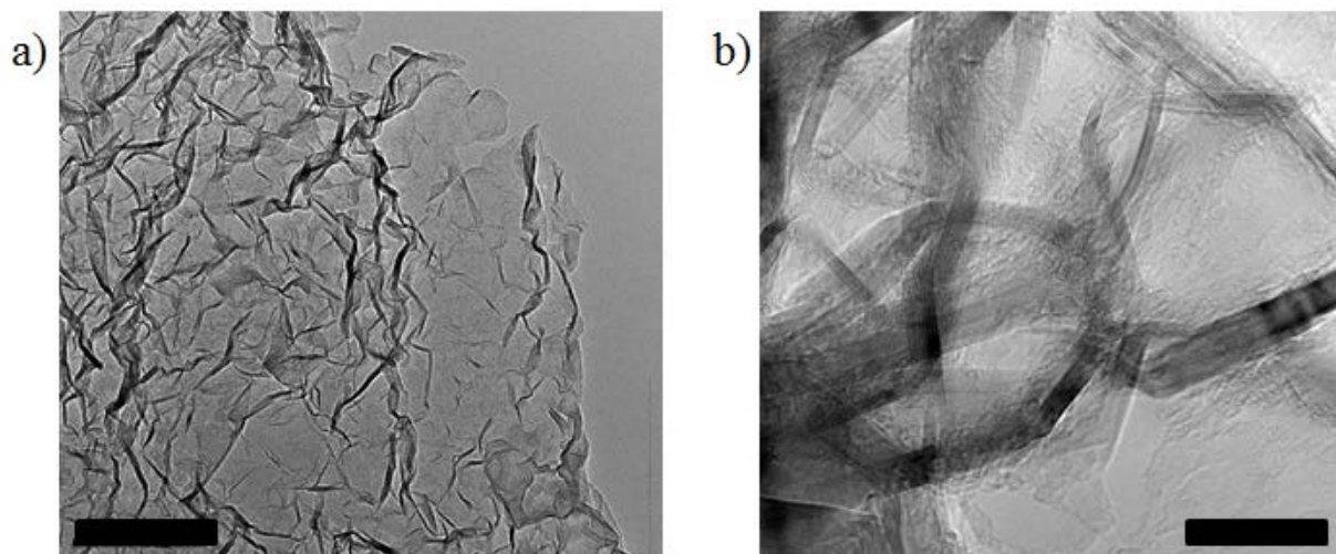
Figure 6.7. Low-magnification TEM of BN aerogel, showing the pores formed by the crystalline BN sheets. Scale bars are (a) 200 nm, and (b) 20 nm. Data courtesy of Thang Pham.
