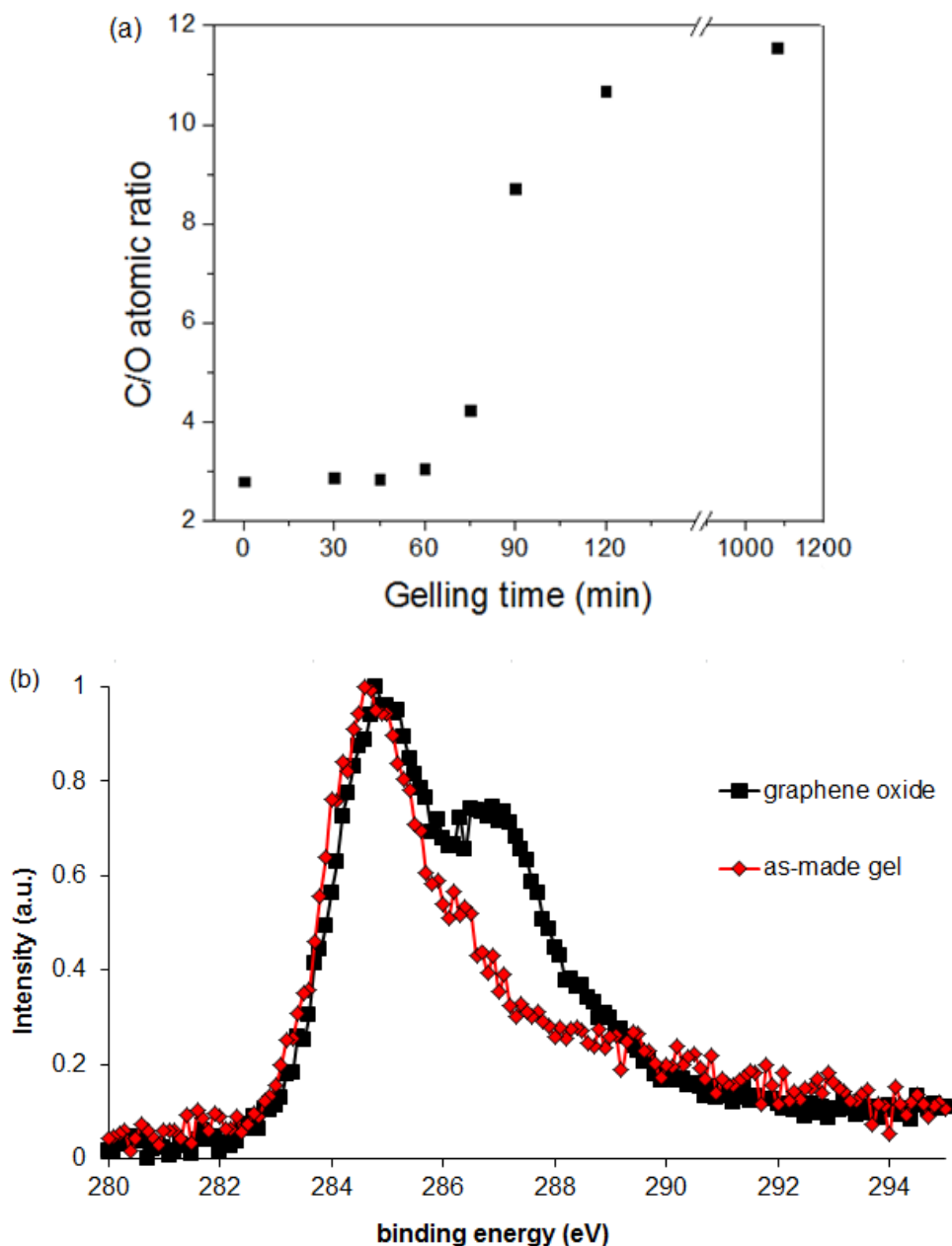
Figure 5.4. (a) Atomic ratios of carbon to oxygen at different gelation times, based on EDS signal. (b) XPS data for GO powder and a fully reacted gel. Spectra are normalized at the maximum signal and baseline subtracted.
