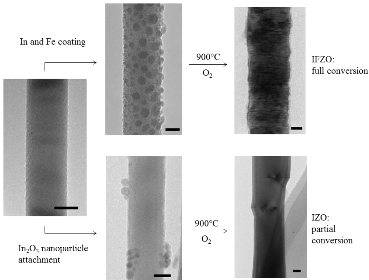
Figure 2.4. Two synthetic methods used to incorporate In and/or Fe into ZnO nanowires are shown, beginning from a VLS-grown ZnO nanowire on the left. Scale bars are 20 nm. The nanowires depicted here by low-resolution TEM are representative of other nanowires from similar samples. For the top path to full IFZO conversion, the sample shown was sputtered with 10 nm of Fe and then thermally evaporated with 10 nm of In, followed by brief exposure to oxygen plasma before annealing. For the bottom path to partially converted IZO, the ZnO array was soaked for two hours in a dilute hexanes solution of In 2 O 3 nanoparticles.
