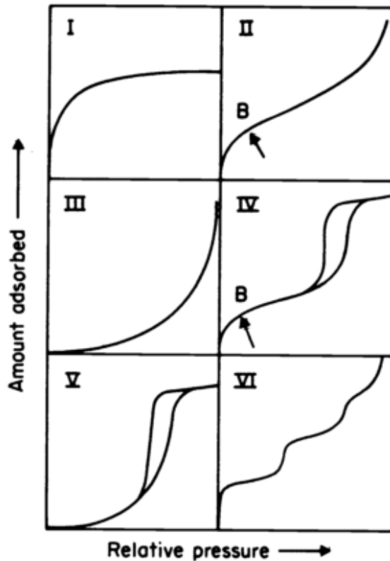
Figure 4.3. Isotherms of Types I-VI that may be obtained from porosimetry measurements. From Sing et al. 7
