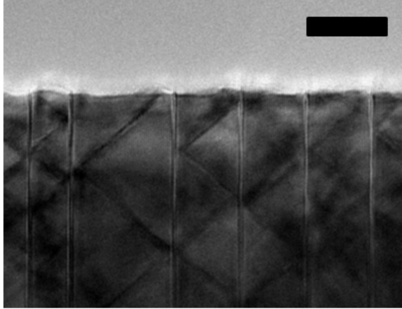
Figure 2.1. TEM image of an IZO nanowire, produced by annealing a ZnO nanowire array coated with In. Two types of inclusions are shown here: basal inclusions are perpendicular to the surface, and zigzags modulate between the basal inclusions. Scale bar is 10 nm.
