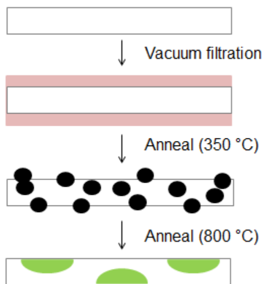
Figure 3.5. A schematic depicting the steps involved in coating a \text{TiO}_2 nanowire with pockets of \text{MTiO}_3 . The nanowires are dispersed in aqueous salt solution, such as \text{Co}(\text{NO}_3)_2 , and vacuum filtered, after which each nanowire is coated in a thin film of solid \text{Co}(\text{NO}_3)_2 (shown in pink above). This film oxidizes when annealed in air to form nanoparticles of \text{Co}_3\text{O}_4 (black). When the nanowire-nanoparticle system is annealed to higher temperatures in Ar, Co diffuses into the nanowire and forms pockets of \text{CoTiO}_3 (green).
