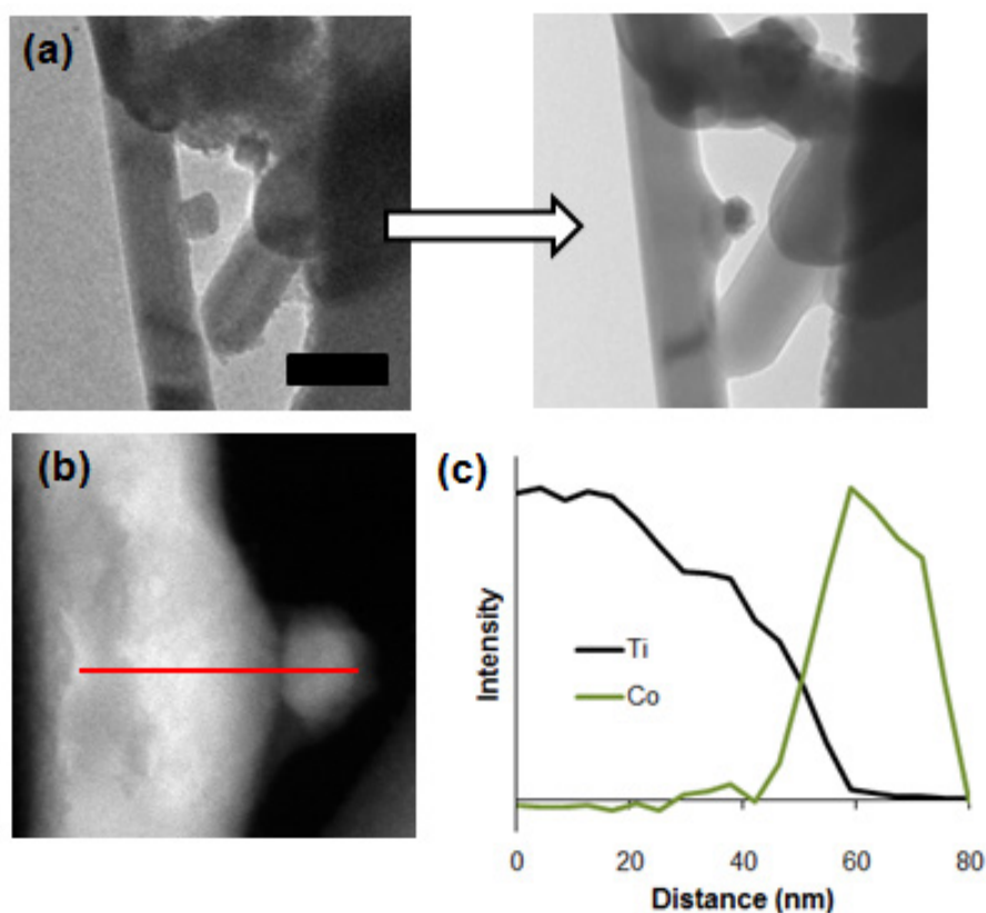
Figure 3.3. (a) Low-resolution TEM of a TiO 2 nanowire interfaced with a cobalt oxide nanoparticle, shown before and after ex situ heating at 785 °C in Ar for 30 seconds. Scale bar 100 nm. (b) The same interface in STEM imaging mode, where the red line indicates the path of the EELS line scan. (c) Results of the EELS line scan, where intensity is the normalized integral of the signal intensity in the region of the Ti L 2,3 region (black line) and the Co L 2,3 region (green line). EELS spectra were background subtracted before integration.
