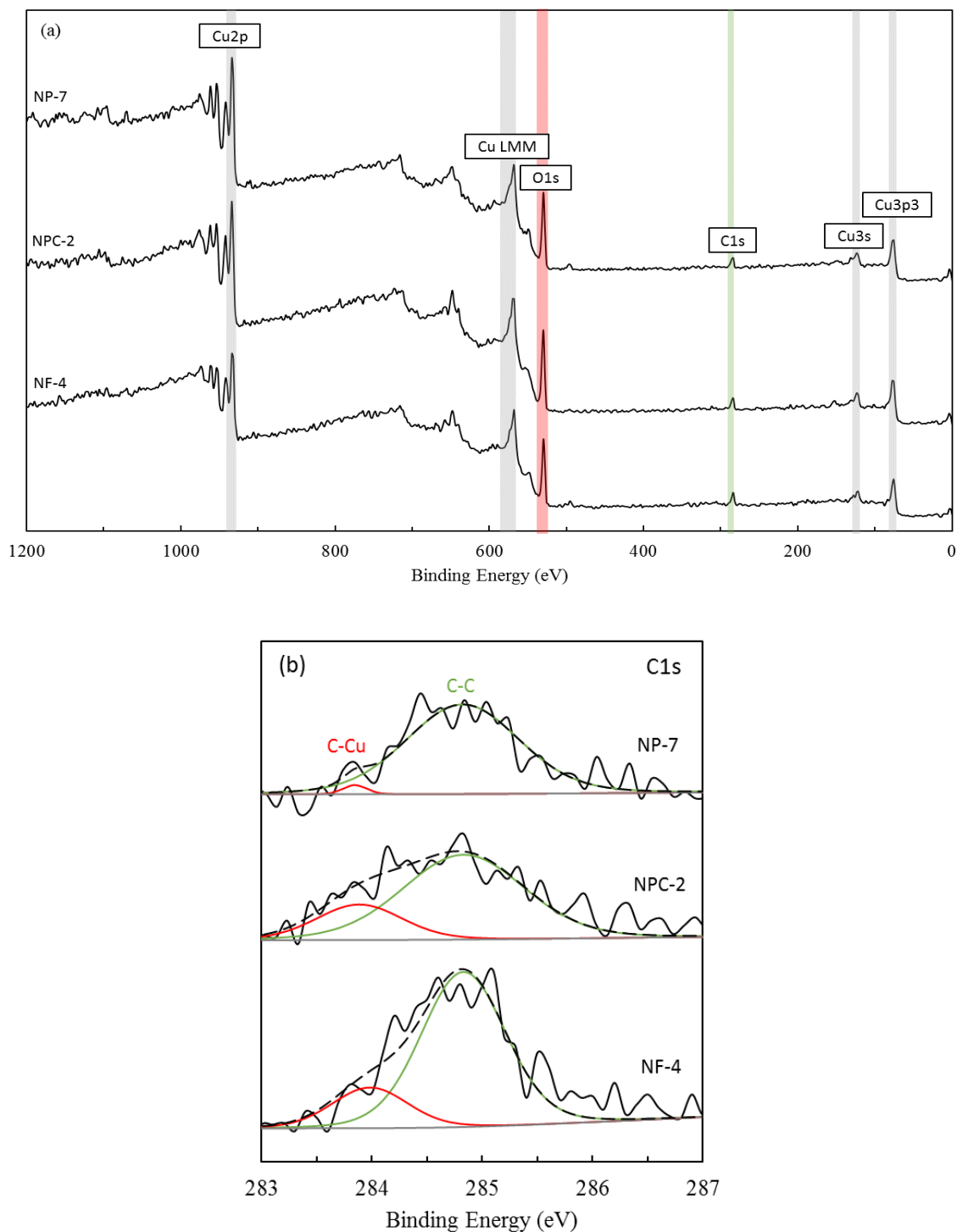
Figure 42. XPS spectrum of CuO nanomaterials (NP-7, NPC-2, and NF-4) prepared via co-precipitation (no polymer), hydrothermal treatment in the presence of PVP (M.W.=1,300,000), and electrospinning, using PVP (M.W.=1,300,000) as a template, respectively. (a) Wide spectra of the copper oxide sorbents, (b) high-resolution spectra of C 1s, with peak fittings corresponding to C-C and C-Cu.
