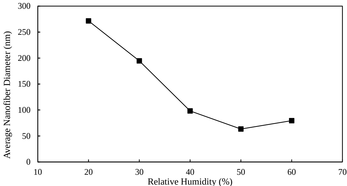
Figure 21. Average diameter of PVP-Cu(NO 3 ) 2 nanofibers at five relative humidity levels (20, 30, 40, 50, and 60 %). Each electrospinning solution was prepared using 1.3 g of PVP, 1.3 g of copper nitrate, 23 cm 3 of ethanol, and 10 cm 3 of DI water. Electrospinning was conducted at 30 kV, 18 inches, and 1.0 cm 3 hr -1 .
