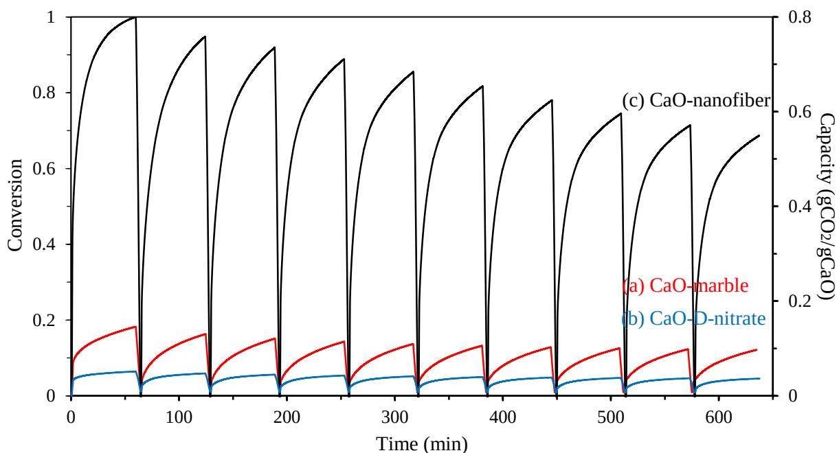
Figure 32. Conversion and capacity for (a, red) CaO-marble, (b, blue) CaO-D-nitrate, and (c, black) CaO-nanofiber over 10 carbonation-calcination cycles at 873 K, 101 kPa, and 200 sccm of CO 2 via thermogravimetric analysis.
