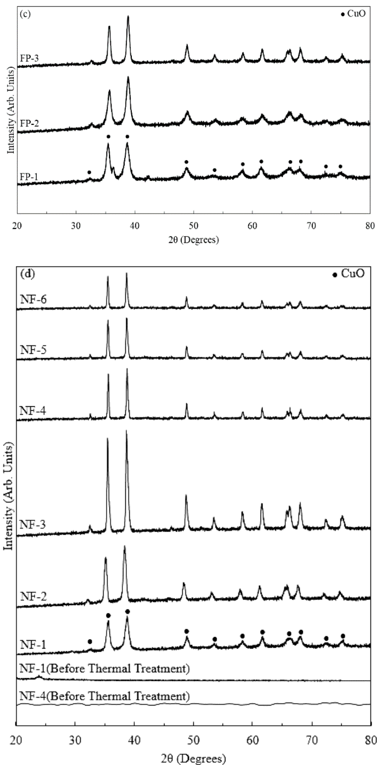
Figure 39. X-ray diffraction patterns of CuO sorbents. (a) nanoparticles via sol-gel, co-precipitation, and hydrothermal treatment (NP and NPC), (b) nanobelts via co-precipitation (NB), (c) flowerlike nanostructures via co-precipitation and hydrolysis (FP), and (d) nanofibers via electrospinning (NF).
