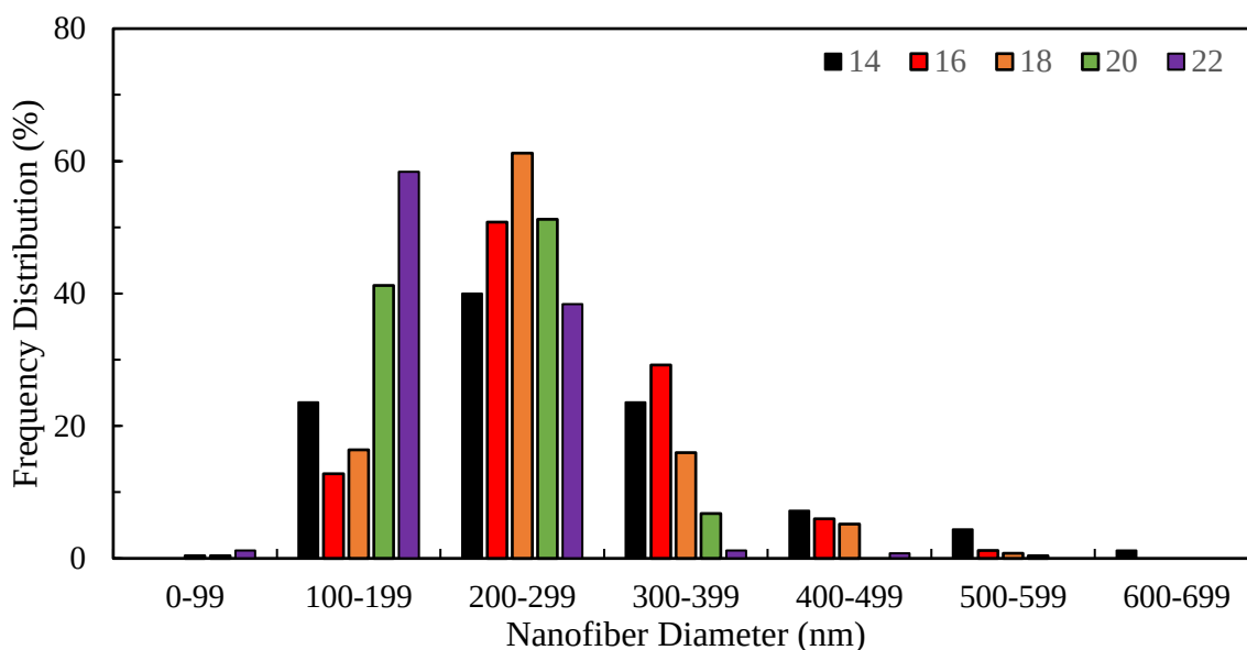
Figure 18. Diameter size distribution of PVP-Cu(NO 3 ) 2 nanofibers prepared at different tip-of -needle to collecting plate distances (14, 16, 18, 20, and 22 inches). Each electrospinning solution was prepared using 1.3 g of PVP, 1.3 g of copper nitrate, 23 cm 3 of ethanol, and 10 cm 3 of DI water. Electrospinning was conducted at 30 kV, 1.0 cm 3 hr -1 , and 20% relative humidity.
