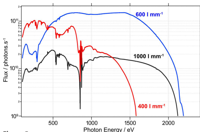
Figure 5 Beamline transmission for the three gratings as measured from a photodiode in ES-2, vertical exit slit opening 9 \mu\text{m} , c_{\text{ff}} 1.4.
