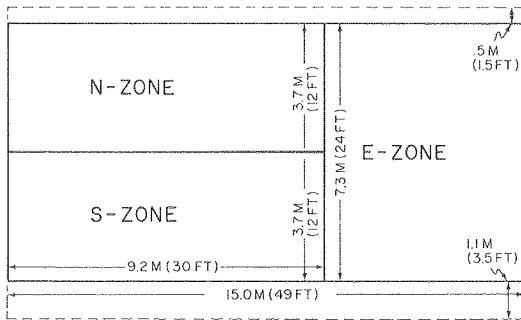
FIG. 2: Floor plan showing thermal zones for blast simulation.
