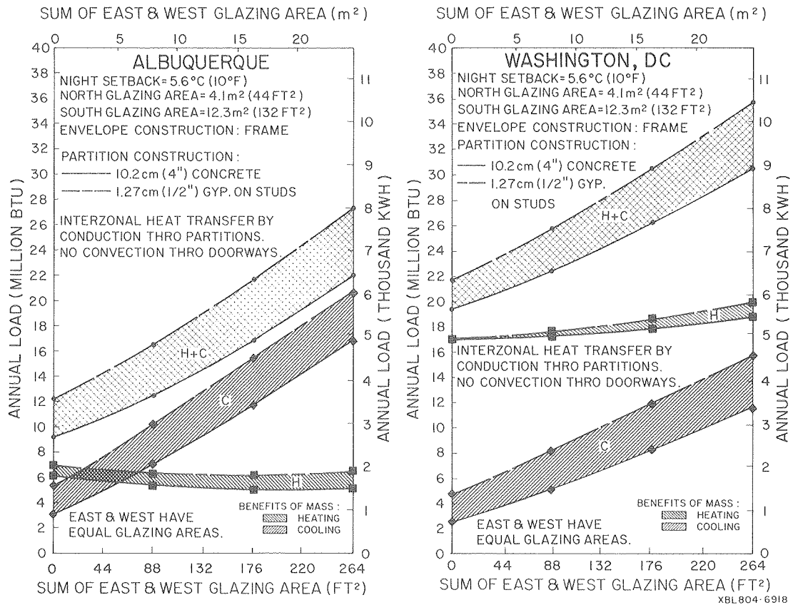
FIG. 6 : Effect of east and west glazing area on building thermal loads.
