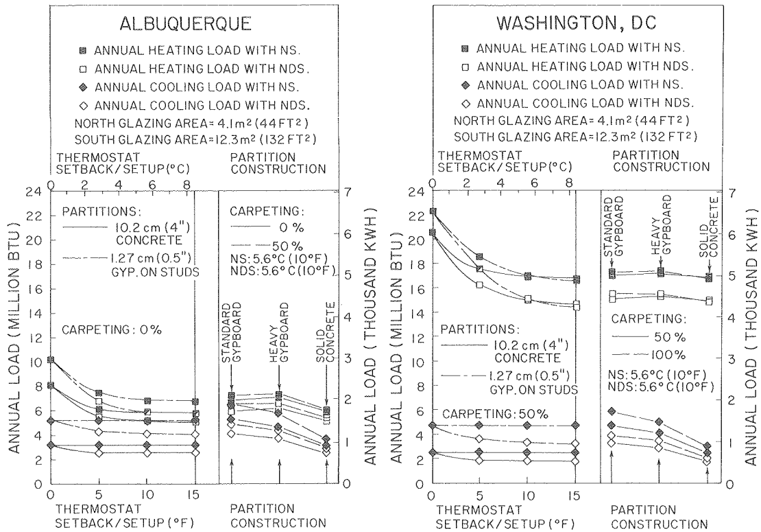
FIG. 7 : Effect of thermostat settings and thermal mass on annual heating & cooling loads.
