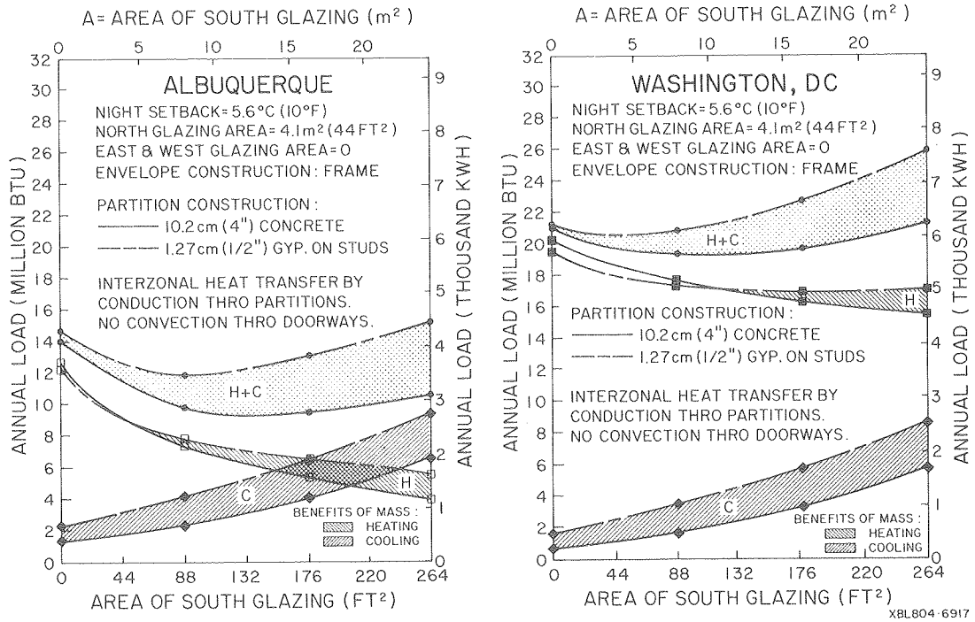
FIG. 5 : Effect of south glazing area on building thermal loads.
