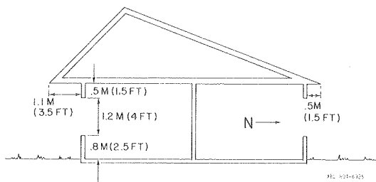
FIG. 3: Cross section for blast simulation.
