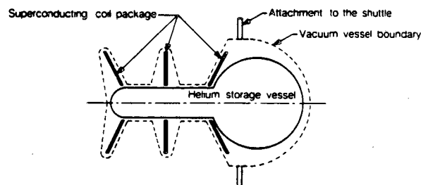
b) Three disc type magnet
