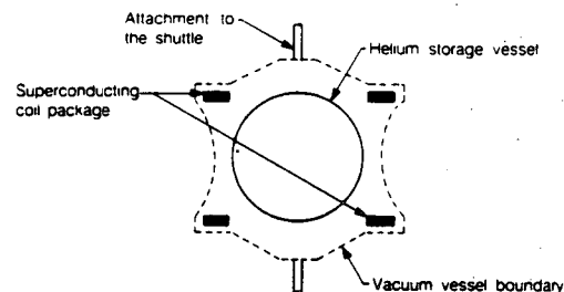
a) HEAO type magnet
