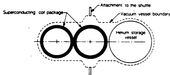
c) Two coil toroid type magnet
